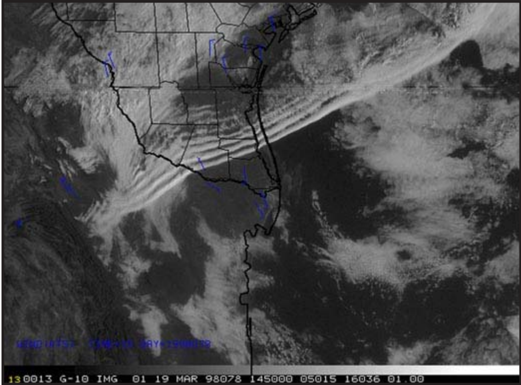
Figure 2-50a. Satellite Depiction of a Gravity Wave.
