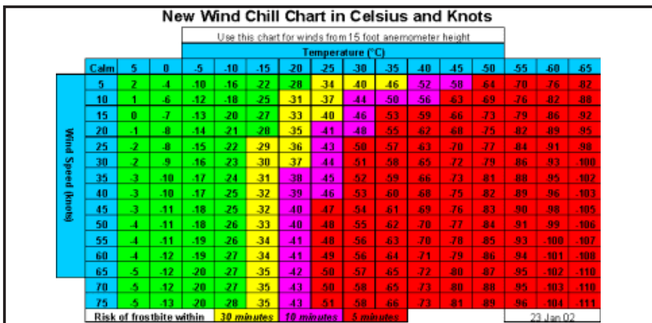
Figure 1-26. Wind Chill Temperature (WCT) Index Chart with 15-Foot Garrison—Anemometer Height (degrees Celsius and knots).
