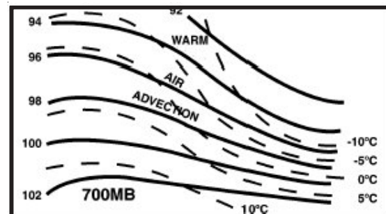
2-76. Decreasing Wind Speed Pattern. Loose thermal packing associated with WAA indicates decreasing wind speeds.
