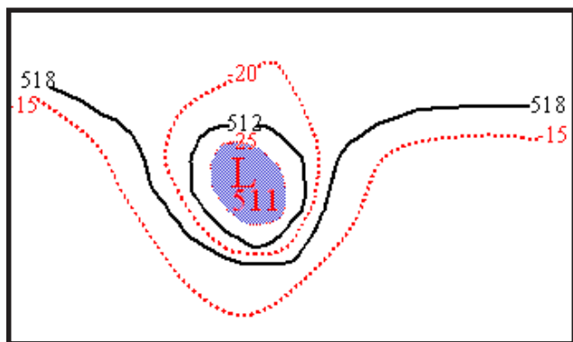
Figure 3-12. Barotropic Low.
