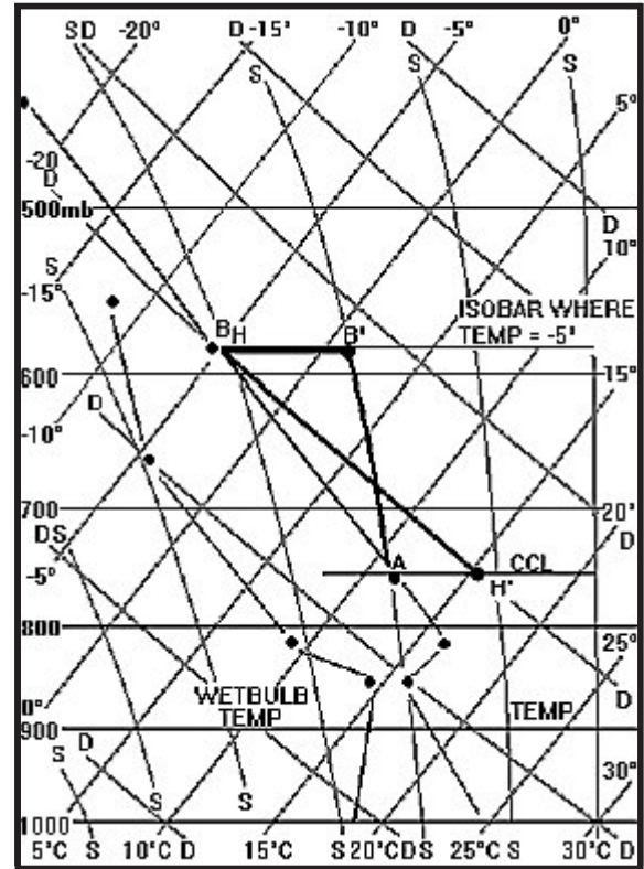
Figure 3-20. Skew-T Chart. Curves labeled “S” are saturation adiabats; lines labeled “D” are dry adiabats. Other points are described in the text.
