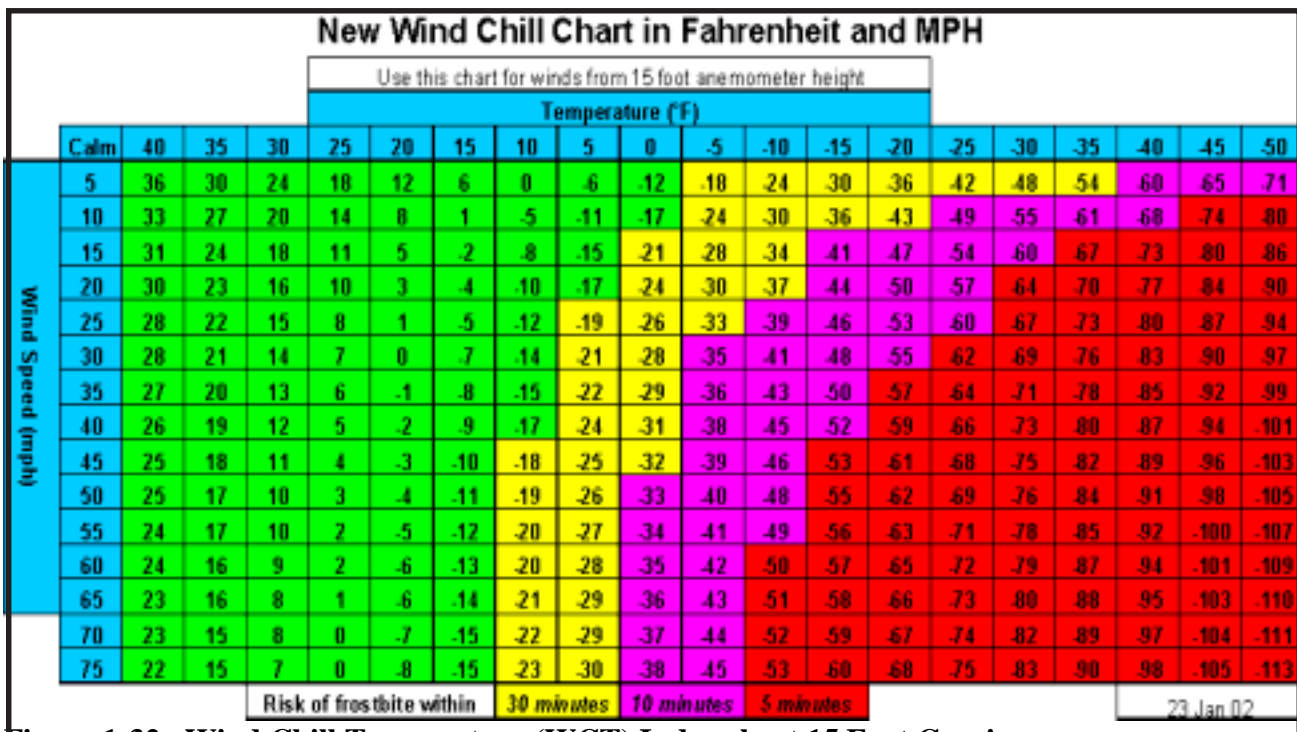
Figure 1-30. Wind Chill Temperature (WCT) Index Chart with 15-Foot Garrison Anemometer Height (degrees Fahrenheit and MPH).
