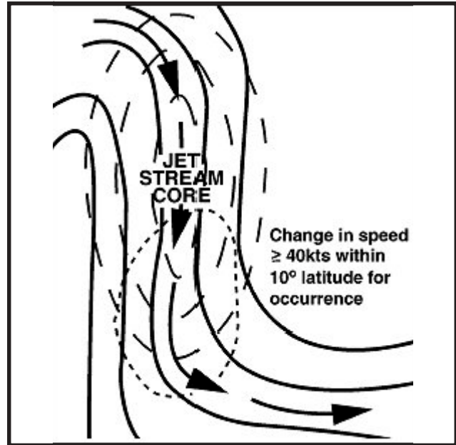
Figure 2-41. CAT Associated with Strong Wind Maximum to the Rear of the Upper Trough. The potential is high when a strong north-south jet is located along the backside of an upper trough.
