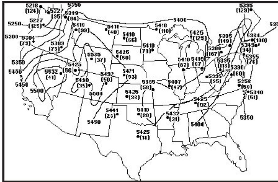
Figure 1-10. Equal Probability of Liquid or Frozen Precipitation. Based upon 1000- to 500-mb thickness (climatology).
