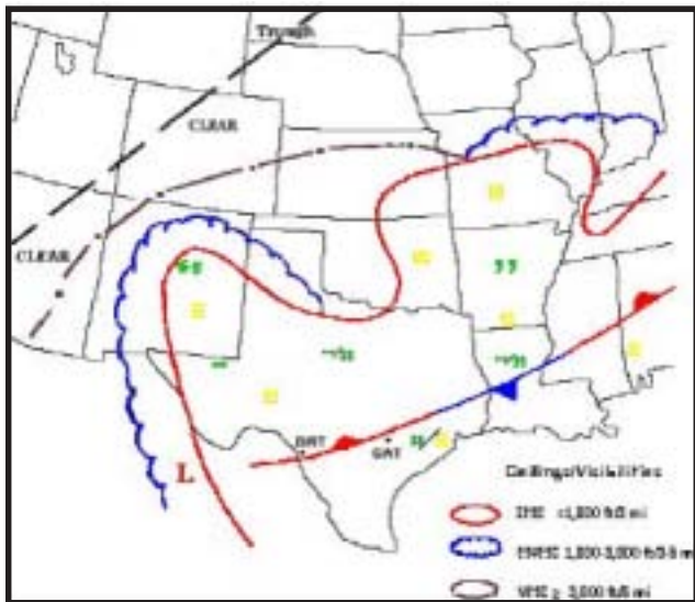
Figure 2-18. Nephanalysis Example.
