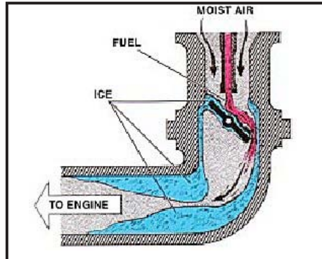
Figure 2-67. Carburetor Icing.
