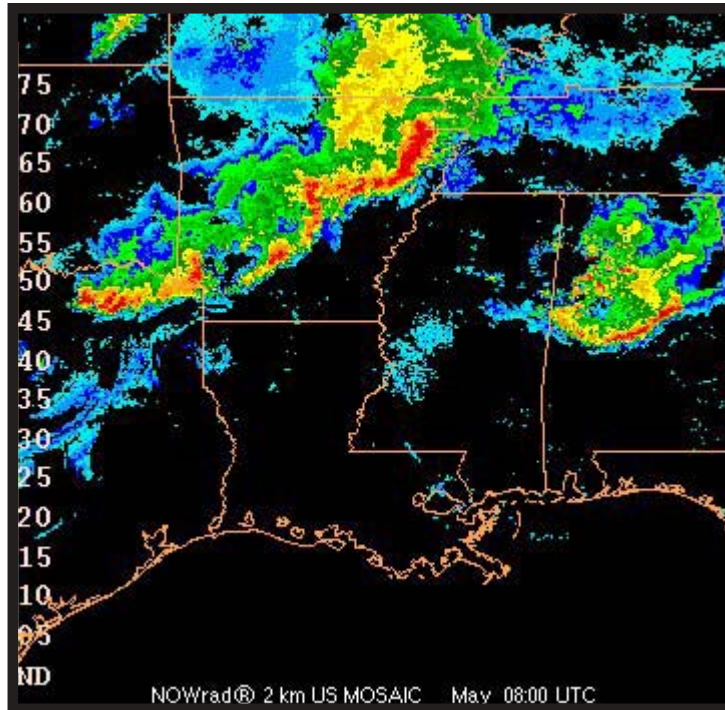
Figure 3-16b. Bow Echo Reflectivity Example.
