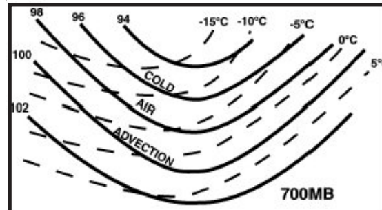
2-75. Increasing Wind Speed Pattern. Tight thermal packing associated with CAA indicates increasing wind speeds.
