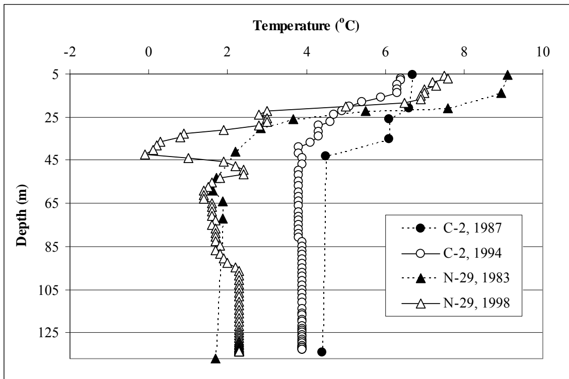
Figure 4.--Outer shelf ( 100 \text{ m} < \text{bottom depth} \leq 200 \text{ m} ) temperature profiles from the southern and northern portions of the survey area from the 1982-1990 and the 1990-2006 data. See Figure 1 for station locations (stars). Statistics associated with these profiles are presented in Table 4.
