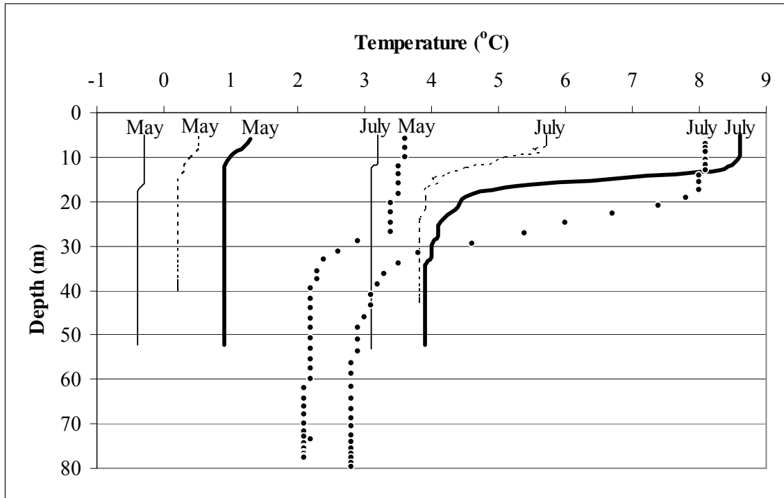
Figure 11.--Comparison of depth-temperature profiles at select stations taken during (May) and after (July) the EBS standard bottom trawl survey in 1999. The locations of stations I-13 (thin, solid line), I-9 (thin dashes), E-12 (thick, solid line), and C-8 (dots) are shown in Figure 1 and are individually identified by their row (letter) and column (number) coordinates on the survey grid.
