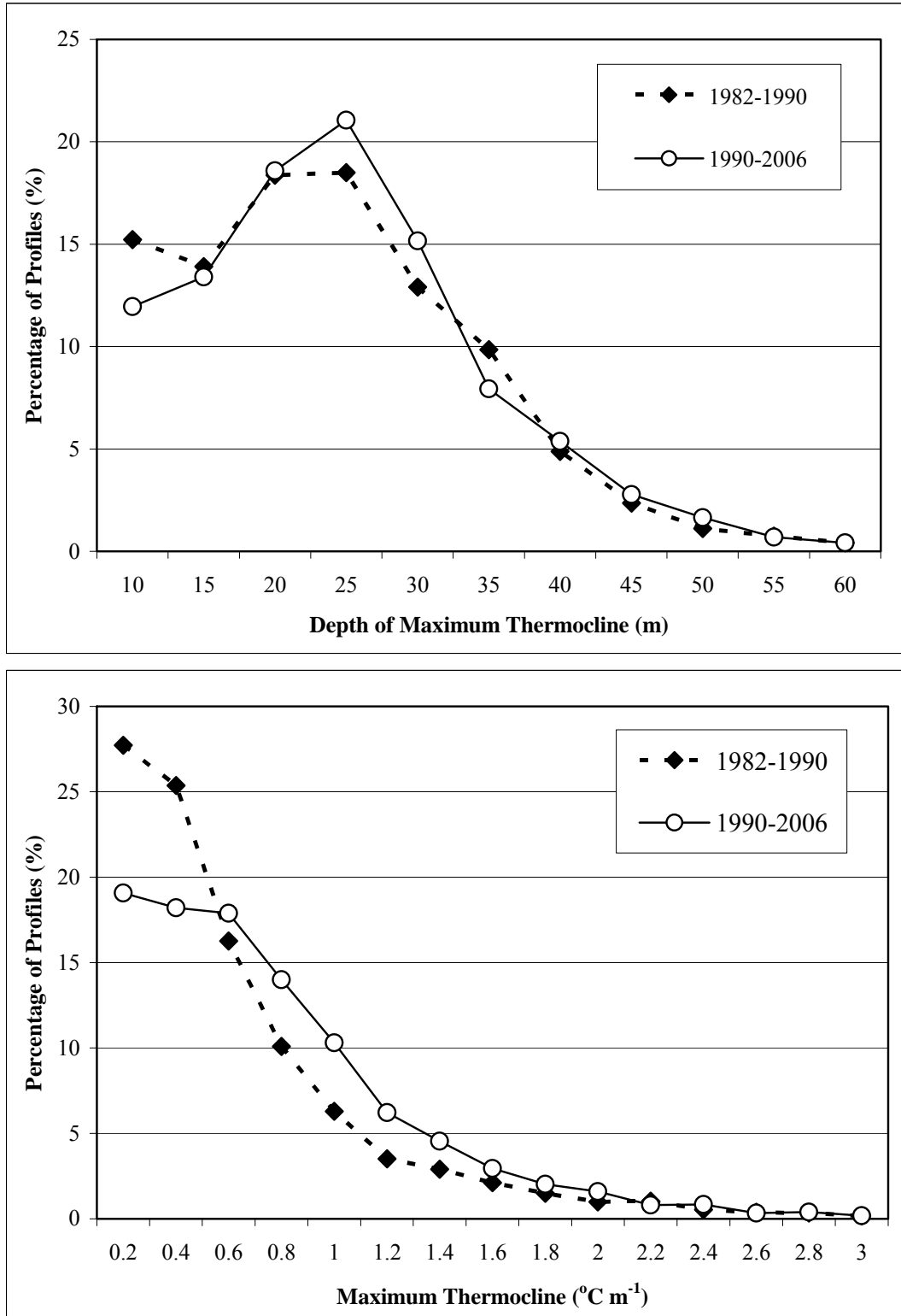
Figure 5.--Comparison of the frequency of the depth of the maximum thermocline (upper panel) and the strength of the maximum thermocline (lower panel) between 1982-1990 and 1990-2006 data.
