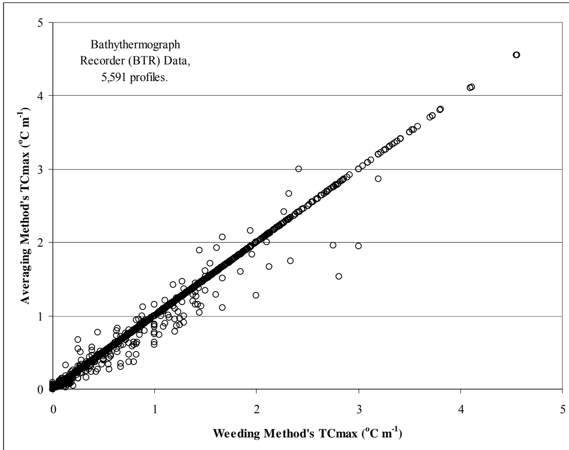
Figure 7.--Comparison of the maximum thermocline values ( \text{TC}_{\text{max}} ) calculated from 1990-2006 data that was thinned by averaging or by weeding in each 1 m depth bin. See Methods for a description of the data-thinning methods.
