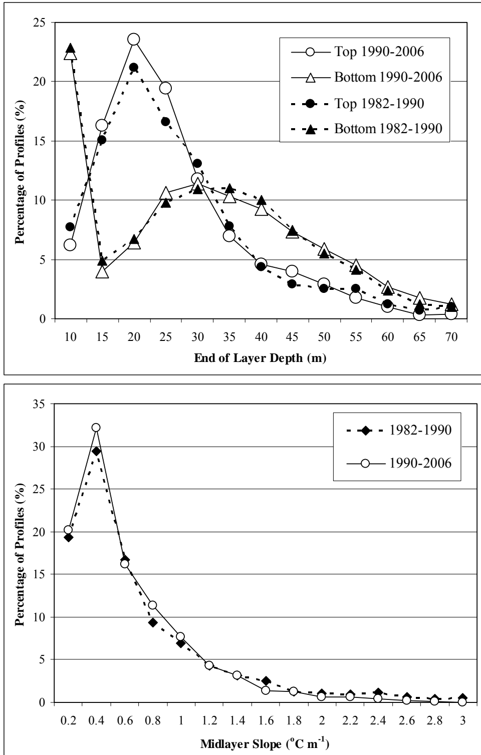
Figure 6.--Comparison of the frequency of the thickness of top layers and the thickness of bottom layers from 1982-1990 and 1990-2006 data (upper panel). And comparison of the frequency of the midlayer slope ( ^{\circ}\text{C m}^{-1} ) from 1982-1990 and 1990-2006 data (lower panel).
