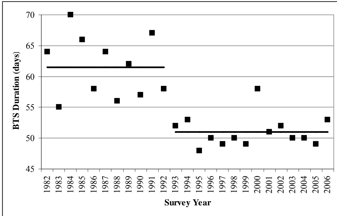
Figure 10.--Duration (End Day minus Start Day) of the AFSC bottom trawl survey (BTS) from 1982 through 2006.
