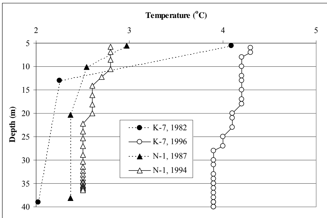
Figure 2.--Inner shelf (bottom depth \leq 50 m) depth-temperature profiles from the southern and northern portion of the survey area from the 1982-1990 and the 1990-2006 data. See Figure 1 for station locations (stars). Statistics associated with these profiles are presented in Table 4.
