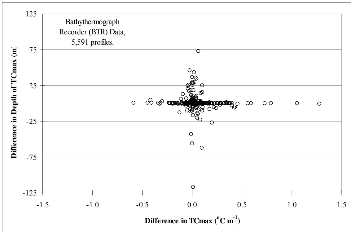
Figure 8.--Comparison of the difference in maximum thermocline values ( \text{TC}_{\text{max}} ) calculated from averaged and weeded data with the difference in the depth associated with the \text{TC}_{\text{max}} from each method of data thinning.
