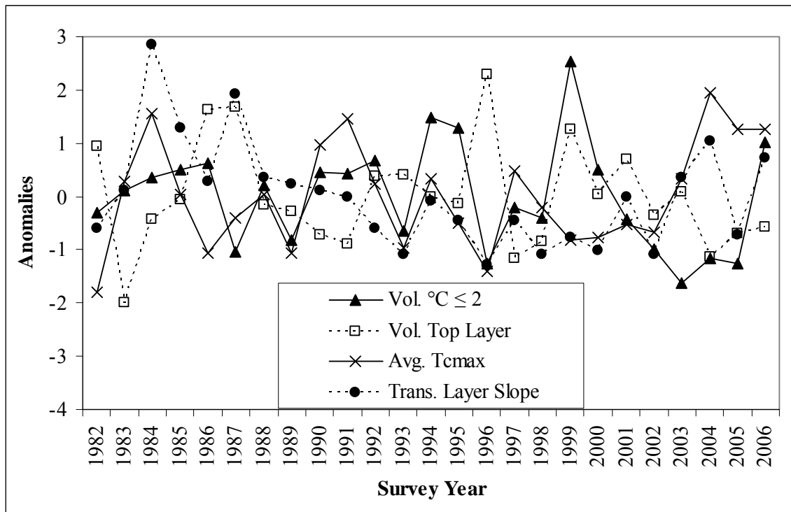
Figure 9.--Time series of some indices for the eastern Bering Sea presented as anomalies. The cold pool is represented by the volume of water with temperatures \leq 2^{\circ}\text{C} . Surface mixing is represented by the volume of the Top Layer. Stratification is represented by both the average of the \text{TC}_{\text{max}} and the average of the Transition Layer slope.
