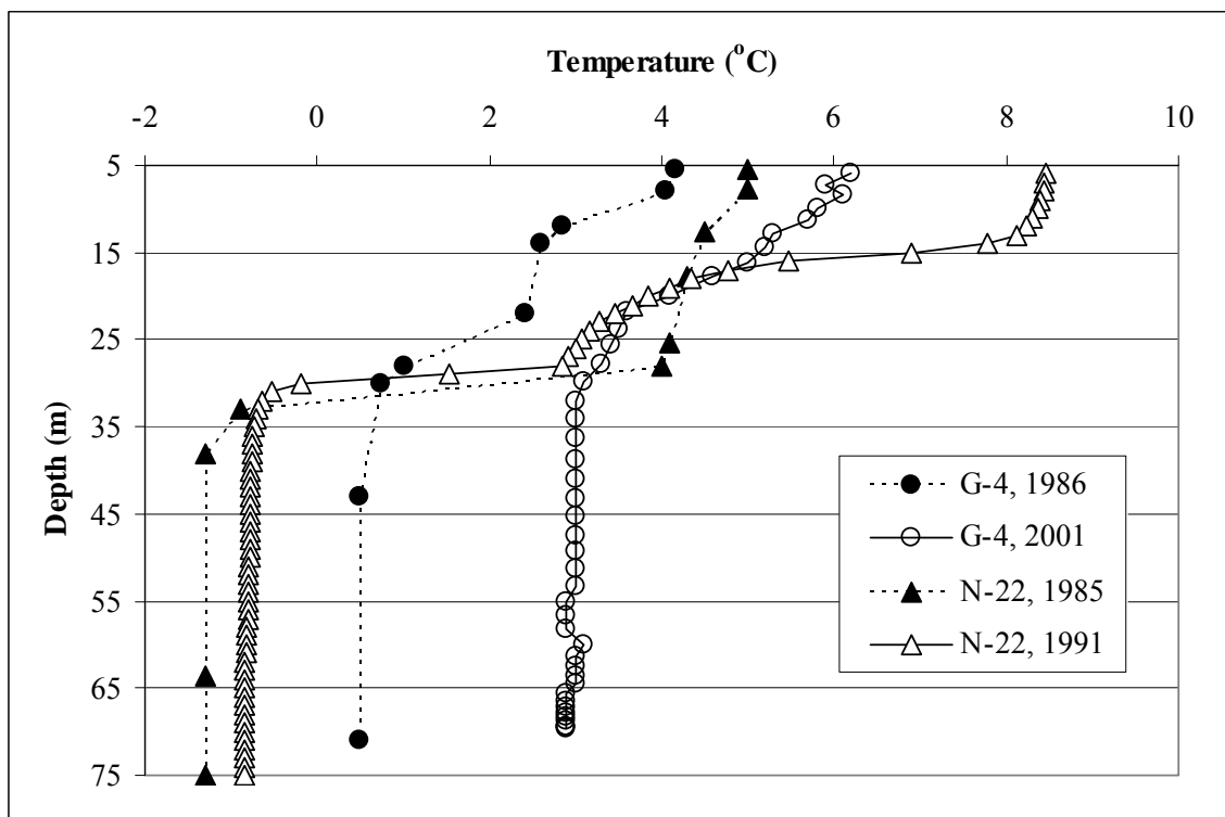
Figure 3.--Middle shelf ( 50 \text{ m} < \text{bottom depth} \leq 100 \text{ m} ) temperature profiles from the southern and northern portions of the survey area from the 1982-1990 and the 1990-2006 data. See Figure 1 for station locations (stars). Statistics associated with these profiles are presented in Table 4.
