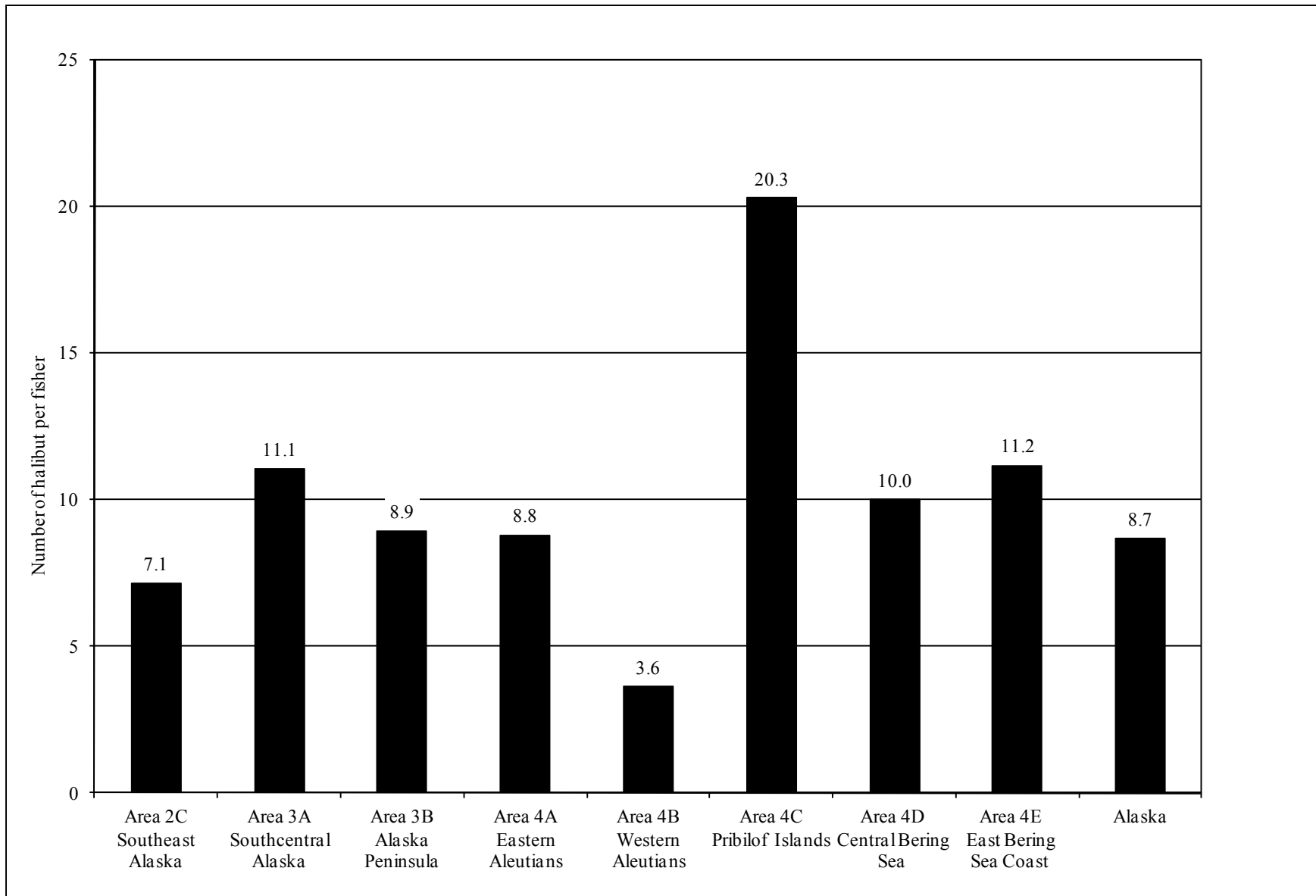
Figure 21.—Average subsistence harvest of halibut per fisher in Alaska, 2010, by regulatory area, in number of fish.
