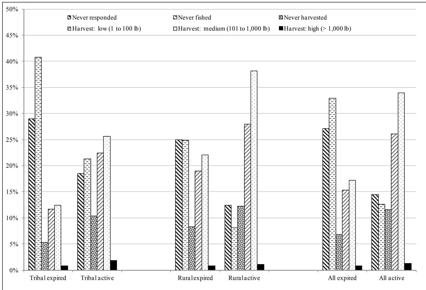
Figure 36.—Percentage of SHARCs that were not renewed by survey response type and SHARC type, through 2009.
