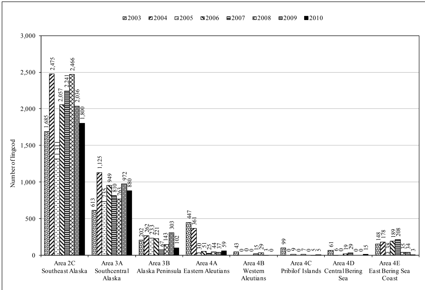
Figure 30.—Estimated incidental harvests of lingcod in the Alaska subsistence halibut fishery, number of fish, by regulatory area fished, 2003–2010.
