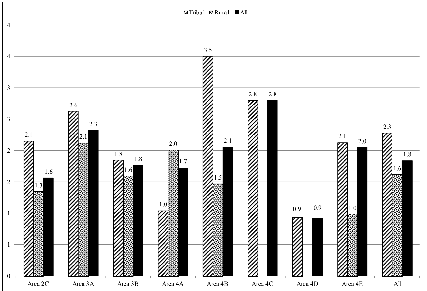
Figure 27.—Average number of halibut harvested per subsistence fishing trip by regulatory area and SHARC type, 2010.
