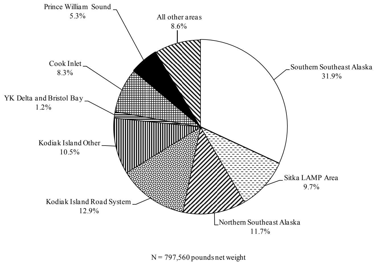
Figure 16.—Percentage of Alaska subsistence halibut harvest by geographic area, 2010.
