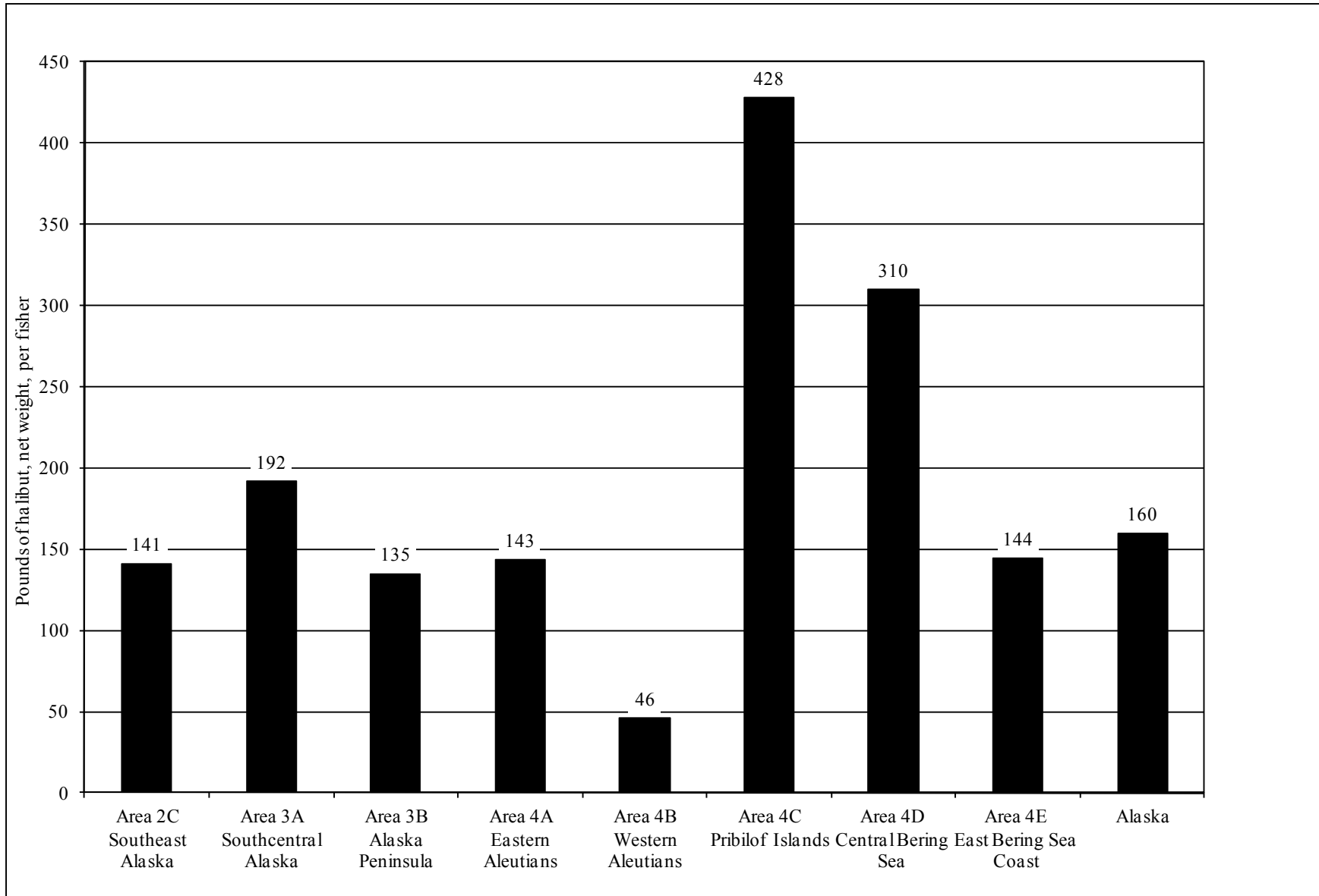
Figure 20.—Average subsistence harvest of halibut per fisher in Alaska, 2010, by regulatory area, in pounds net weight.
