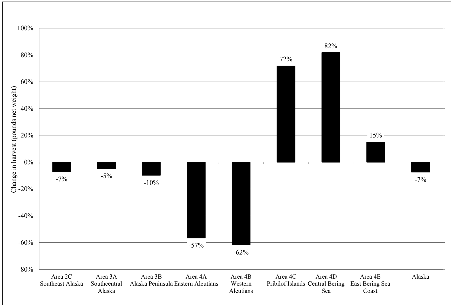
Figure 18.—Change in Alaska subsistence halibut harvests from 2009 through 2010 by regulatory area fished.
