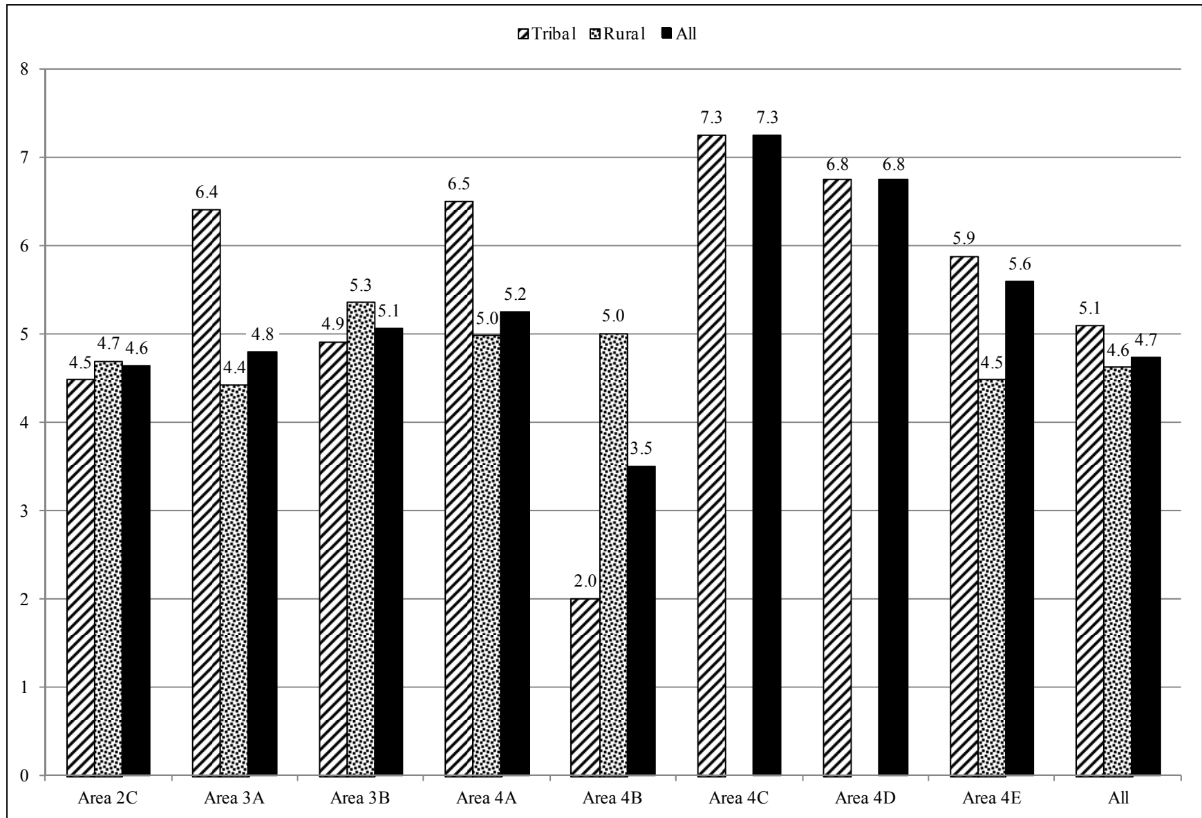
Figure 25.—Average number of subsistence fishing trips for halibut by regulatory area and SHARC type, 2010.
