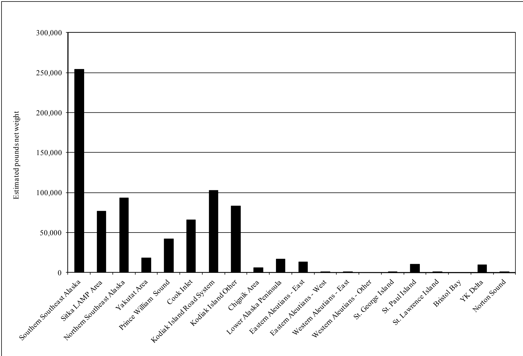
Figure 15.—Alaska subsistence halibut harvests by geographic area, 2010.
