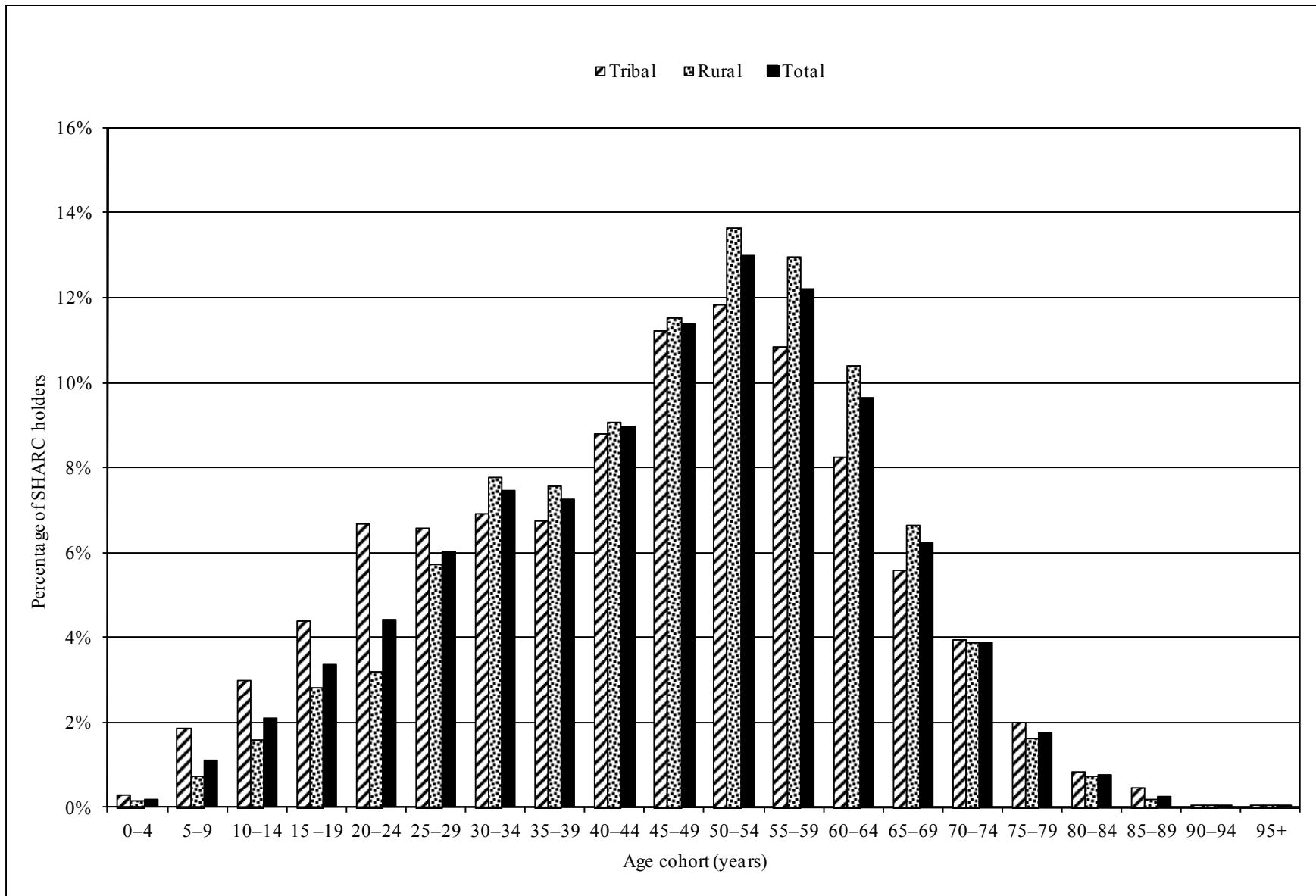
Figure 7.—Age of subsistence halibut registration certificate holders by SHARC type, 2010.
