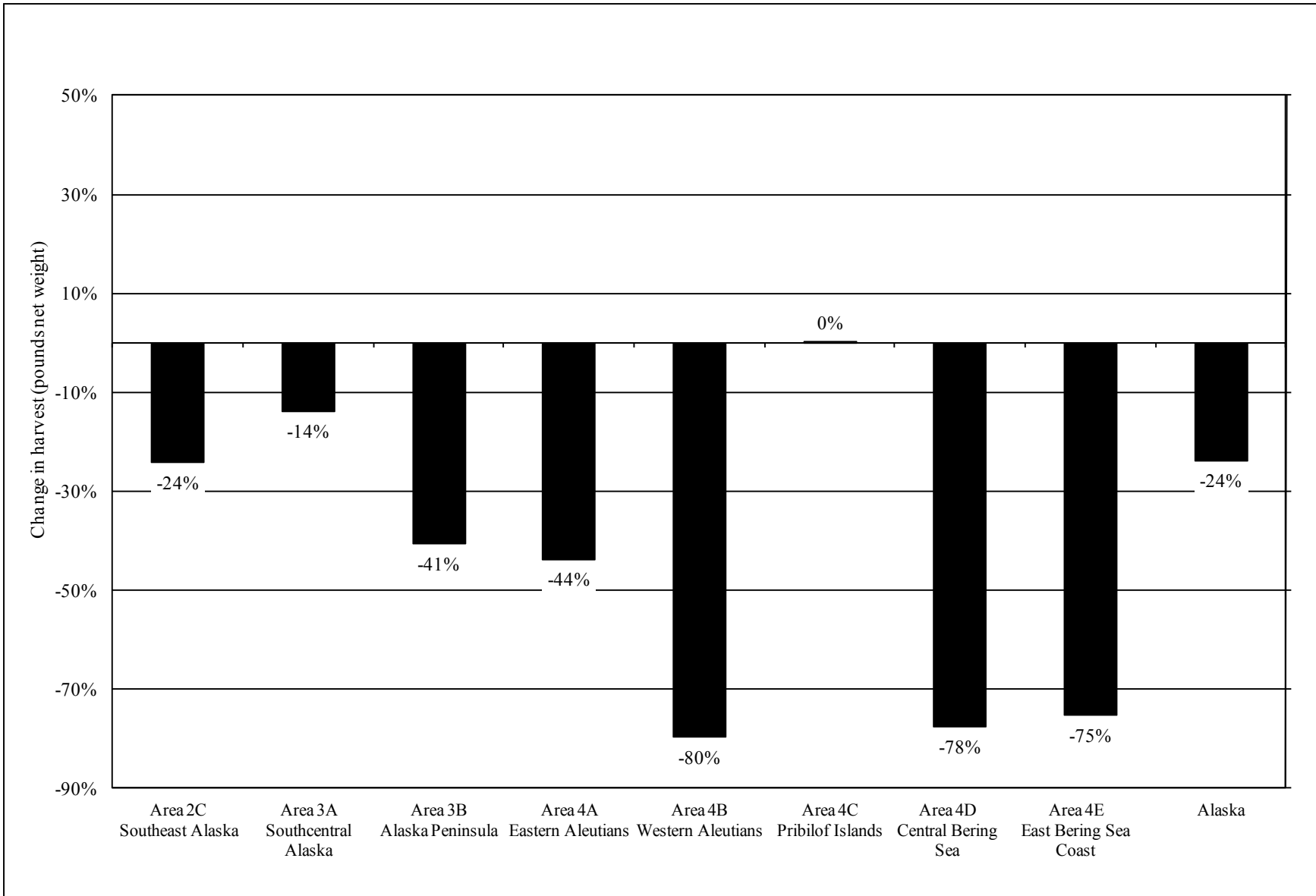
Figure 19.—Change in Alaska subsistence halibut harvests in 2010 compared to recent 7-year average (2003–2009) by regulatory area fished.
