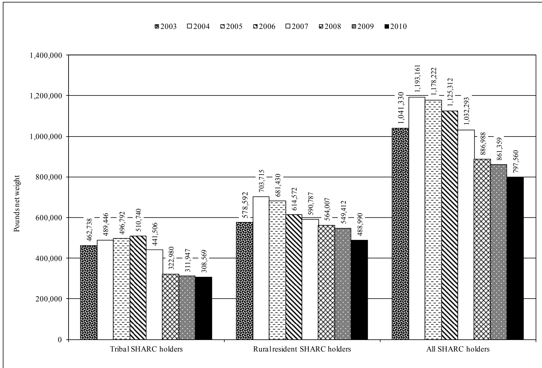
Figure 11.—Estimated Alaska subsistence halibut harvests in pounds net weight by SHARC type, 2003–2010.
