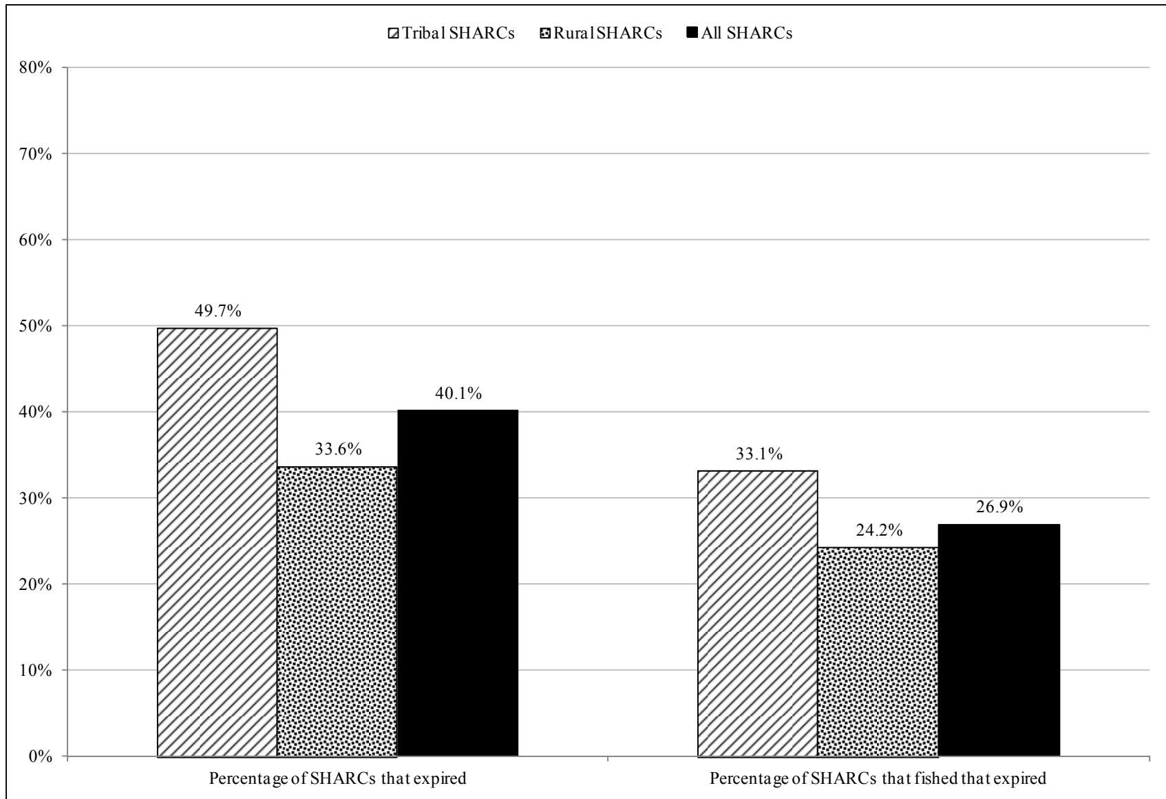
Figure 35.—Percentage of SHARC holders, and SHARC holders who fished for halibut, who did not renew their SHARC, by SHARC type, through 2009.
