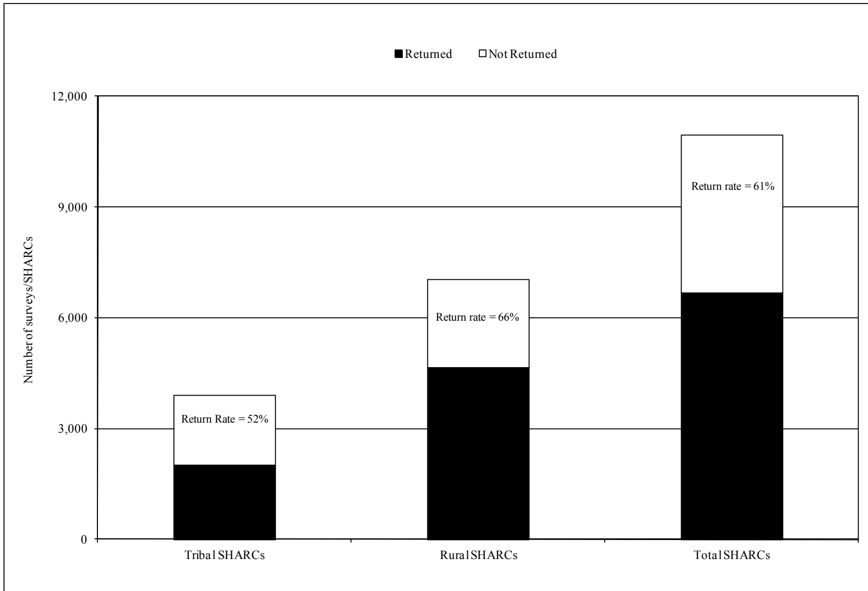
Figure 2.—Number of surveys returned and return rates for subsistence halibut surveys, by SHARC type, 2010.
