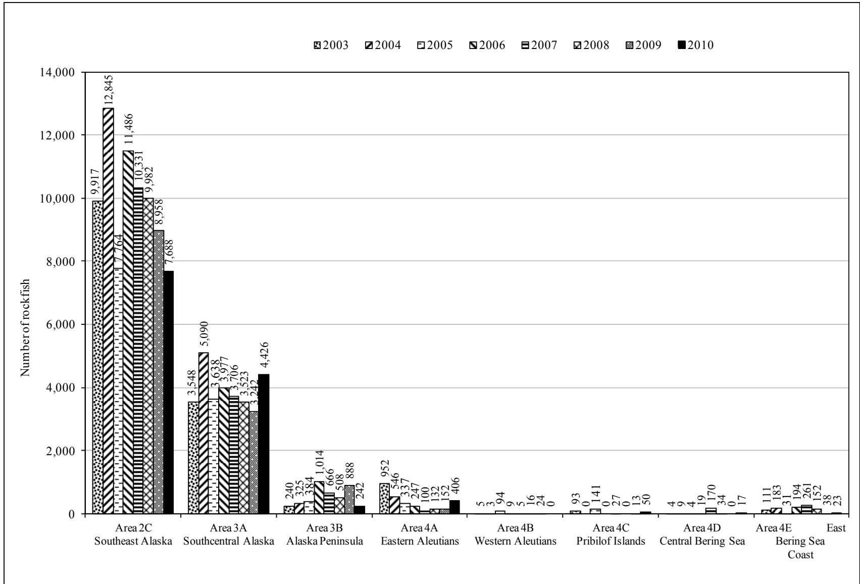
Figure 28.—Estimated incidental harvests of rockfish in the Alaska subsistence halibut fishery, number of fish, by regulatory area fished, 2003–2010.
