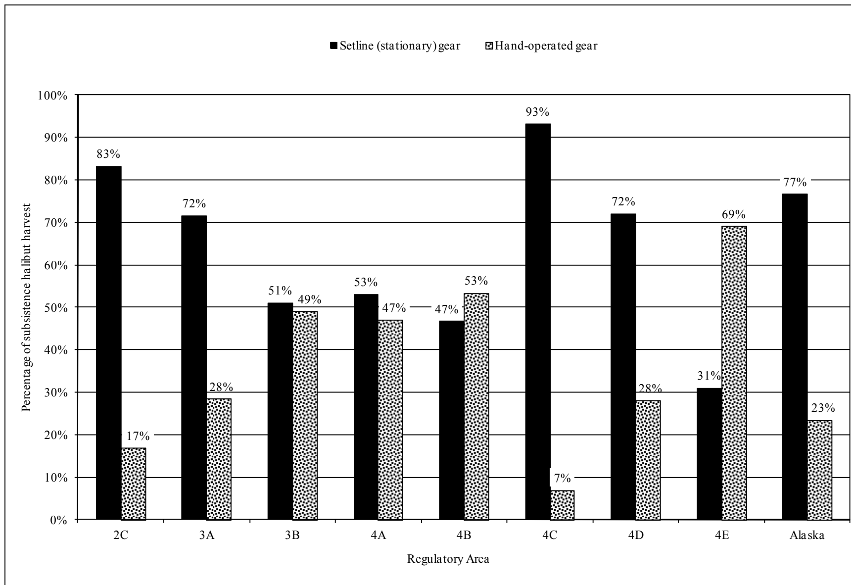
Figure 23.—Percentage of subsistence halibut harvest by gear type by regulatory area, 2010.
