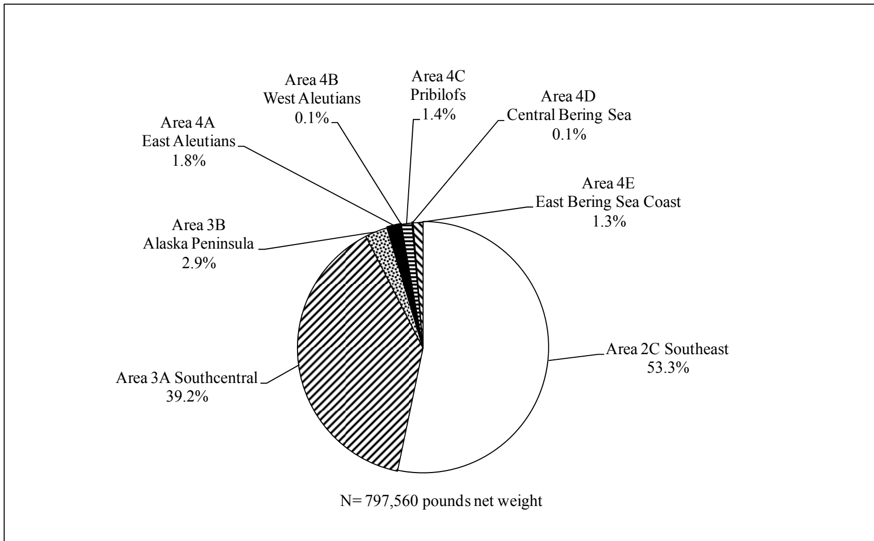
Figure 14.—Percentage of subsistence halibut harvest by regulatory area fished, 2010.
