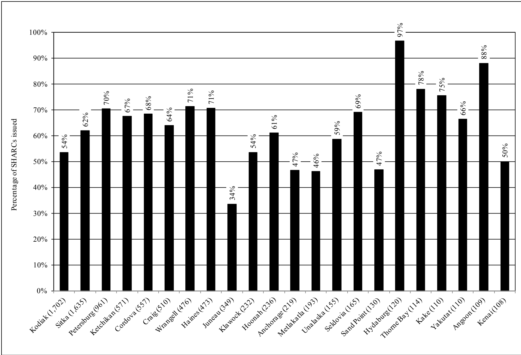
Figure 4.—Return rate by place of residence, 2010.
