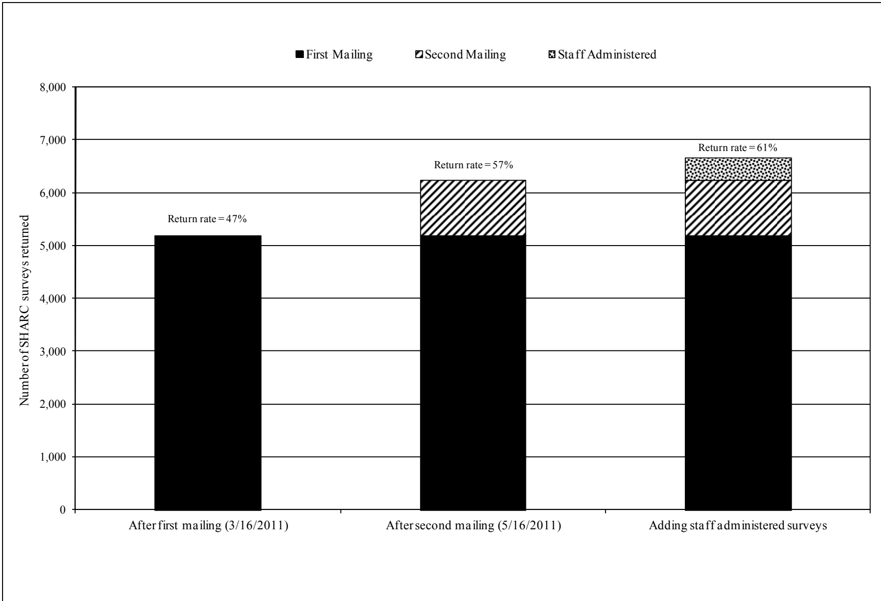
Figure 5.—Number of survey responses by response category, 2010.
