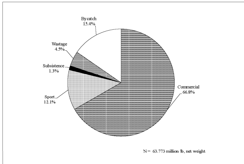
Figure 33.—Halibut removals, Alaska, 2010.
