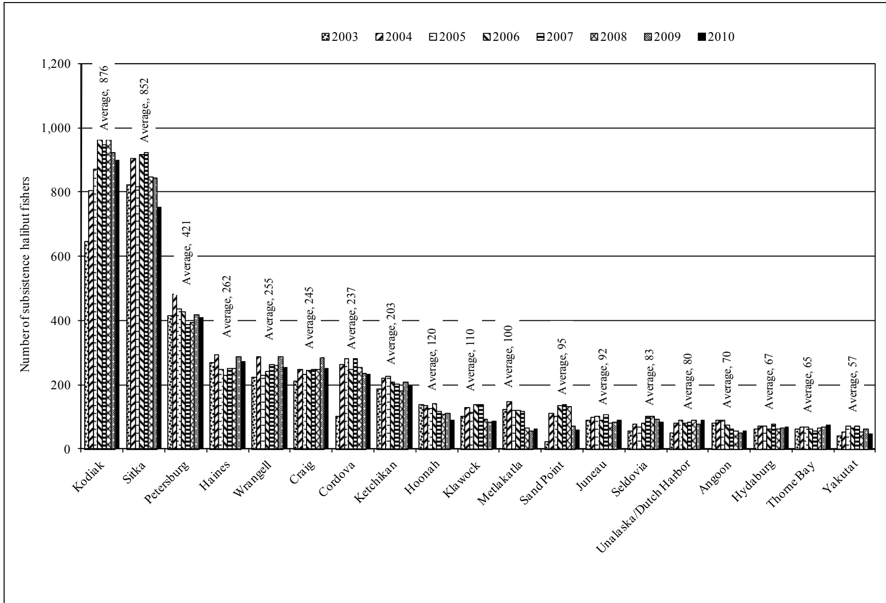
Figure 9.—Estimated number of subsistence halibut fishers by place of residence, 2003–2010, communities with 50 or more fishers in 2010.
