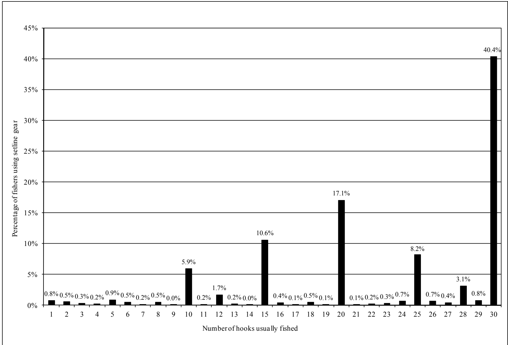
Figure 24.—Number of hooks usually fished, percentage of fishers using setline (stationary) gear, Alaska subsistence halibut fishery, 2010.
