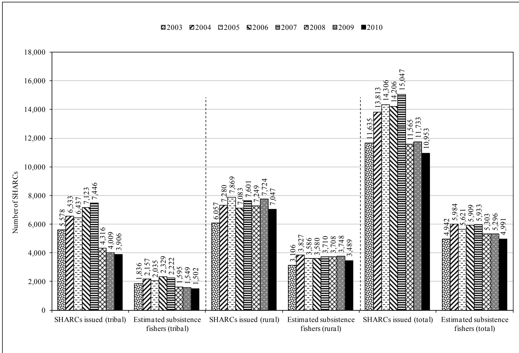
Figure 6.—Number of SHARCs issued and estimated number of subsistence halibut fishers by SHARC type, 2003–2010.
