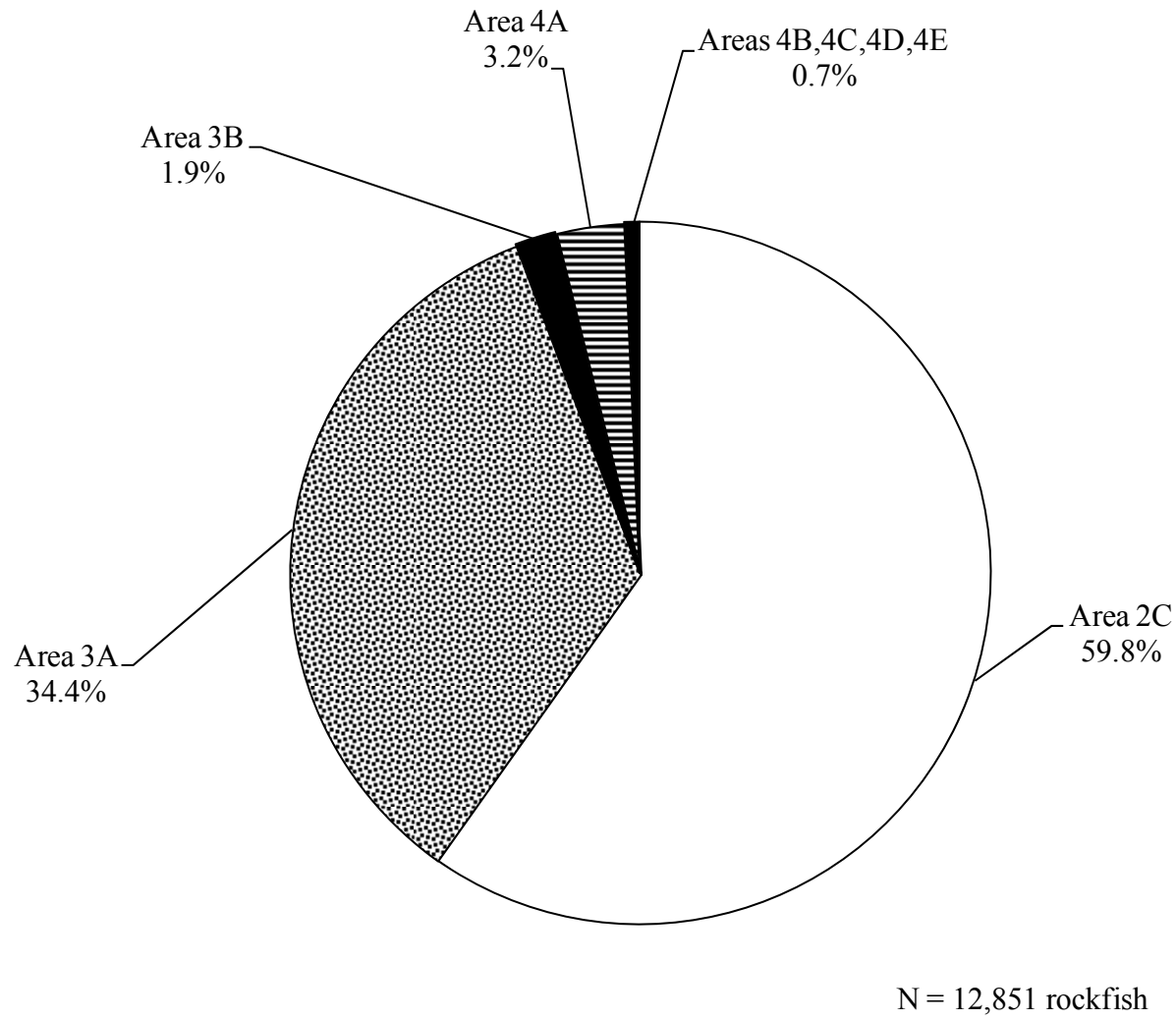
Figure 29.—Percentage of incidental harvest of rockfish by regulatory area fished, 2010.
