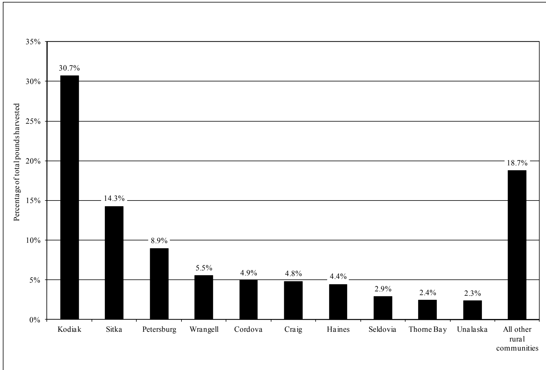
Figure 13.—Percentage of rural community subsistence halibut harvest by community, 2010.
