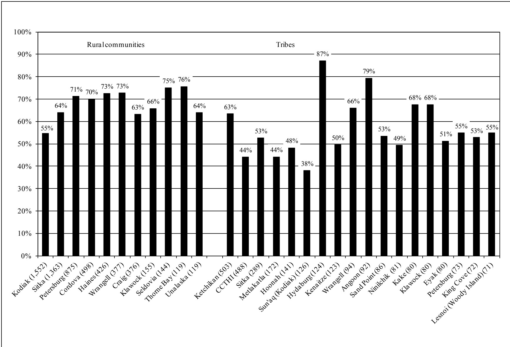
Figure 3.—SHARC survey return rates, communities with more than 100 SHARCs issued and tribes with more than 70 SHARCs issued, 2010.
