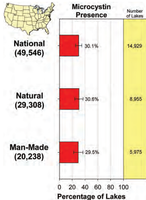
Figure 17. Occurrence of microcystin in lakes.
