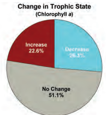
Figure 35. Proportion of NES lakes that exhibited improvement, degradation, or no change in trophic state based on the comparison of the 1972 National Eutrophication Survey and the 2007 National Lakes Assessment.
