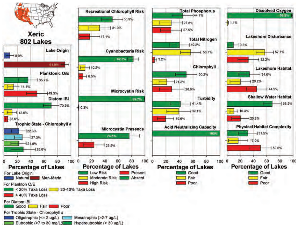
Figure 33. NLA findings for the Xeric. Bars show the percentage of lakes within a condition class for a given indicator. For Recreational Chlorophyll risk and Cyanobacteria risk, the percentage numbers indicate the risk of exposure to algal toxins associated with the presence of chlorophyll-a and cyanobacteria, not the risk of exposure to chlorophyll-a and cyanobacteria per se .
