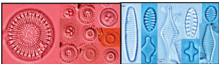
Centrate (left) and pinnate (right) diatoms. Image courtesy of J. Smol as provided by D. Charles.
