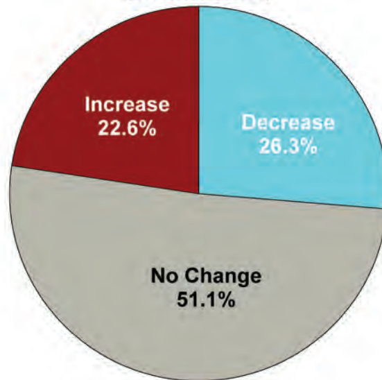
Change in Trophic State (Chlorophyll a )
