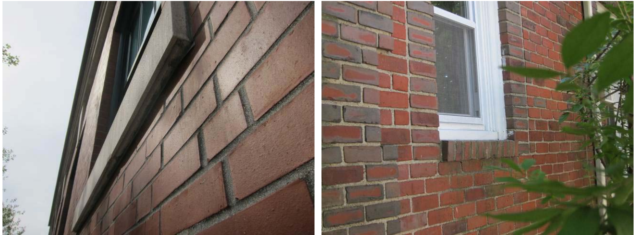
Figure 17. Precast window sill drip edge detail (L); rowlock window sill (R)
