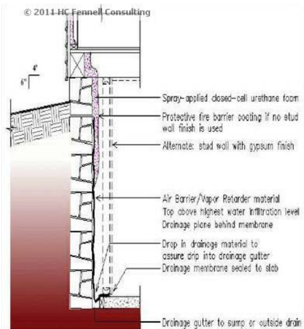
Figure 4. AVID installation and diagram (© 2011 by HC Fennell Consulting; reprinted with permission)
