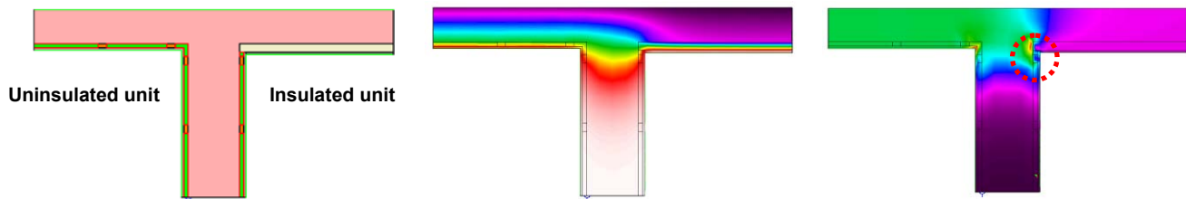
Figure 18. Two-dimensional heat flow modeling party wall (assembly, temperatures, heat flux)
