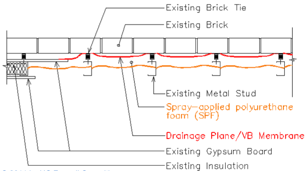
Figure 5. “Inside-out” approach (© 2011 by HC Fennell Consulting; reprinted with permission)
