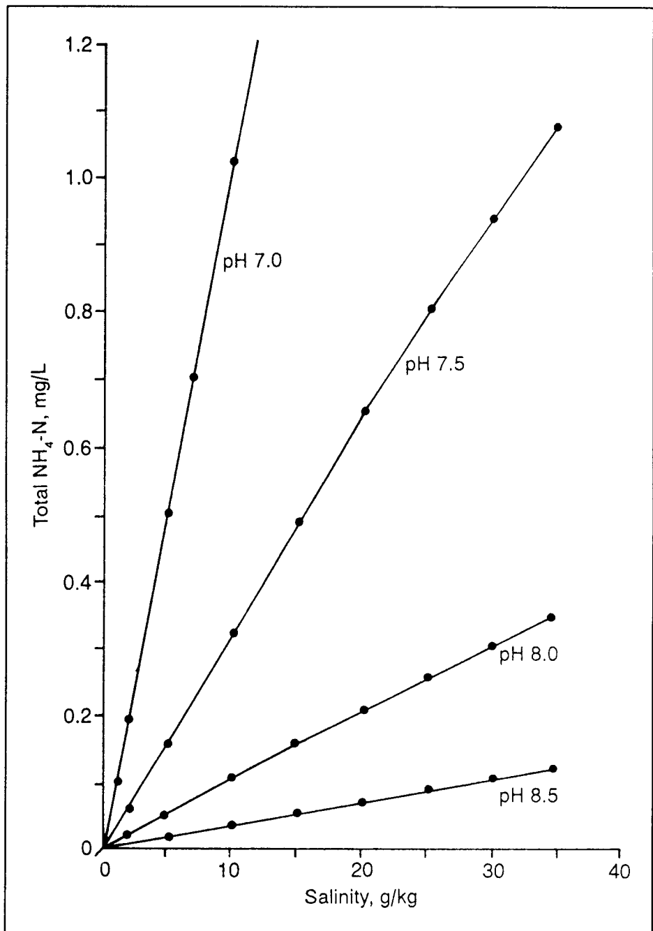
Figure 7.—Plot of total ammonia nitrogen (total NH 4 -N) versus "salinity" in artificial seawater to give an equal probability of forming hypobromous acid (HOBr) or monochloramine (NH 2 Cl) at a stipulated pH. Combinations falling above a pH line produce conditions favorable for NH 2 Cl formation; combinations below a line enhance formation of HOBr. Source: Johnson and Inman (1978).
