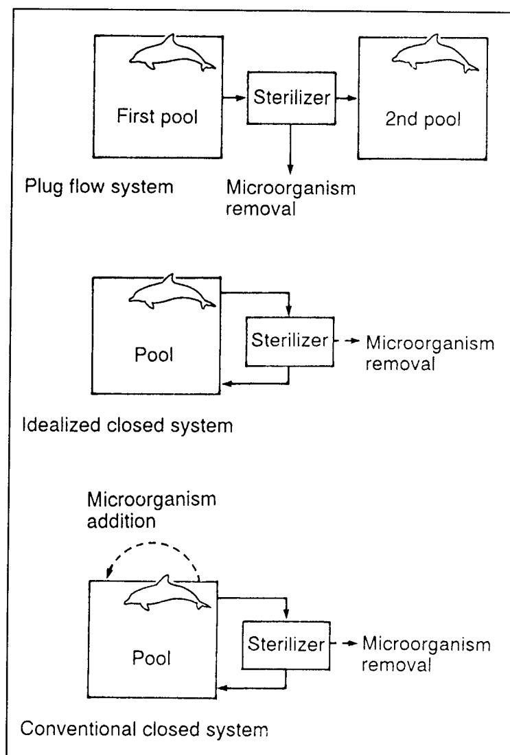
Figure 3.—Plug flow system: water flows through the sterilizer in a single pass, and micro-organisms are removed at a constant rate. Idealized closed system: all water is recycled, there is no new addition of pathogens, and micro-organisms are removed at a rate proportional to their concentration. Conventional closed system: all water is recycled, micro-organisms are added at a constant rate, and removed at a rate proportional to their concentration. Efficacy at all three contact sites is assumed to be 100 percent. Source: Spotte and Adams (1981).
