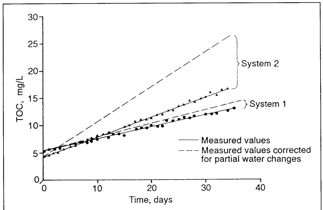
Figure 8.—Accumulation of total organic carbon (TOC) with time in two closed-system marine mammal pools (see text descriptions). Source: Spotte and Adams (1979).
