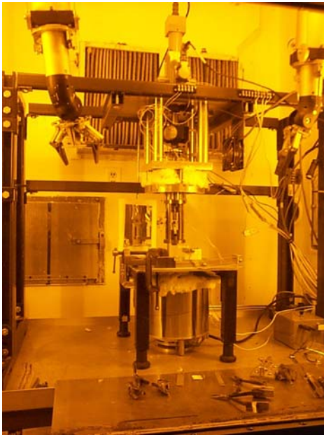
In-Cell Fracture Toughness Tester
