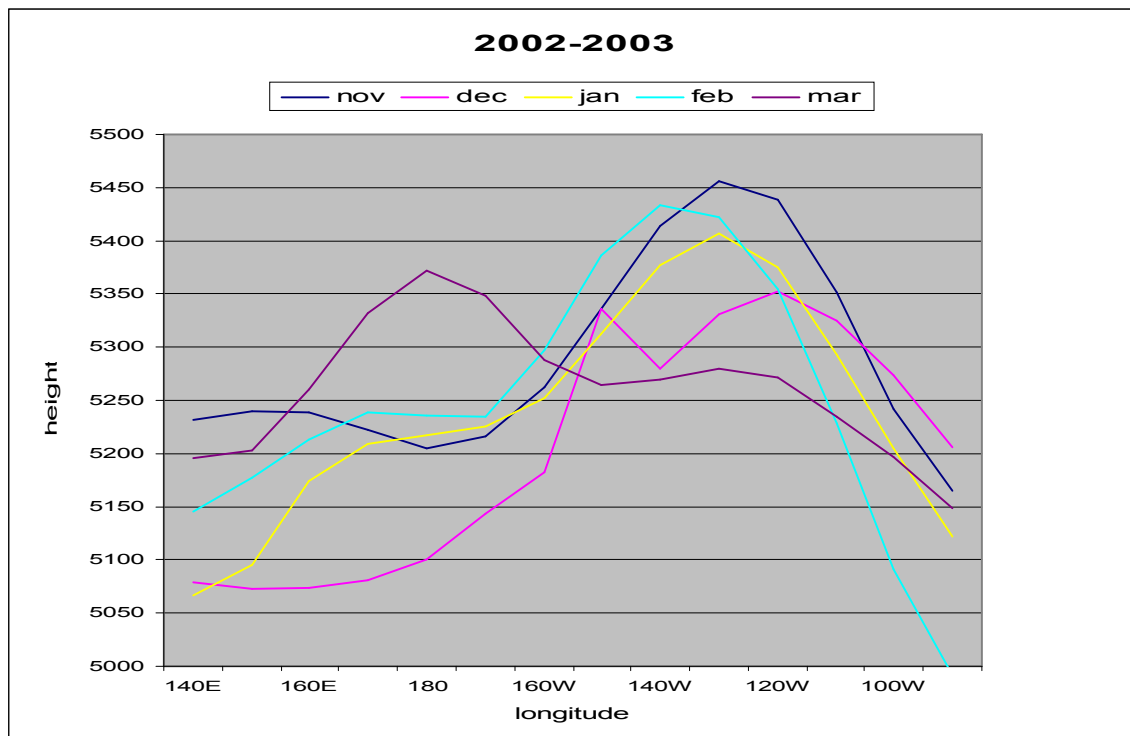
Figure 2: Mean monthly 500mb heights at 60°N for 2002-2003 El Nino.
