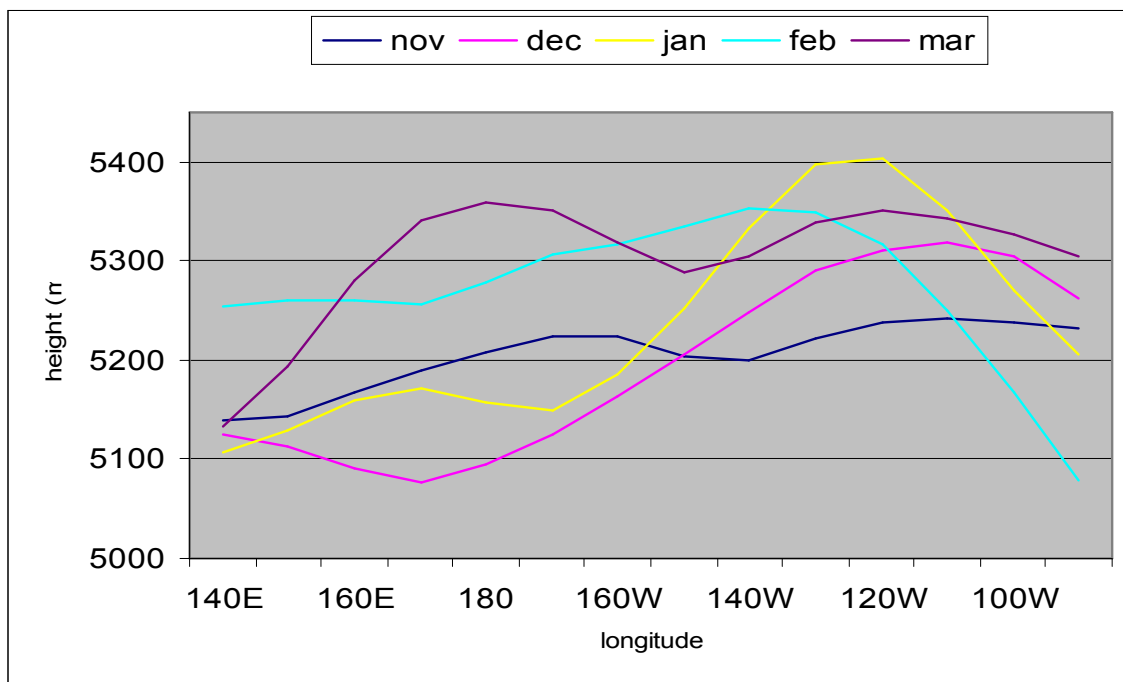
Figure 2: Mean monthly 500 mb heights at 60°N for 1994-1995 El Nino
