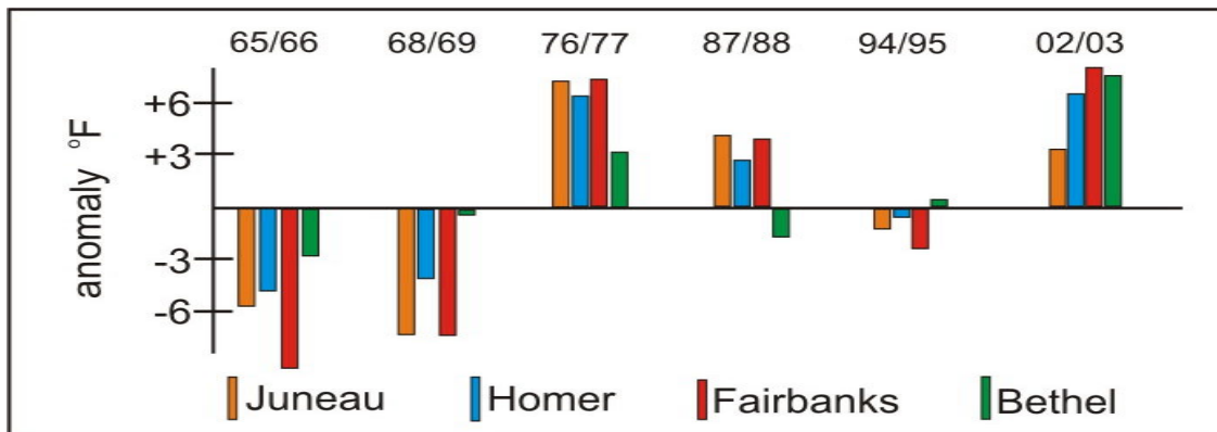
Figure 1: Seasonal temperature anomalies for six El Nino's
