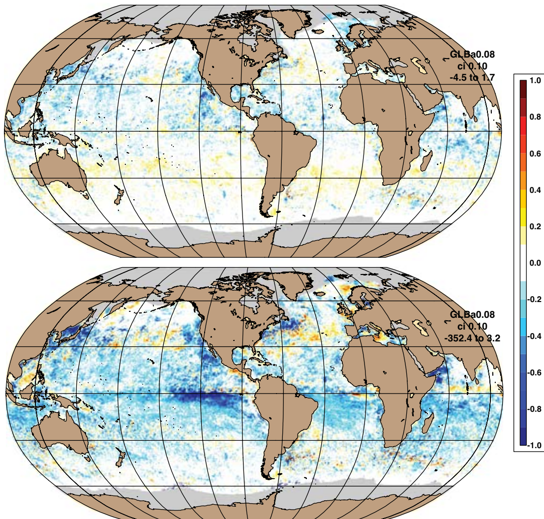
FIGURE 5 Sea surface temperature (SST) mean error (bias) relative to ~33,000,000 multi-channel SST (MCSST) observations at the analysis time (top) and for a 3-day forecast (bottom). Red (blue) colors indicate simulated SST is warmer (cooler) than observed. Values between \pm 0.1 °C are white. The gray area near the poles is an annual average ice coverage mask.
