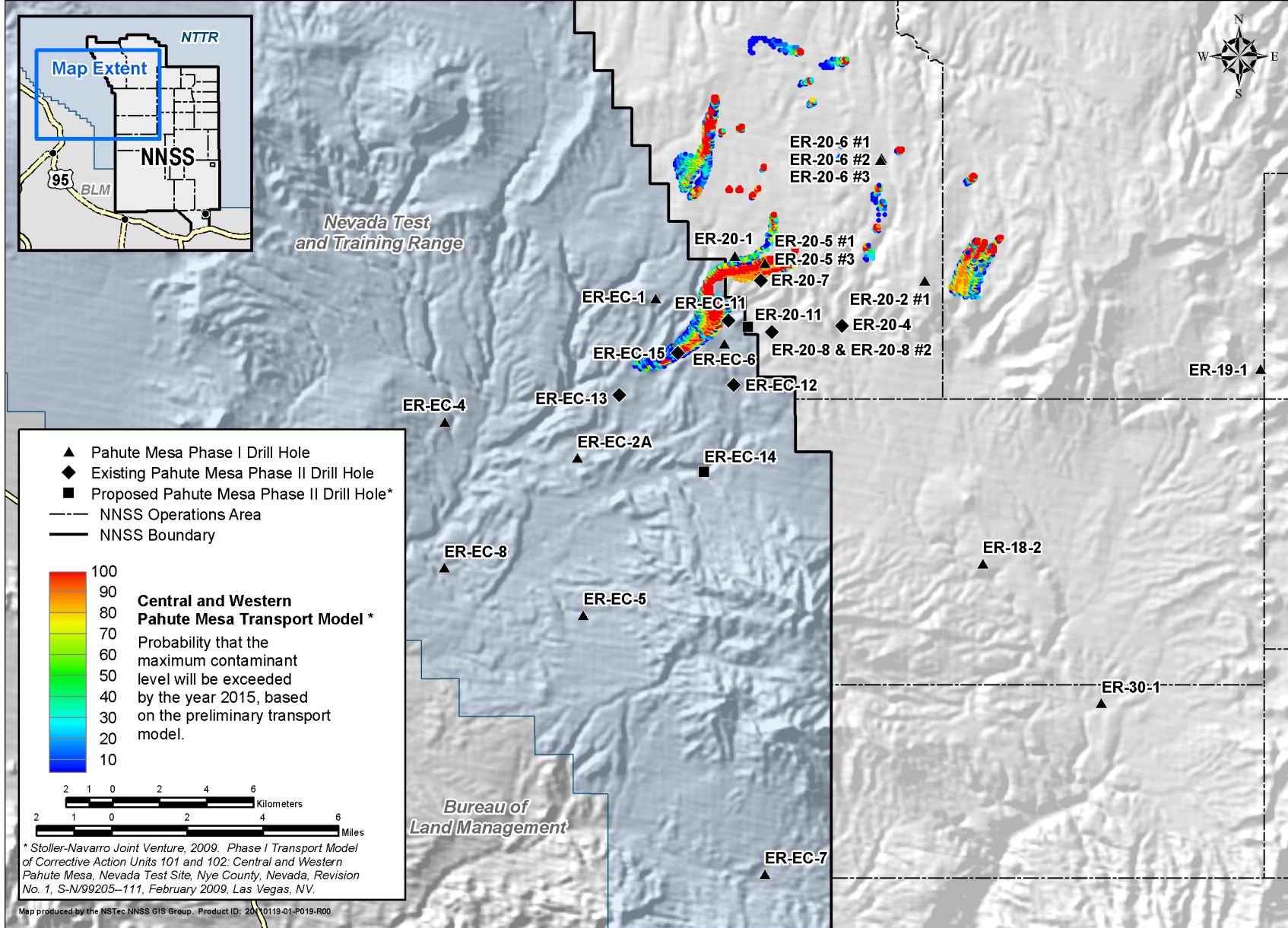
Figure 12-6. Results of Phase I Central and Western Pahute Mesa Transport Modeling
