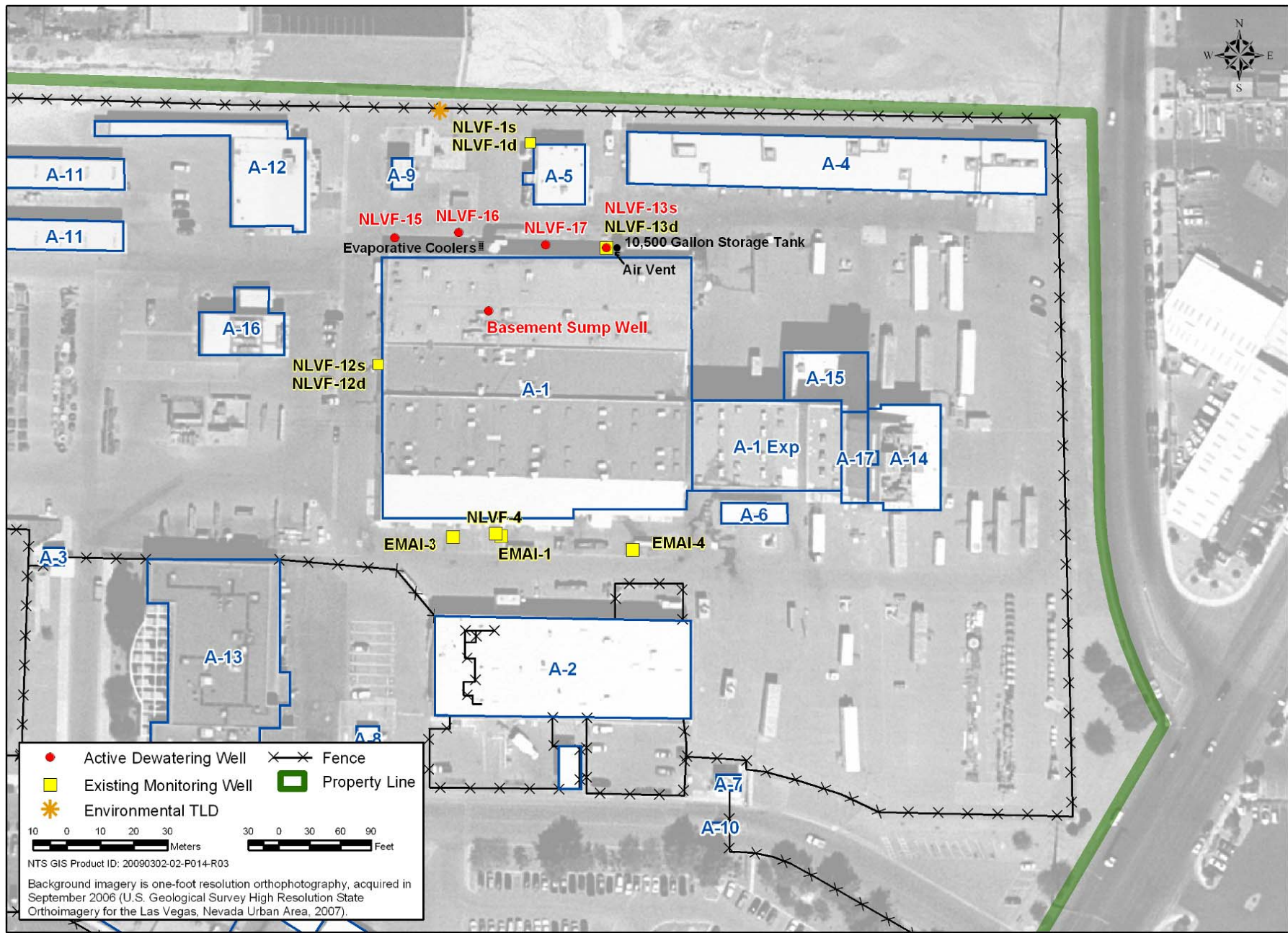
Figure A-2. Location of dewatering and monitoring wells around Building A-1
