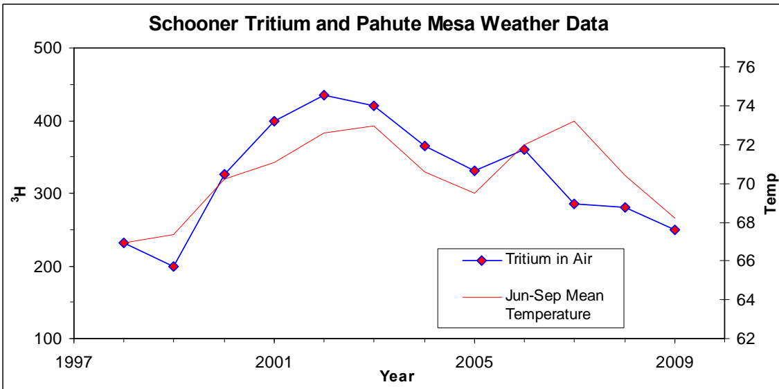
Figure 4-10. Concentrations of ^3\text{H} at Schooner and June–September mean temperatures at Pahute Mesa, 1998–2009
