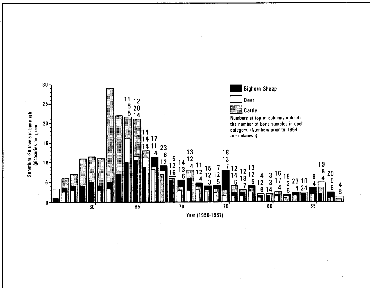
Figure 19. Average ^{90}\text{Sr} Concentrations in Animal Bone.
