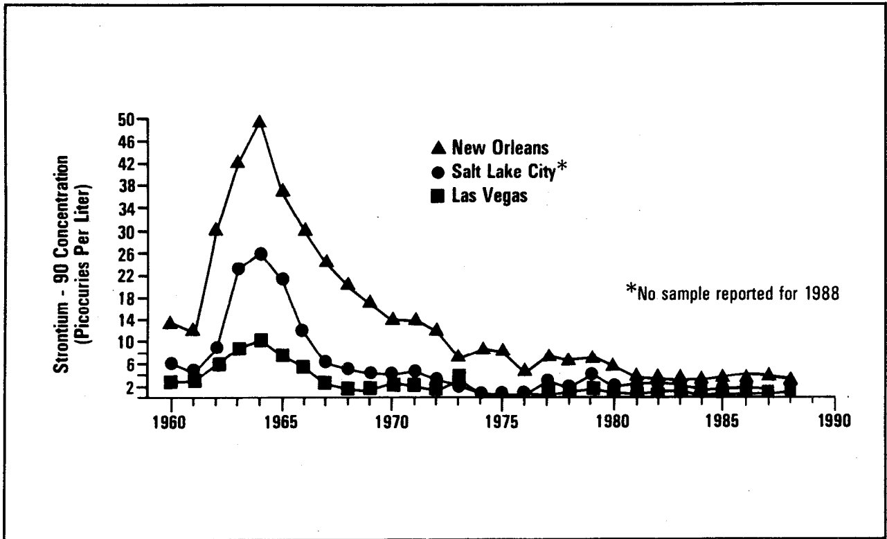
Figure 17. Strontium-90 Concentration in Pasteurized Milk Network Samples.
