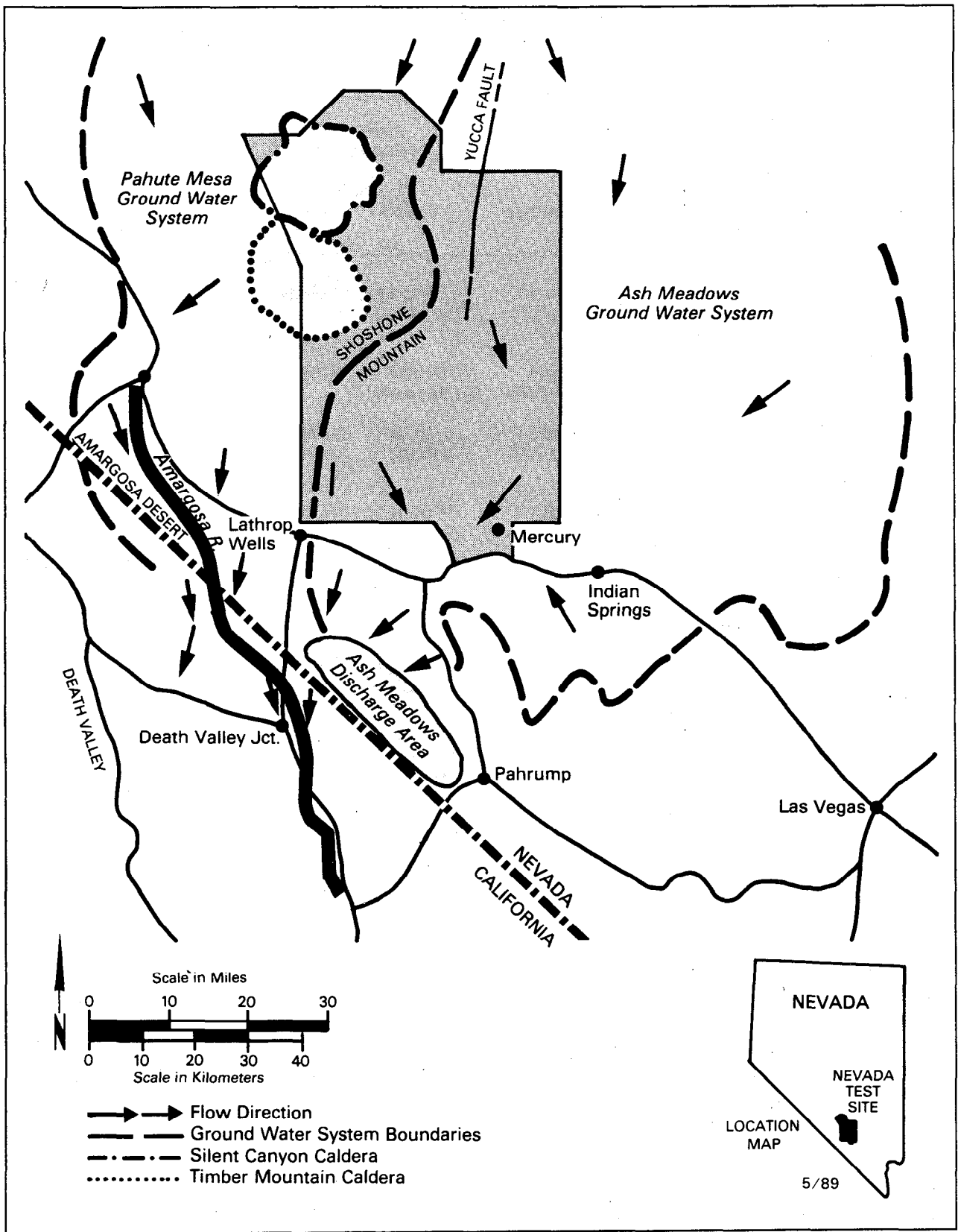
Figure 2. Ground Water Flow Systems Around the Nevada Test Site
