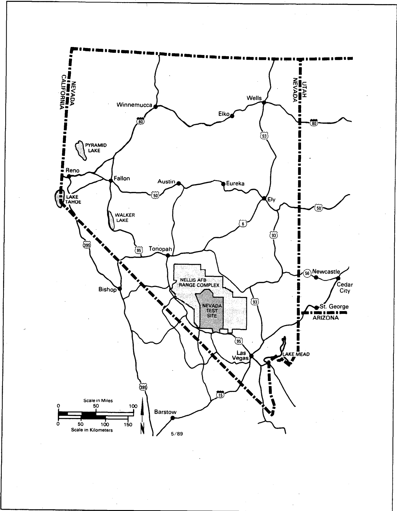
Figure 1. Location of the Nevada Test Site (NTS).
