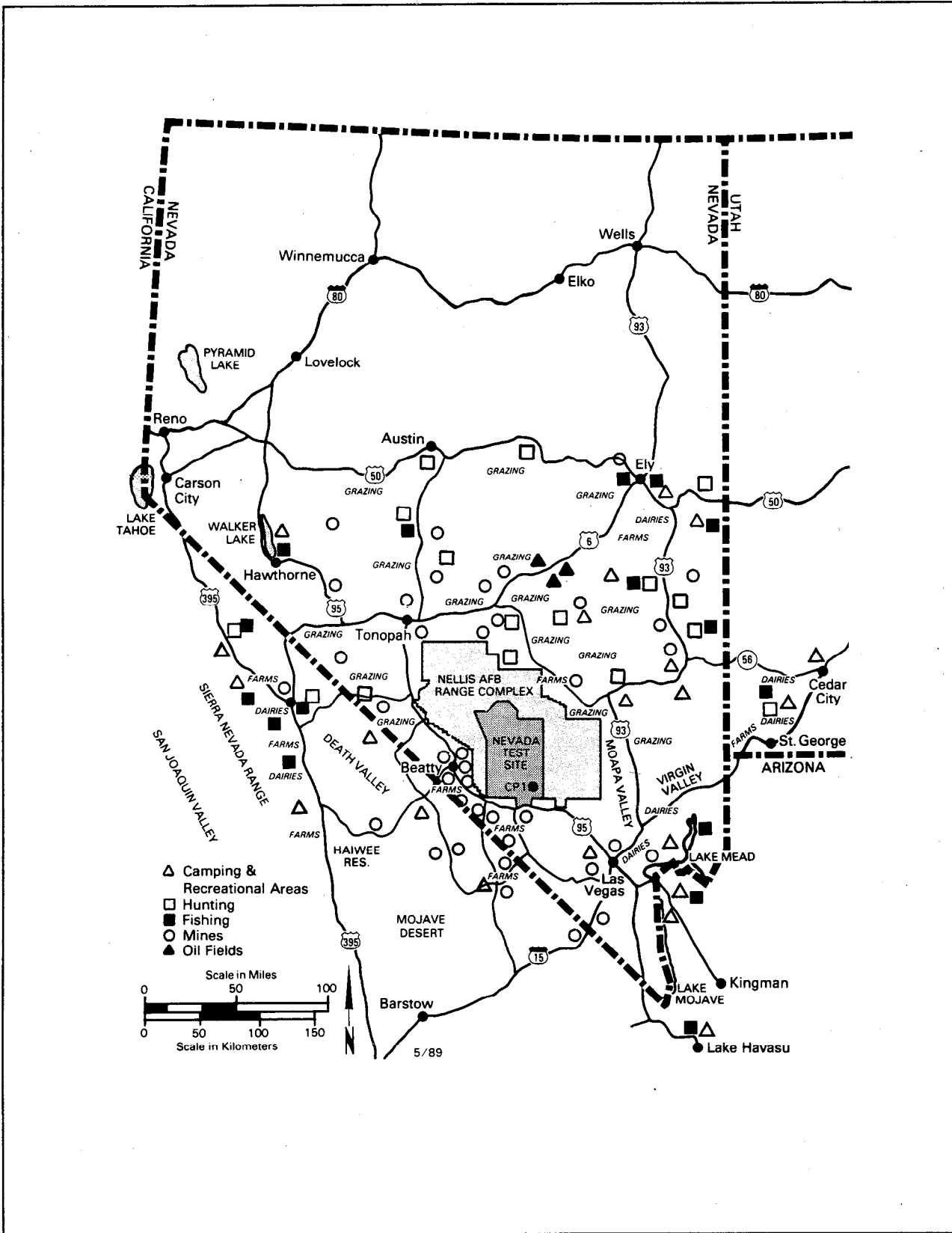
Figure 3. General Land Use Within 300 km of the Nevada Test Site.
