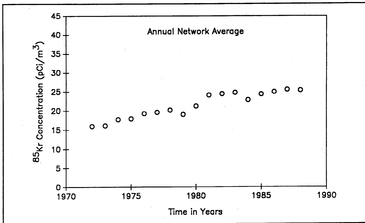
Figure 14. Annual Network Average 85 Kr Concentration.
