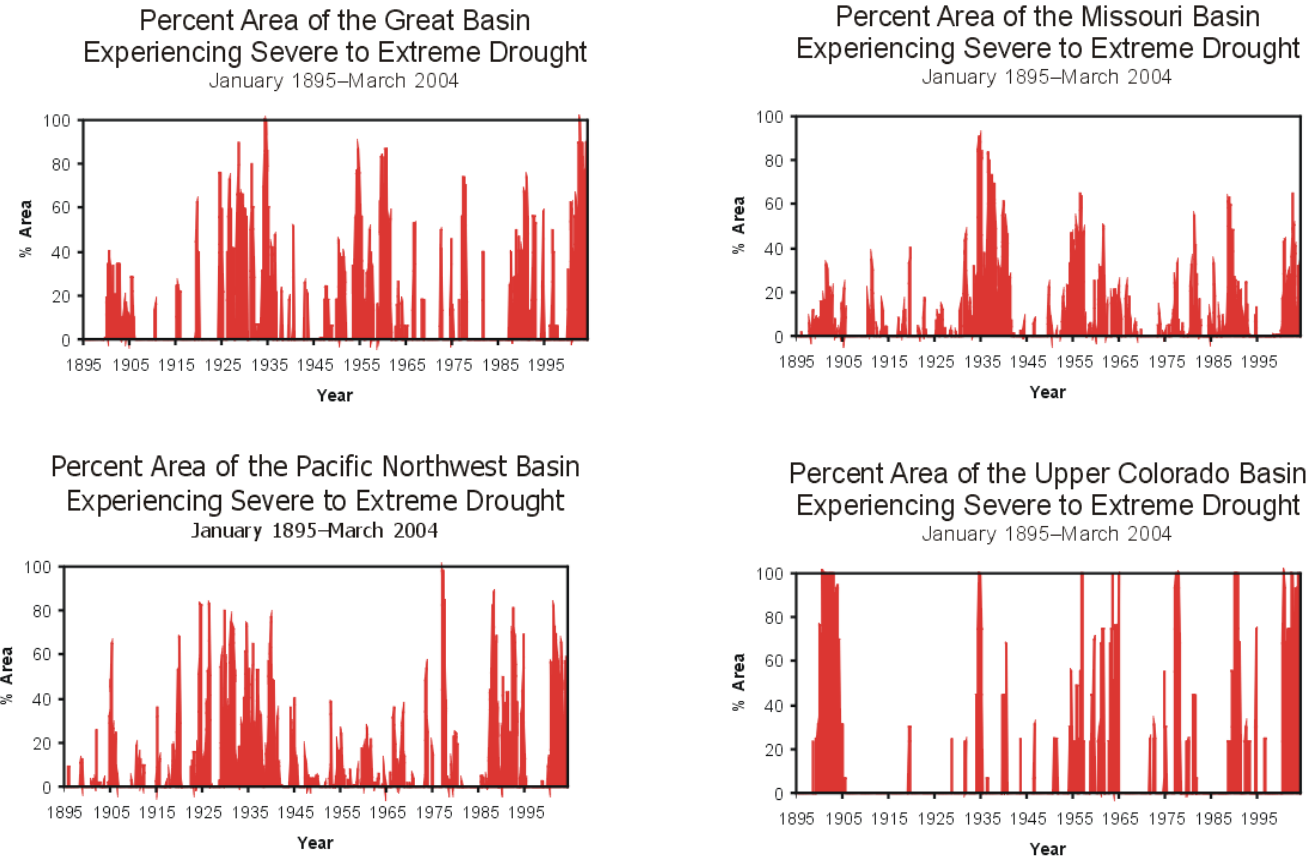
Fig. 7.11. Percent of major river basins experiencing drought conditions from 1895 to 2004 (U.S. National Drought Mitigation Center 2004). The graphs represent the Palmer Drought Severity Index (1965), which measures the degree of departure based on precipitation, temperature, and available water capacity.
