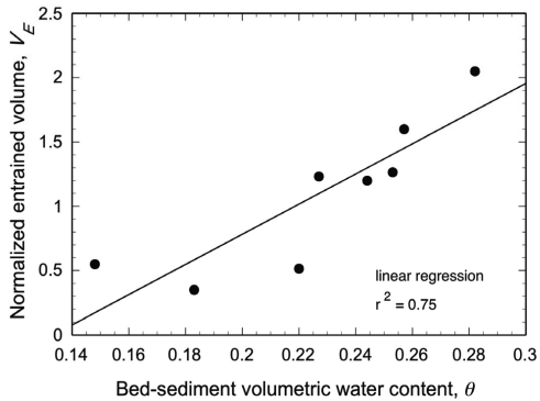
Fig. 3 - Normalized volume of sediment entrained, V_E (entrained volume/control debris-flow volume of 6 m 3 ) as a function of bed-sediment volumetric water content, \theta . Normalization differs from that of IVERSON, et alii (2011)
