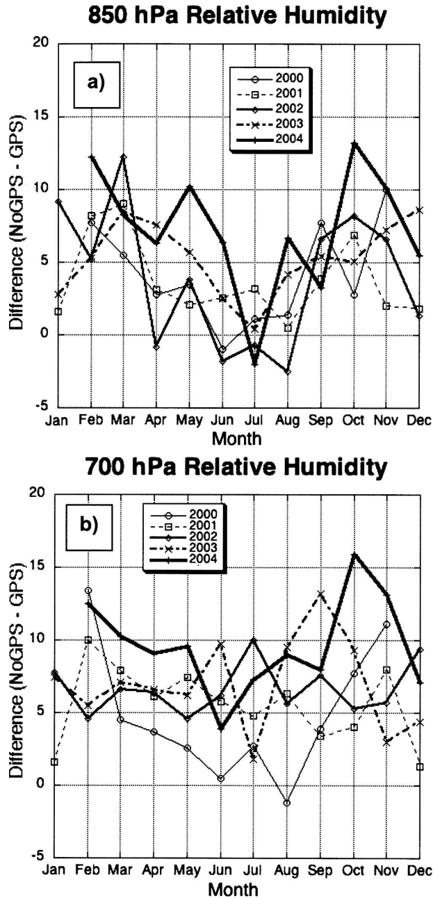
FIG. 4. Same as in Fig. 2, but by month for years 2000–04 for (a) 850 and (b) 700 hPa. (Note: some months were missing because of processing problems.)
