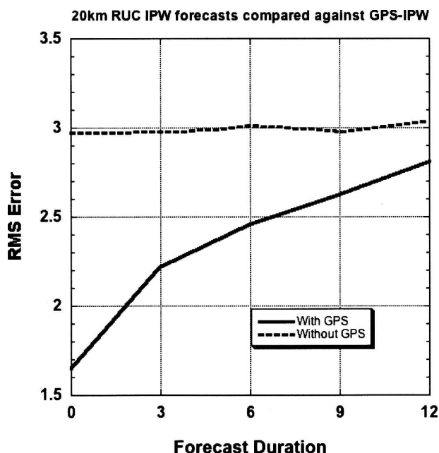
FIG. 6. IPW RMS error (mm) for RUC20 IPW analysis/forecast grids against GPS-IPW observations at ~275 sites in the RUC continental United States (CONUS) domain. Statistics are for the 3-month period from 1 Mar to 31 May 2004. RUC20 with GPS is solid; RUC20 without GPS is dashed.
