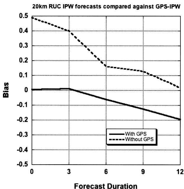
FIG. 7. Same as in Fig. 6, but for bias (RUC gridded IPW minus GPS-IPW).
