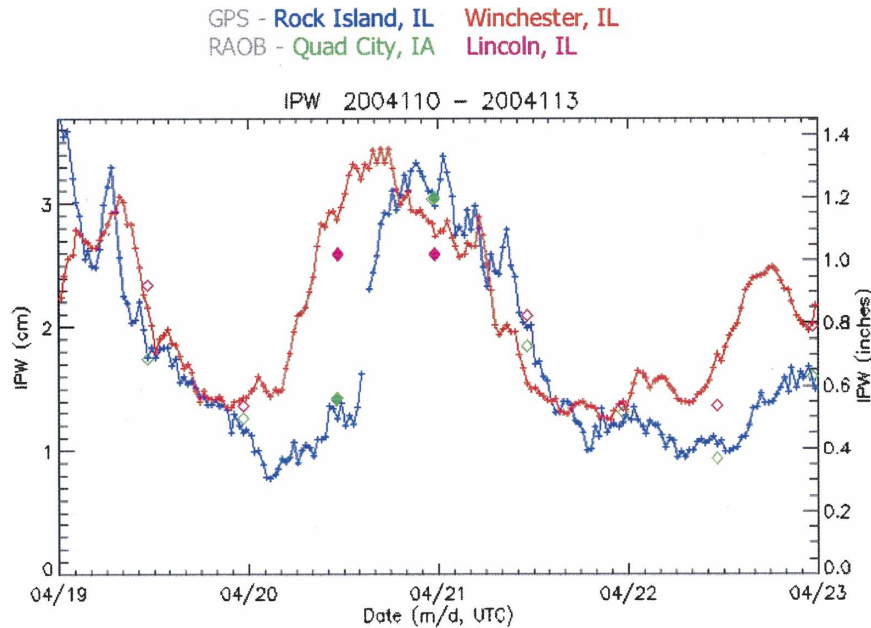
FIG. 11. IPW observations (cm) for 19–22 Apr 2004. GPS-IPW time series at Rock Island, IL (blue), and Winchester, IL (red). IPW plots every 12 h from rawinsondes at Davenport, IA (green diamonds), and Lincoln, IL (pink diamonds).
