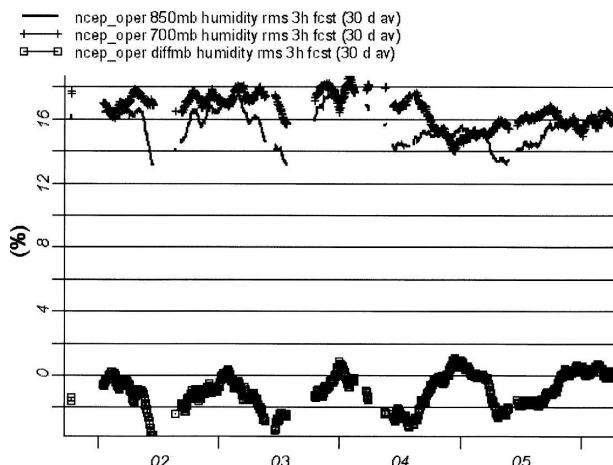
FIG. 16. The 3-h relative humidity forecast error from the operational RUC model at 850 hPa (top, solid), 700 hPa (top, crosses), and 700–850-hPa error difference (bottom, boxes) from January 2002 to April 2006 for full national RUC domain. A 30-day running mean was applied to verification every 12 h at raob launch times, and missing values are caused by missing data in the ESRL/GSD verification archive.
