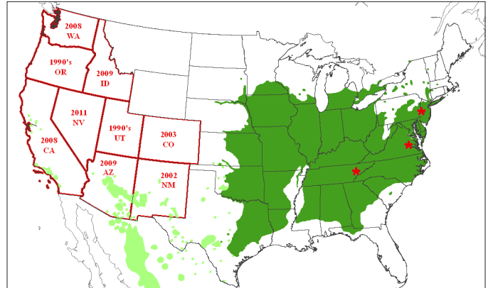
Figure 1. Thousand cankers disease occurs in 9 western states; the year in which the disease was confirmed is noted. Since 2010, TCD has been found in three locations in the East (TN, VA, PA - see *). The native ranges of eastern black walnut (dark green) and four western black walnut species (light green) are shown. Eastern black walnut is widely planted in the West, but is not depicted on this map.
