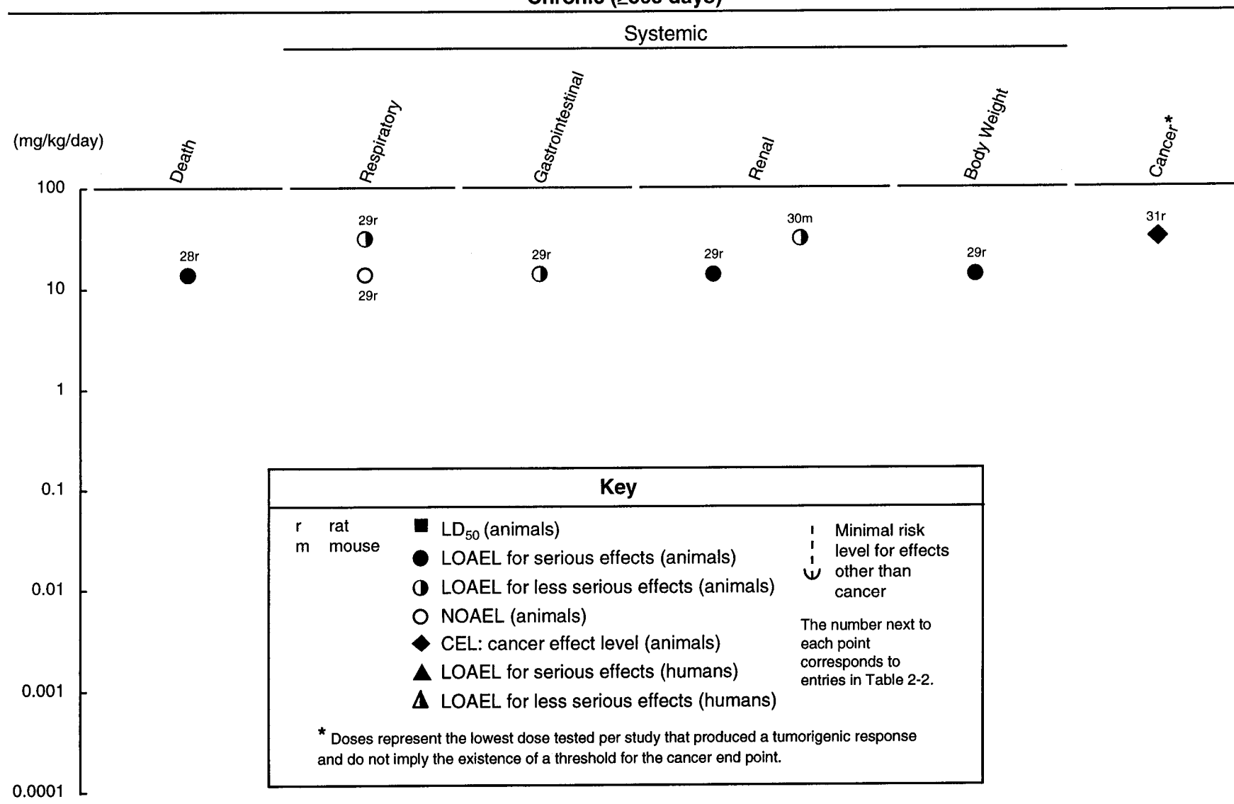
Figure 2-2. Levels of Significant Exposure to Inorganic Mercury - Oral (cont.)
