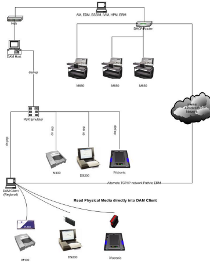
ES&S 4.0 Dial-up and TCP/IP Network Configuration Layout
