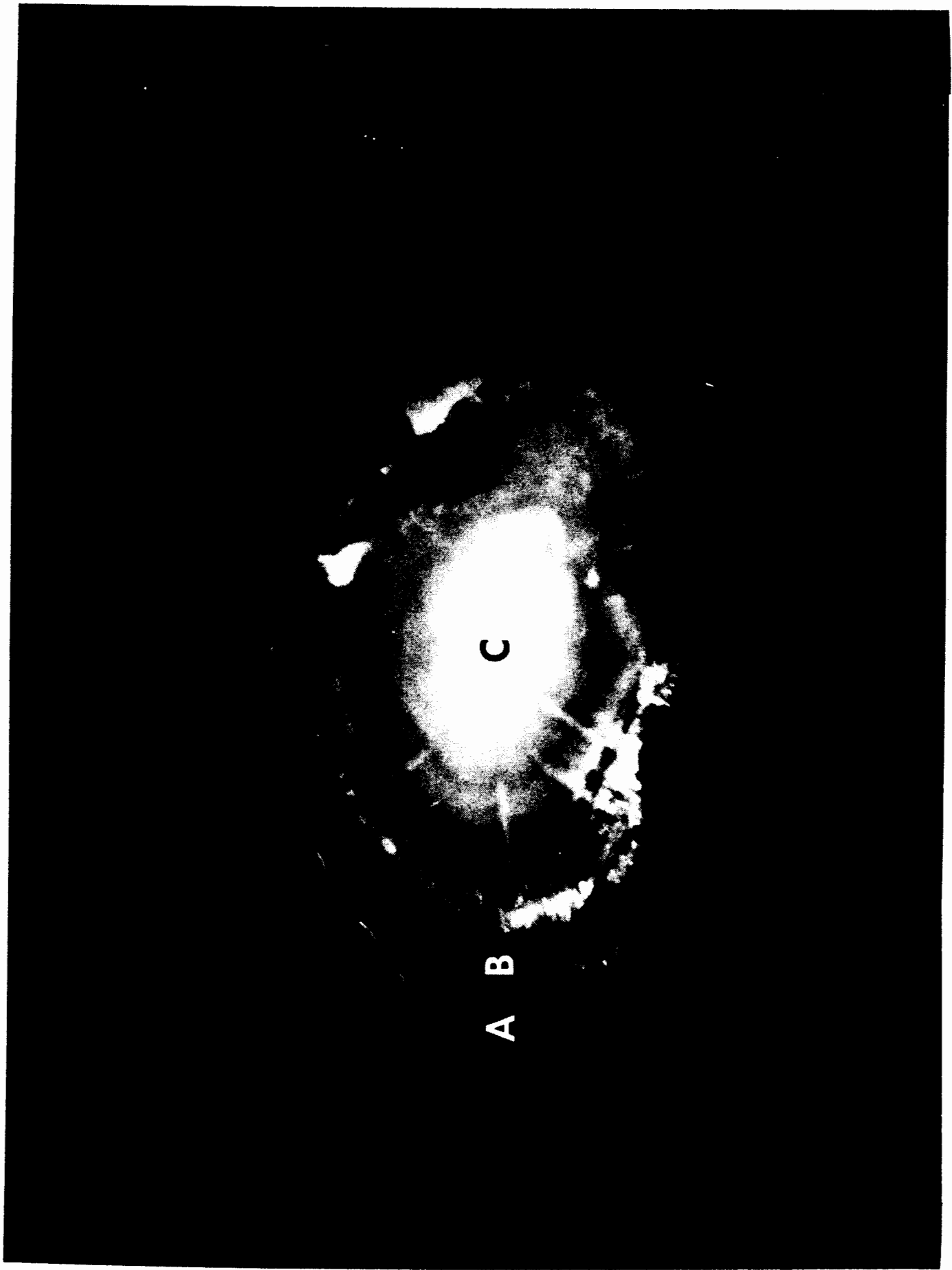
Figure 2. Whole otolith of a spot under reflected light (A - anterior edge, B - opaque zone, and C - focus).
