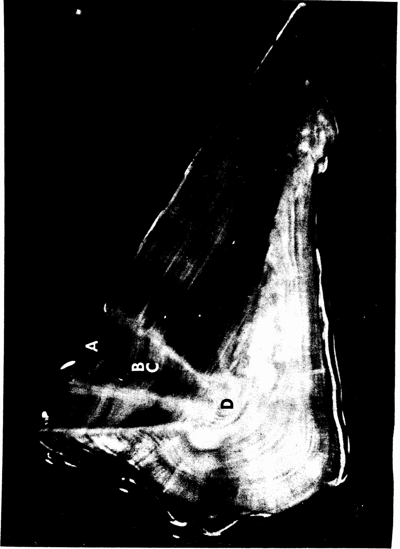
Figure 1. Cross section of an Atlantic croaker otolith under reflected light (A - proximal margin, B - hyaline zone, C - opaque zone, and D - focus).
