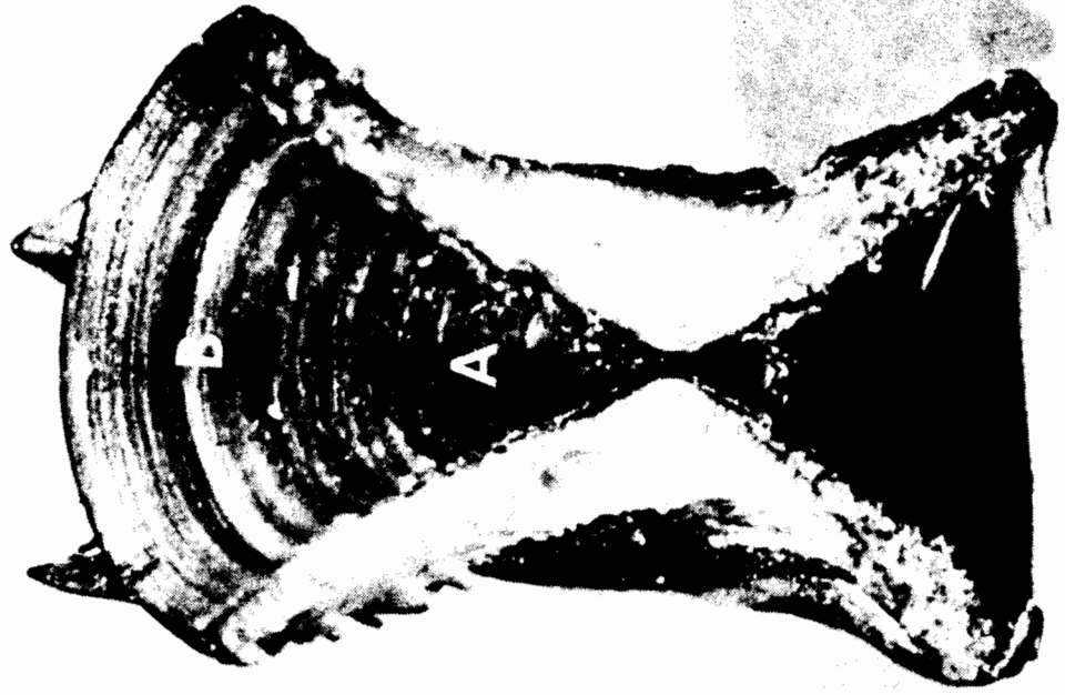
Figure 4. Atlantic croaker vertebral centrum (A - groove and B - ridge).
