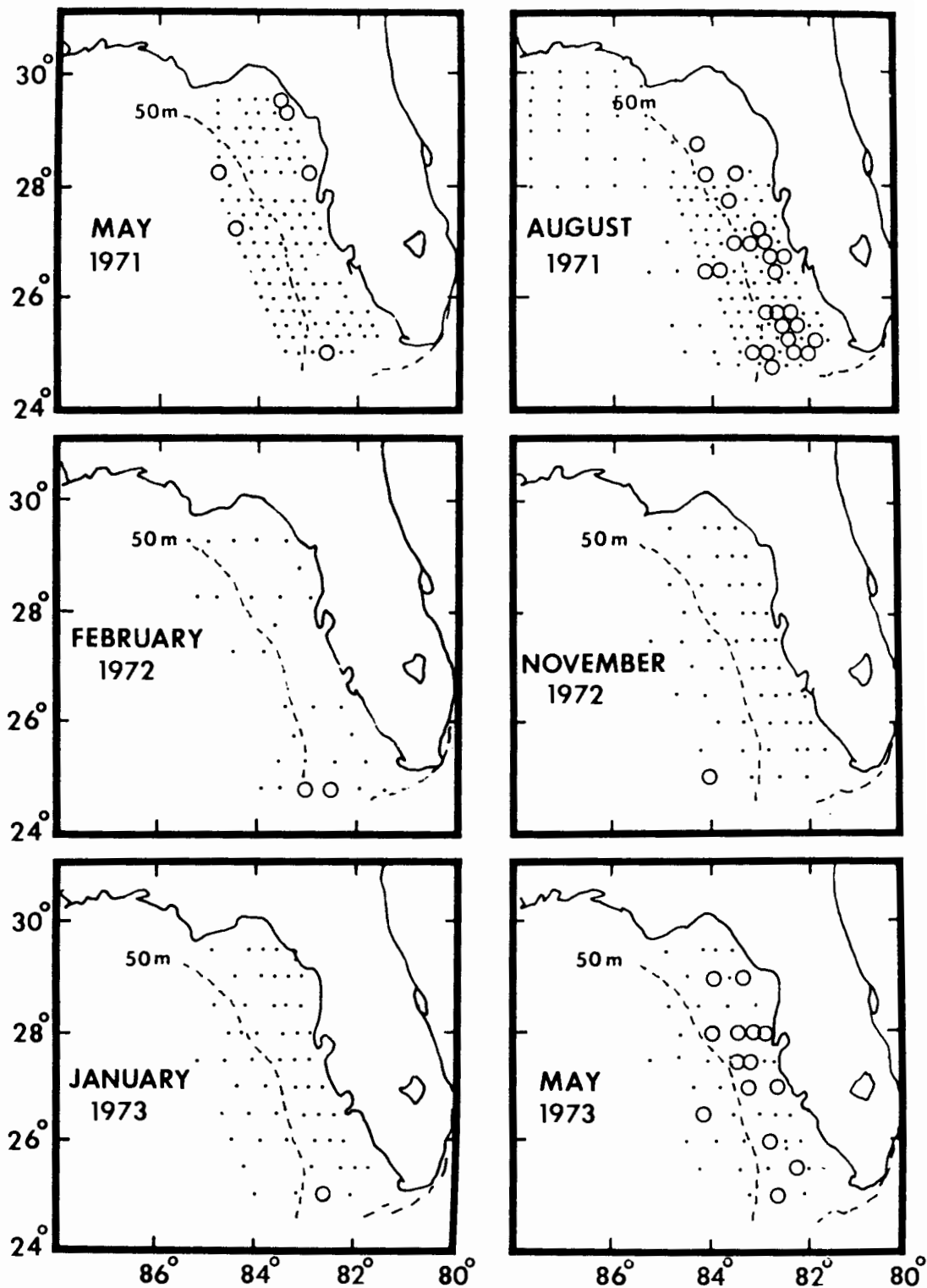
Figure 7. Distribution and abundance of S. aurita larvae in the eastern Gulf of Mexico, 1971-1974. 0 = tows in which larvae occurred (Houde et al. 1979).
