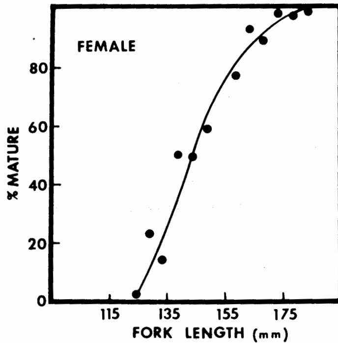
Figure 14. Frequency of mature S. aurita by fork length (Graff 1984).
