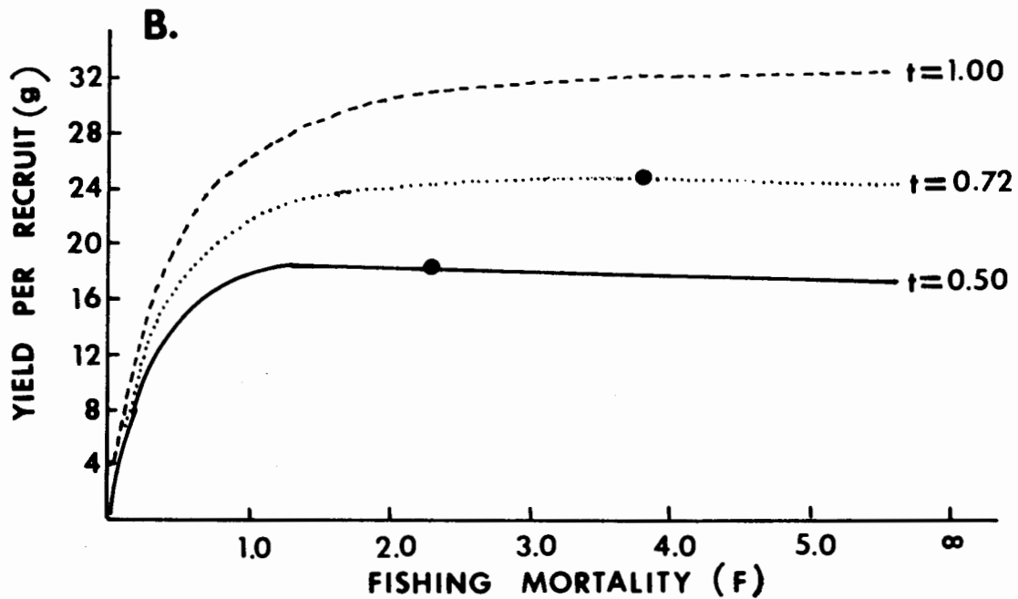
Figure 21. Yield-per-recruit curves assuming several ages at first capture ( t ) under various fishing mortalities ( F ) based on approximately first annulus formation at (A) one year of age or (B) six months of age of S. aurita (Grall 1984).
