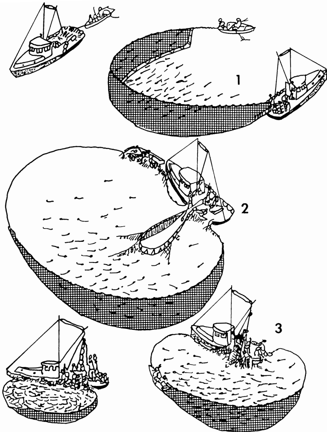
Figure 25. Sequence of purse seine operation: 1) setting the net 2) pursing 3) haul in purse seine rings and leadline (Roithmayr 1983).
