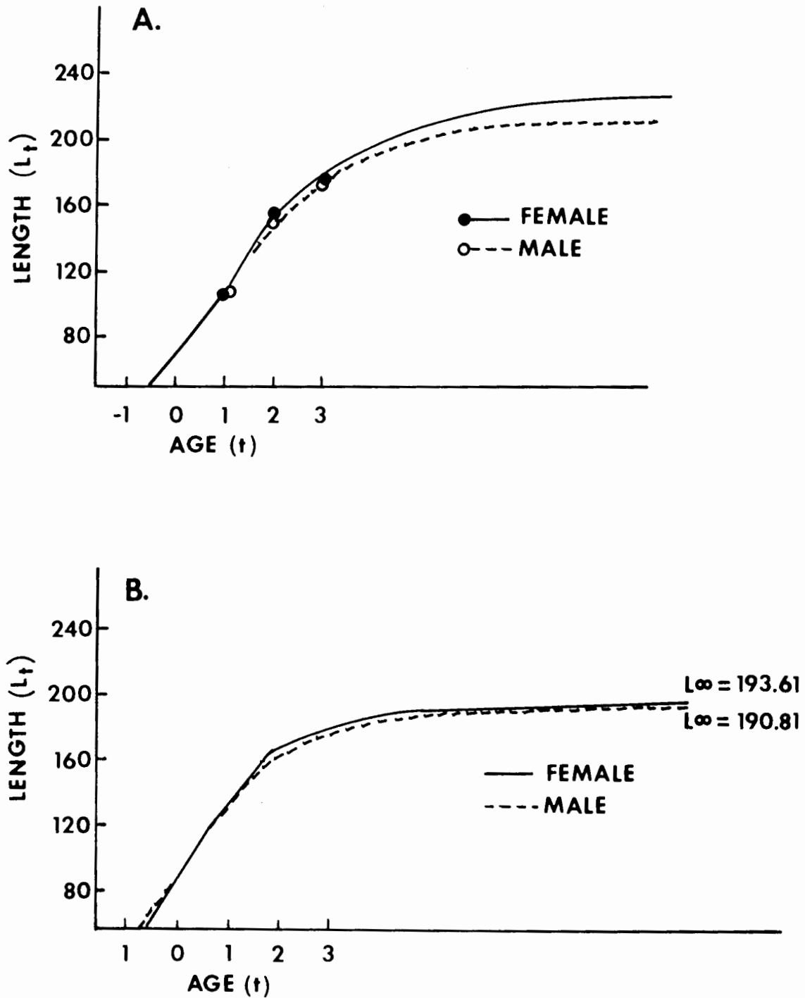
Figure 20. The von Bertalanffy growth curve fitted to age data based on first annulus formation at approximately (A) one year of age or (B) six months of age of S. aurita (Grall 1984).
