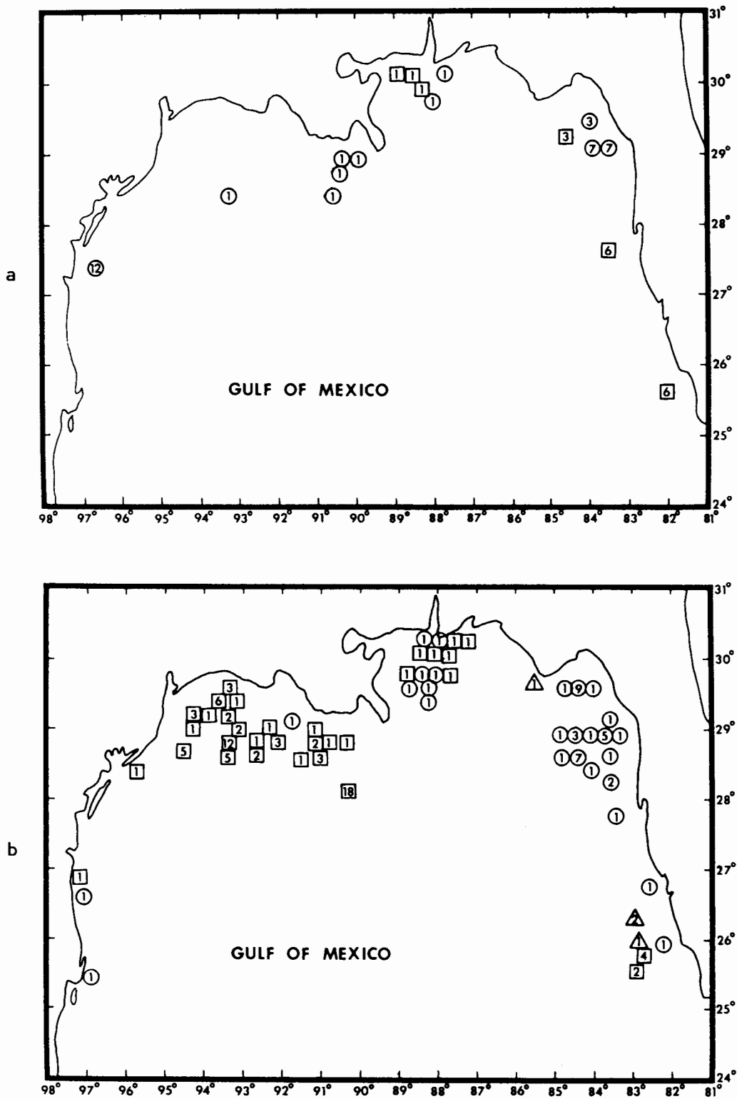
Figure 9. Catch rates for exploratory fishing for S. aurita , 1950 to 1985. a) Fall-winter (0=fall; ◻=winter) b) spring-summer (O=spring; ◻=summer). Also, O and ◻ are bottom trawls; ◻ are mid-water trawls. Numbers are pounds/hr. Information from Frederick Minkler, NMFS, Pascagoula Laboratory, Miss., May 1985.
