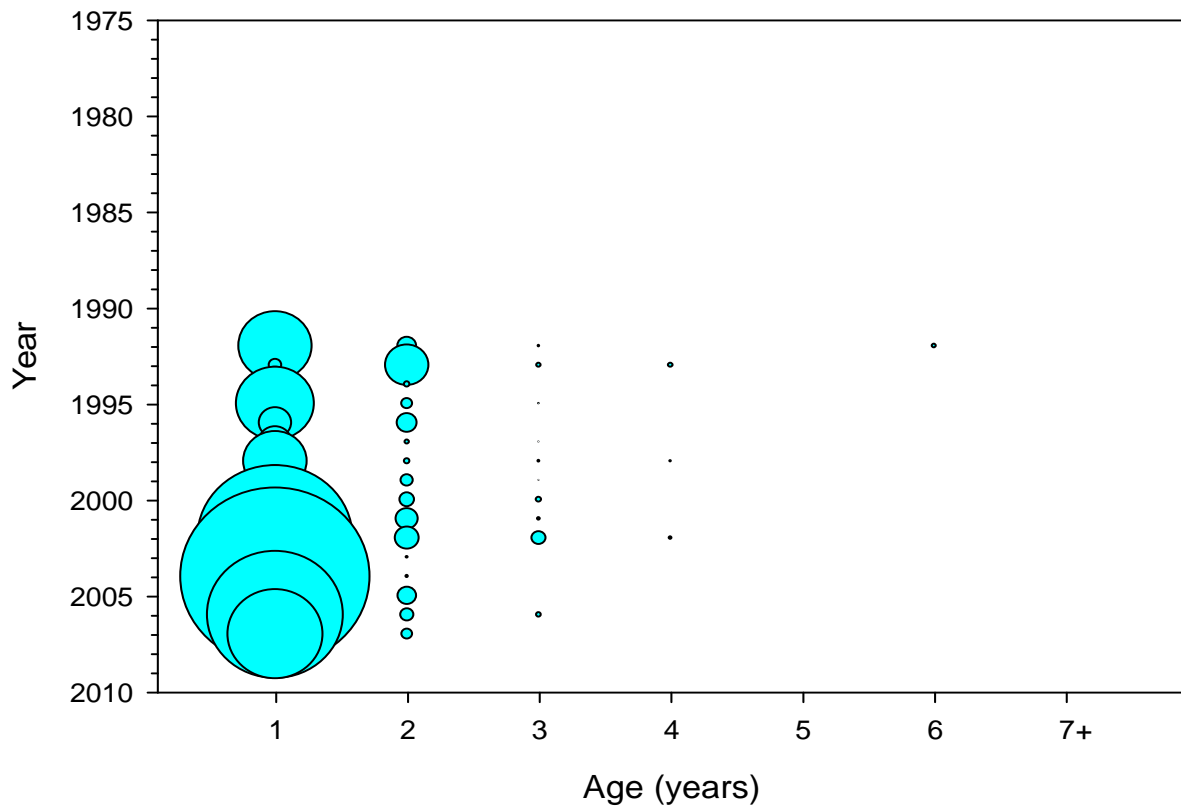
Figure 9. NEFSC Winter survey indices by age for scup.
