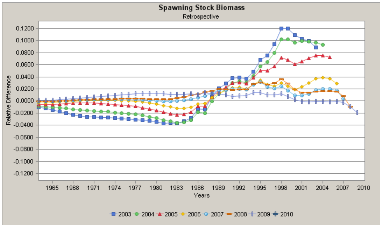
Figure 25. Retrospective analysis of the ASAP SCAA: Spawning Stock Biomass.
