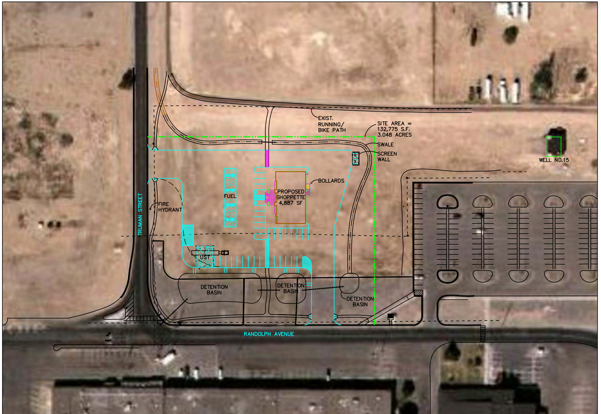
FIGURE 2-2 PRELIMINARY SITE PLAN
