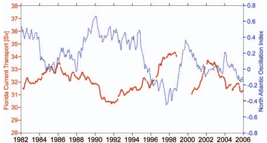
FIG. 3.10. Florida Current transport (Sv; red solid) as measured by the NOAA-funded submarine cable across the Florida Straits, along with the NAO index (blue dashed) produced by NOAA/NCEP.
