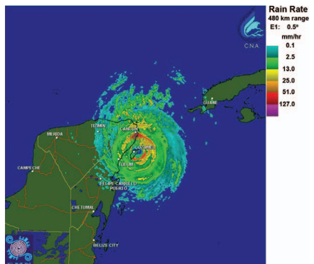
FIG. 4.6. Mexican Meteorological Service radar image of category 5 Hurricane Wilma striking the Yucatan Peninsula on 21 Oct 2005. [Source: Servicio Meteorológico Nacional]
