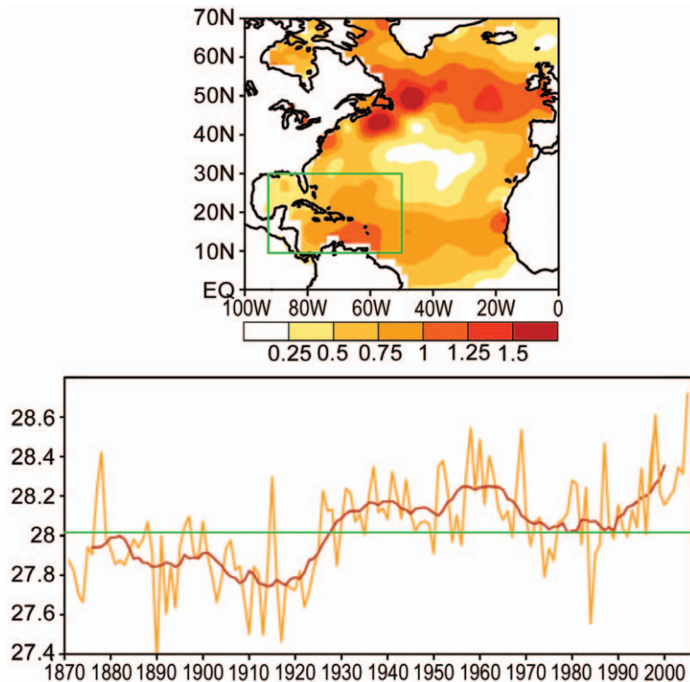
FIG. 4.12. Seasonal June–November (top) SST anomalies ( ^{\circ}\text{C} ) during 2005 and (bottom) time series of area-averaged SSTs ( ^{\circ}\text{C} ) in the (top) green boxed region. (bottom) Red line shows the corresponding 11-yr running mean. Averaging region corresponds to where seasonal activity was heavily focused during 2005.
