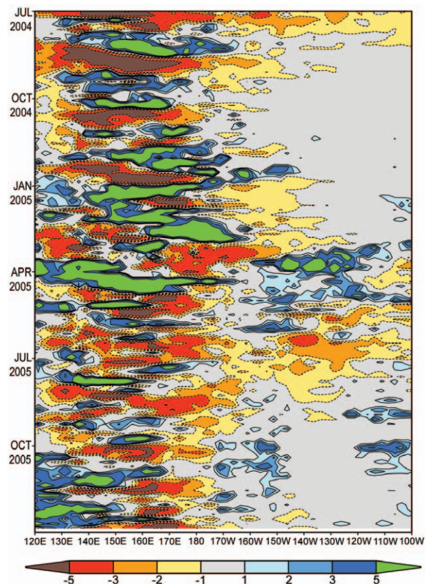
FIG. 2.13. Time–longitude section of precipitation anomaly (mm; 1979–95 base period) averaged over the tropical Pacific (5°S–5°N) as observed by the Global Precipitation Climatology Project (GPCP) pentad precipitation dataset (Xie et al. 2003).
