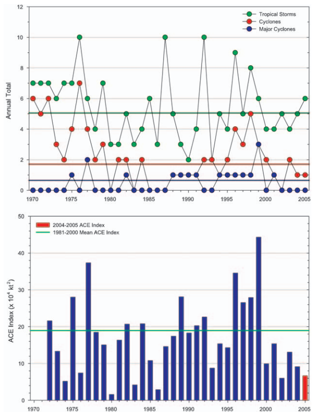
FIG. 4.18. Annual tropical cyclone statistics for the NIO 1970–2005. (top) Number of tropical storms, cyclones, and major cyclones. (bottom) Estimated annual ACE Index ( \times 10^4 kt 2 ) for all NIO tropical cyclones during which they were at least tropical storm or greater intensities (Bell et al. 2000). The ACE Index is estimated due to a lack of consistent 6-h sustained winds data for every storm.
