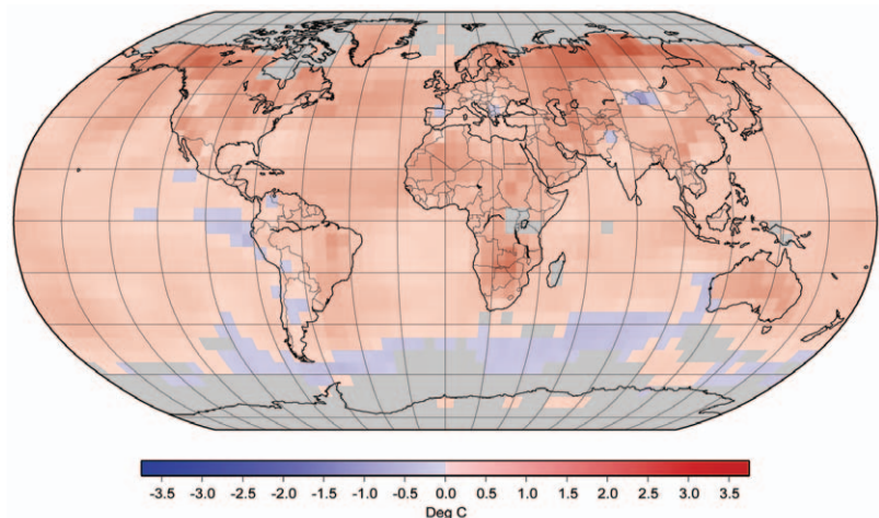
FIG. 2.4. Geographic distribution of surface air temperature anomalies (°C) in 2005 relative to the 1961–90 mean. [Source: NOAA/NCDC]
