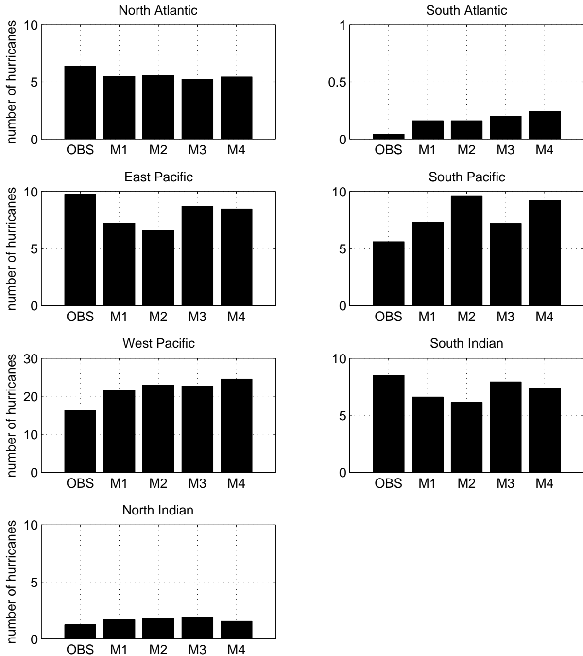
Figure 4. A comparison of observed and simulated annual mean hurricane count for each ocean basin averaged over 1981 to 2005. M1, M2, M3, M4 represent each integration of the 4-member ensemble.
