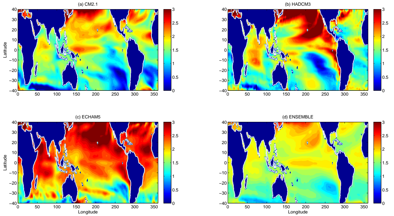
Figure 12. Aug-Sept-Oct seasonal mean SST anomaly from a) GFDL CM2.1, b) UKMO HADCM3, c) MPI ECHAM5 and d) multi-model ensemble mean (see detailed description in the text). Unit: ^{\circ}\text{K} .
