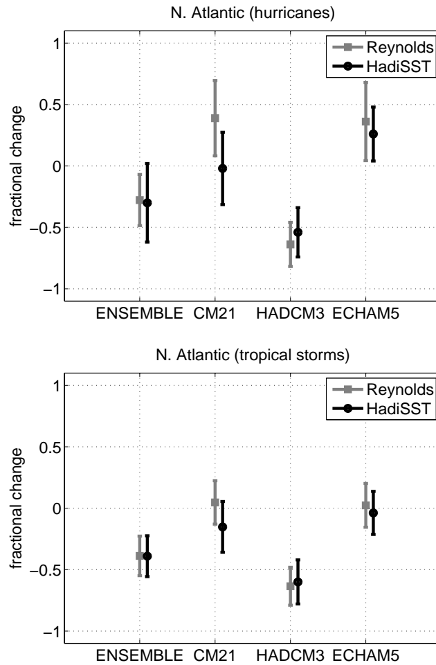
Figure 13. Fractional changes in annual hurricane (upper) and tropical storm (lower) count for the North Atlantic basin from the 4 SST anomaly simulations based on 2 different control climatological-SSTs. Error bars show the 90% confidence level assuming the sampling distributions are normally distributed. Legend shows the two control climatological-SSTs.
