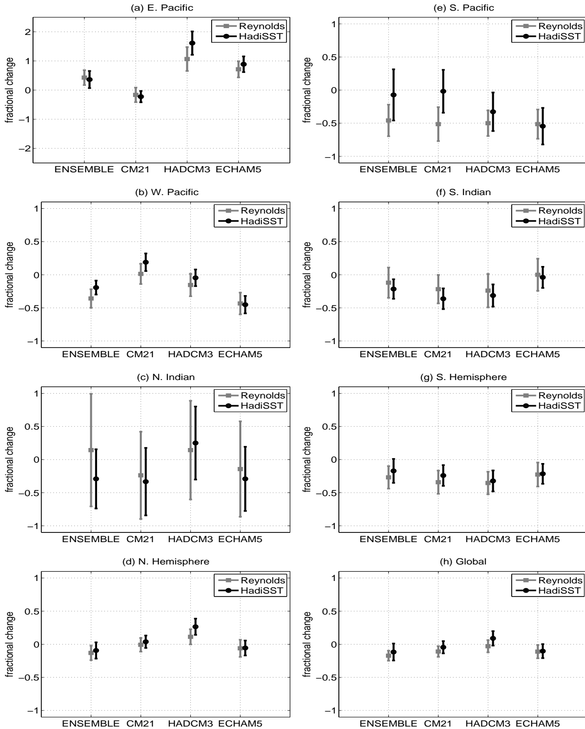
Figure 17. Fractional changes in annual hurricane counts (as in Fig 13a) except for a) East Pacific, b) West Pacific c) North Indian, d) Northern Hemisphere, e) South Pacific, f) South Indian, g) Southern Hemisphere, and h) the global ocean. Error bars show the 90% confidence level assuming the sampling distributions are normally distributed.
