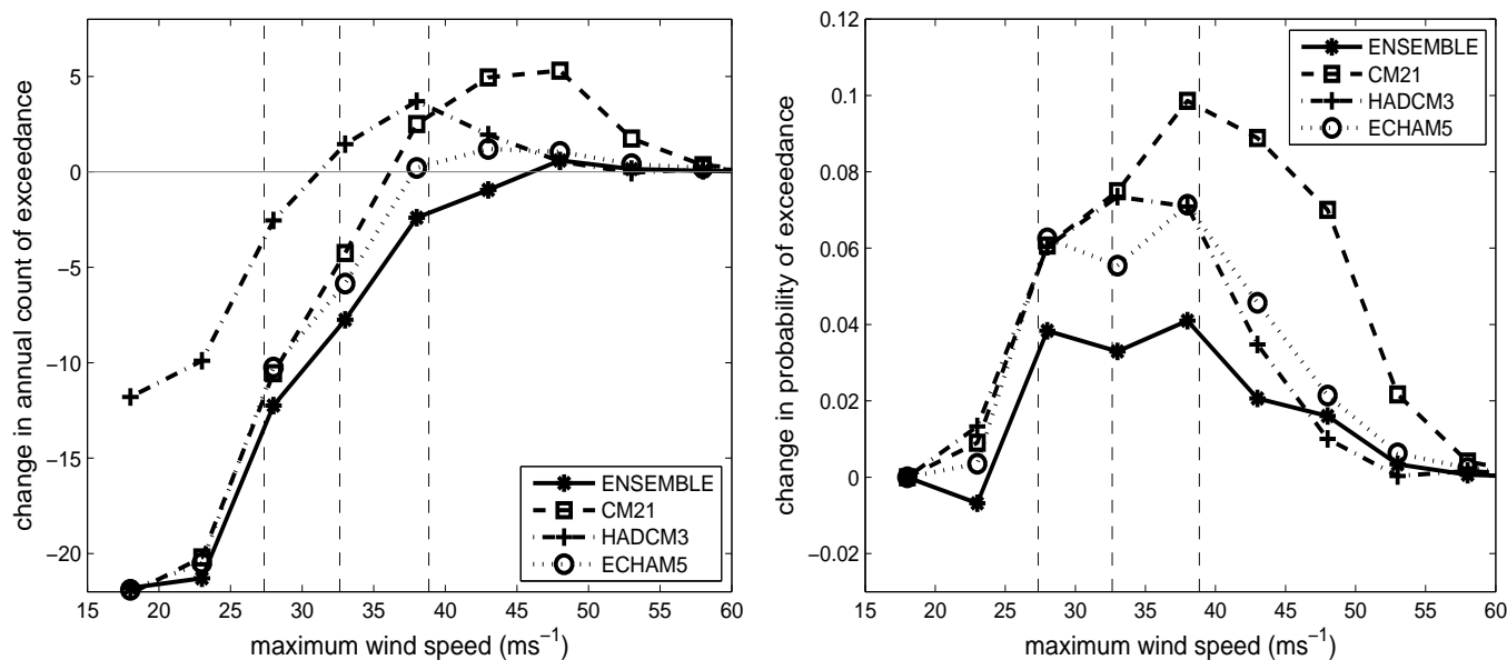
Figure 18. a) Change (warming minus control) in annual storm count exceeding a given surface maximum wind for the entire global tropical ocean. Vertical lines show the lower quartile, median, and upper quartile of the controls. b) As in a) but show change in the probability of exceedance of tropical storm intensity. Positive value indicates relative increase in the fraction of storms with maximum surface wind speed above the corresponding value.
