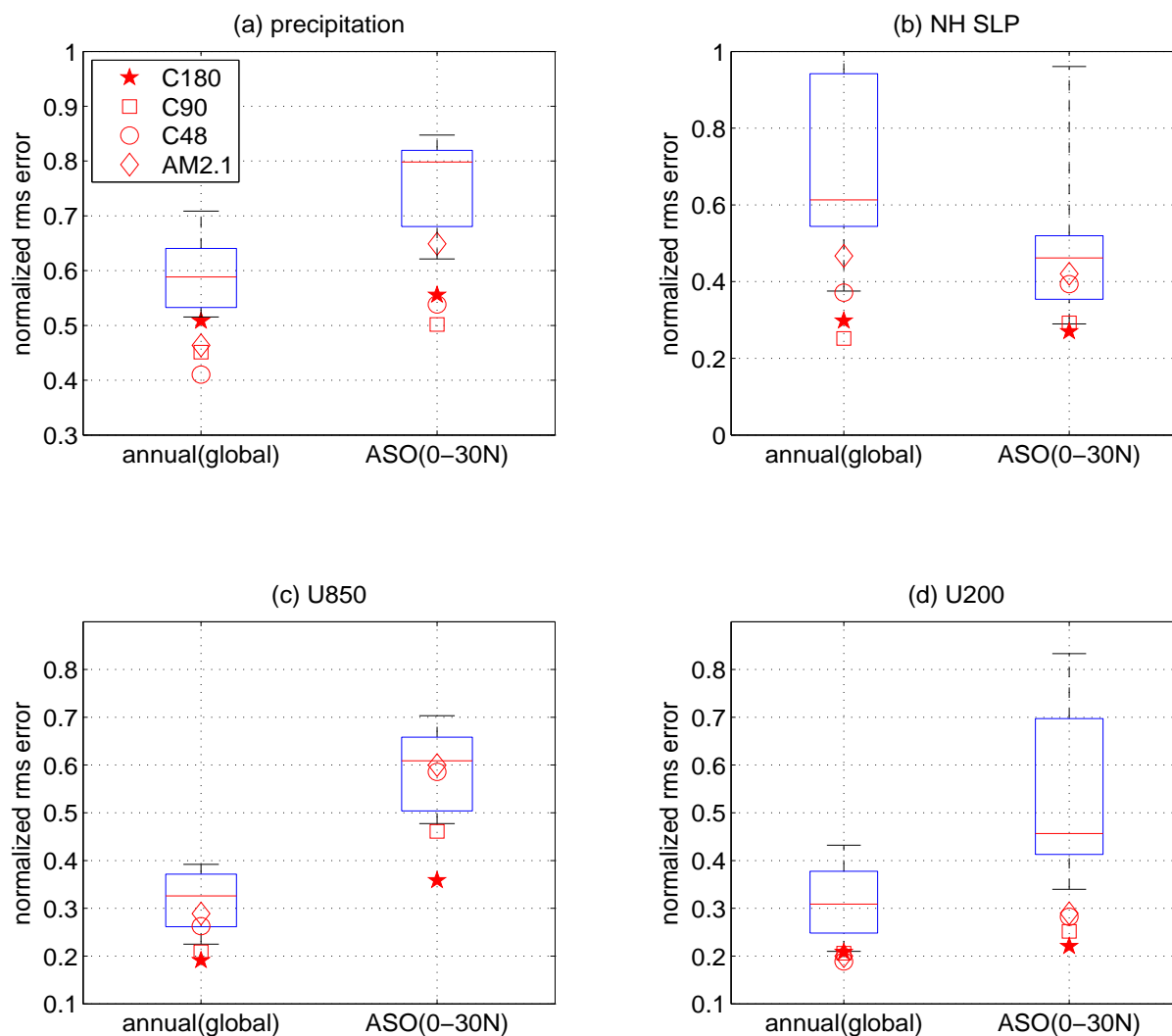
Figure 2. A comparison of RMS error (normalized by observed standard deviation of spatial variation of each time-mean field) of selected fields from the C180, C90, C48 HIRAM2.1 and the standard AM2.1 integrations with prescribed SSTs (1981-2005). The boxes show the lower quartiles, medians (red lines), and upper quartiles of 10 other model runs from the CMIP3 data base, while the whiskers show the max and min values among these models. a) Precipitation compared to CMAP; b) Northern Hemisphere sea level pressure (compared to NCEP-NCAR reanalysis); c) 850 hPa zonal wind (compared to NCEP-NCAR reanalysis); d) As in c) but for 200 hPa zonal wind.
