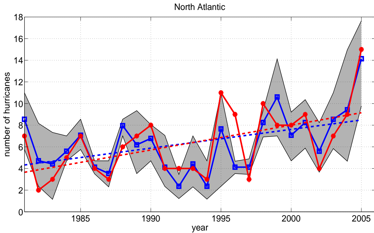
Figure 7. Interannual variation of hurricane numbers for North Atlantic from 1981 to 2005. Red: IBTrACS observations (Kruk et al. 2008); blue: 4-member ensemble mean; shaded area shows the simulated maximum and minimum number for each year from the 4 member integrations. Model time series are normalized by time-independent multiplicative factors so as to reproduce the observed total number. Dotted lines show observed and model (ensemble mean) linear trends.
