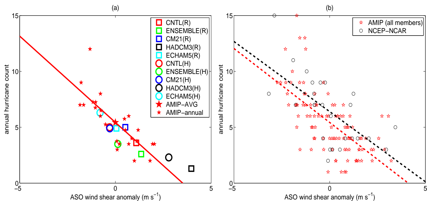
Figure 15. a) Scatter plot of annual Atlantic hurricane count versus ASO season vertical wind shear anomalies from the ensemble mean for each year of the 4 observed-SST simulations (small pentagrams). The big pentagram shows the AMIP all-year mean and the line is a linear regression of the 25 year data points. Also shown are results from the two control climatological-SST simulations (red symbols) and the various SST anomaly simulations (green: ENSEMBLE, blue: CM2.1, black: HADCM3, cyan: ECHAM5). Squares denote the set of experiments using Reynolds climatological-SST as a control, circles denote the set of experiments using HadISST climatological-SST as a control. For the control and SST anomaly simulations, the ASO wind shear anomalies are the mean ASO wind shear minus the AMIP all-year mean. b) As in a) except showing all members of the AMIP runs with all climate change experiments removed. Black circles show scatter plots of observed Atlantic hurricane count versus vertical wind shear calculated from NCEP-NCAR reanalysis. The red and black lines are respectively linear regression of the model and observation data points.
