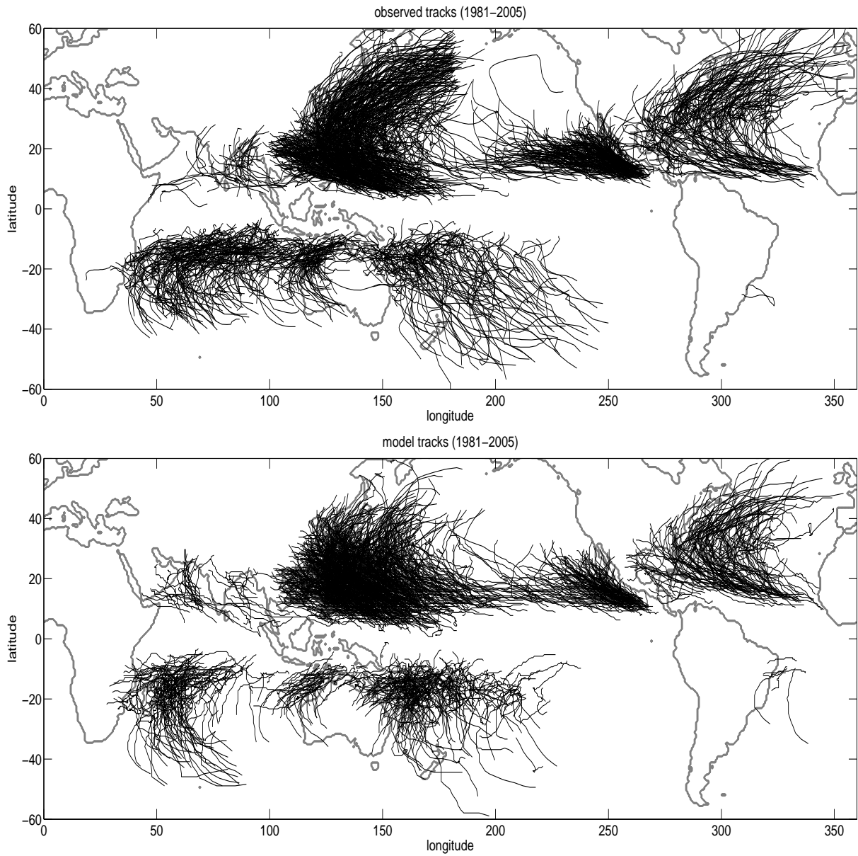
Figure 3. A comparison of observed (upper panel) and model simulated (lower panel) hurricane tracks from 1981 to 2005.
