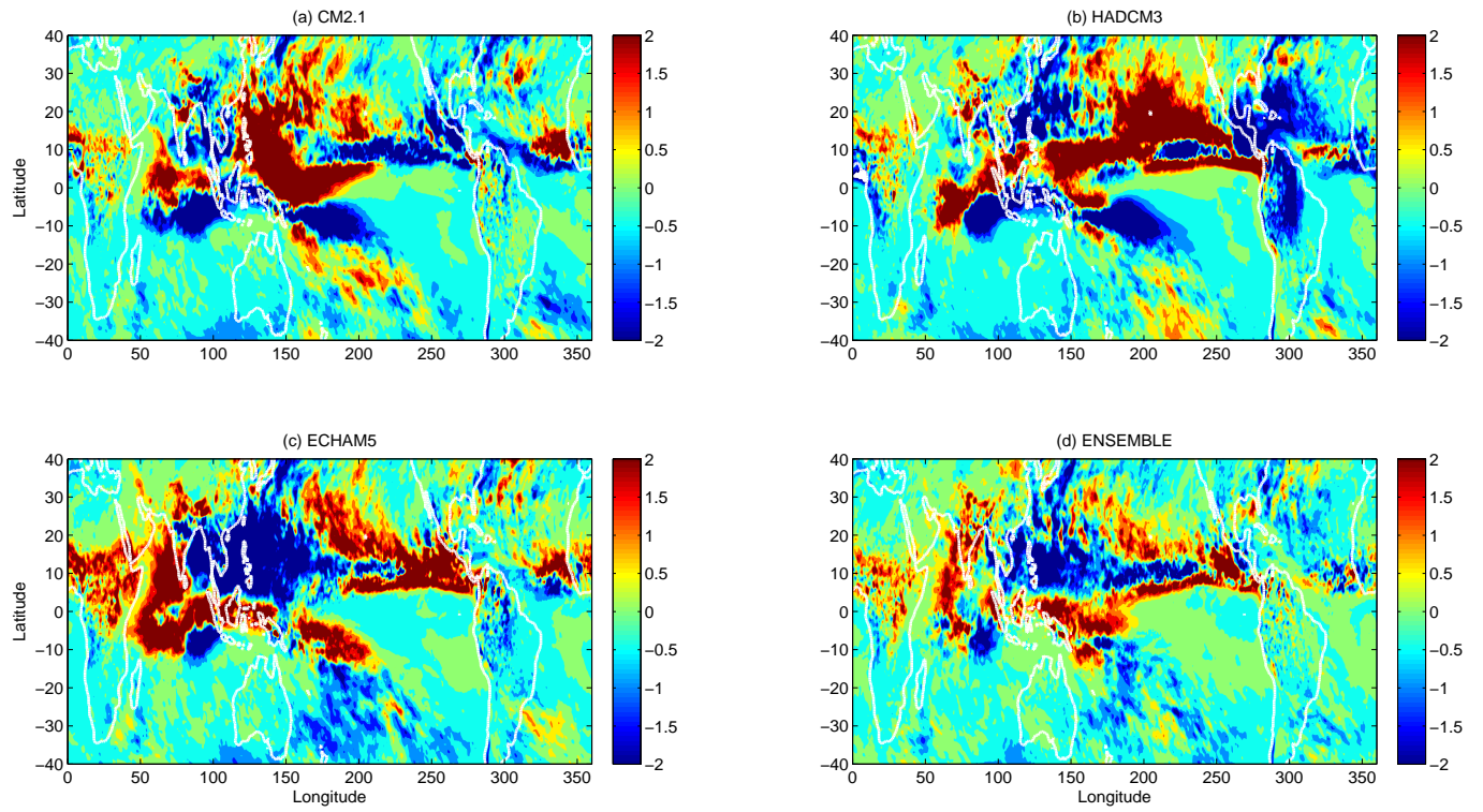
Figure 14. Aug-Sept-Oct seasonal mean precipitation differences between SST anomaly simulations and the control simulation. Unit: \text{mm day}^{-1} .
