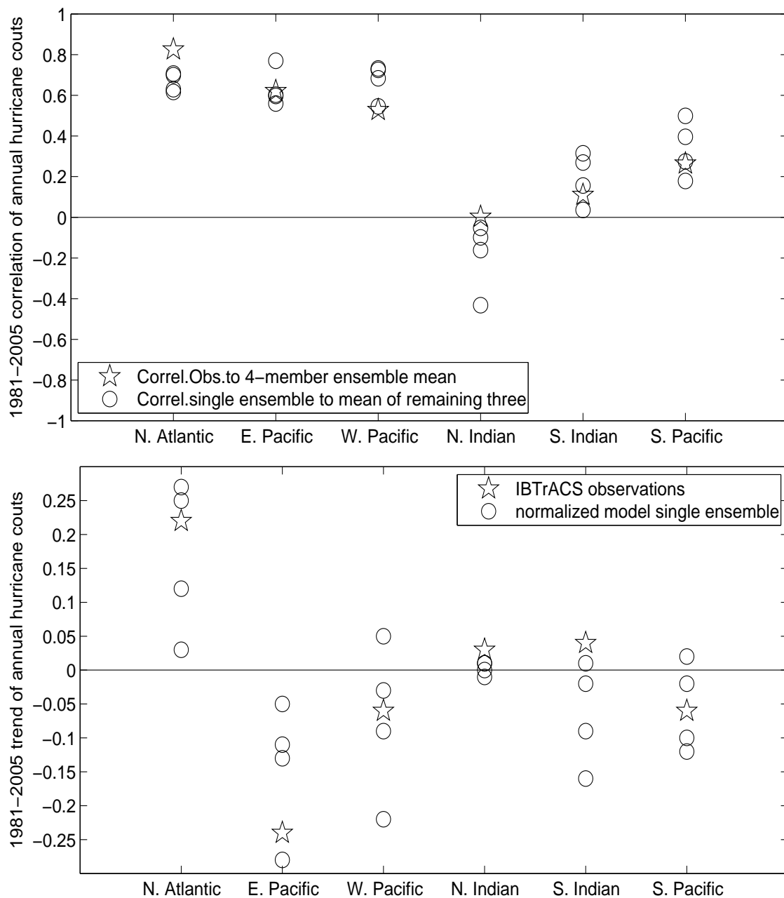
Figure 11. Upper panel: the correlation of observed hurricane count to the 4-member ensemble mean (stars) and the correlation of each ensemble member to the ensemble mean of the remaining three (circles) for each basin. Lower panel: observed (stars) and modeled (circles) linear trends in hurricane frequency for the period 1981-2005 in each basin. Model trends are from individual realizations and calculated from normalized time series.
