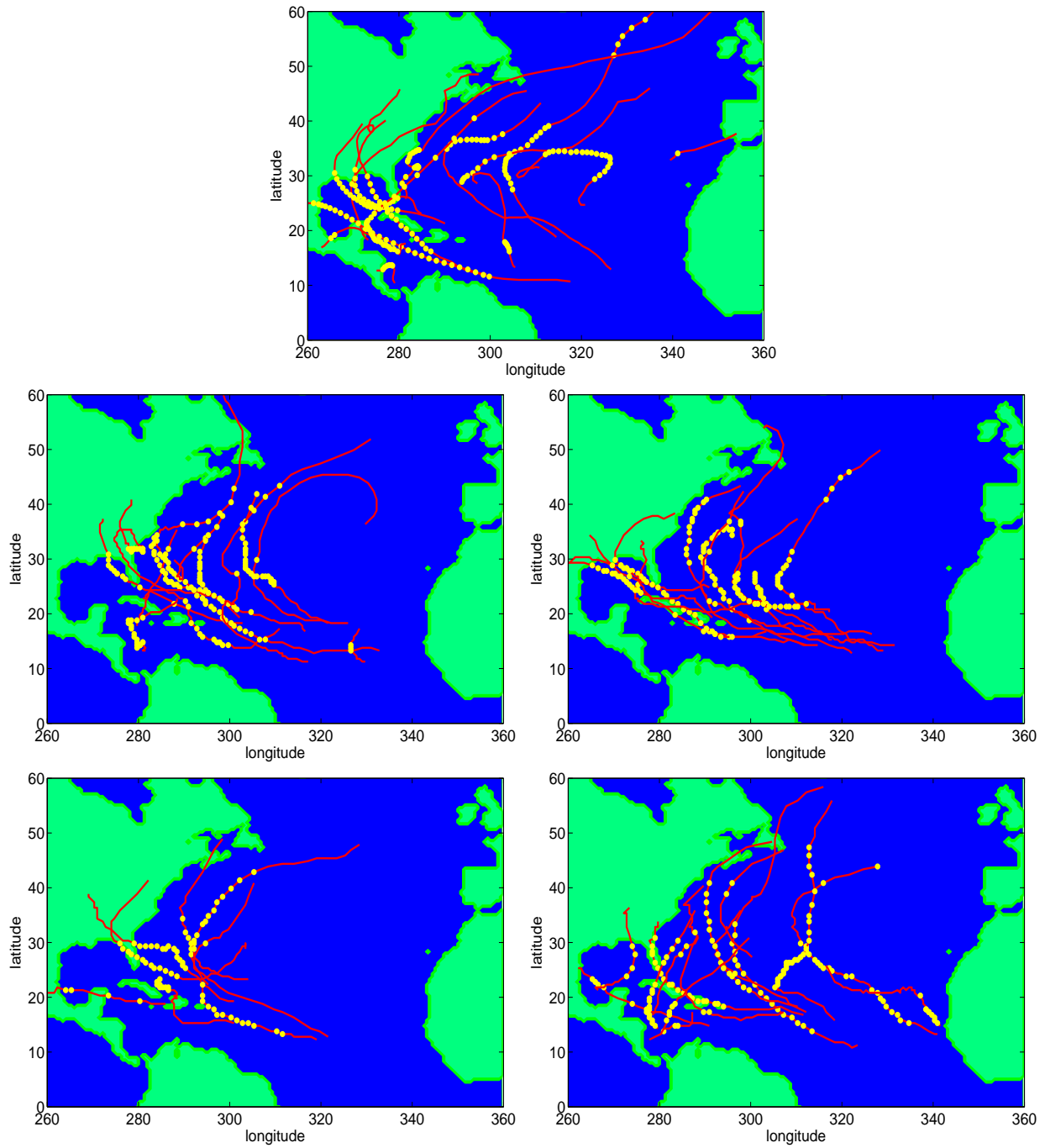
Figure 8. A comparison of observed and model simulated hurricane tracks for year 2005. Upper panel: observed tracks; middle and bottom panels: simulated tracks from each individual realization of the 4-member ensemble. Yellow dots show the locations where maximum wind speed exceeds 33 \text{ m s}^{-1} along each track.
