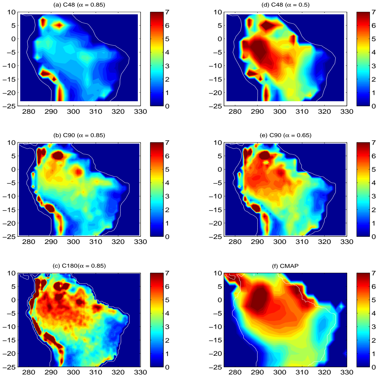
Figure 1. Sensitivity of annual mean Amazon precipitation to horizontal resolution and cumulus lateral mixing rate over land. Left column (panel a,b,c): the same physics except for the indicated resolution change, with a fixed ratio of land to ocean lateral mixing rates of \alpha=0.85 . Right column: panel d: as in a) except \alpha=0.5 ; panel e: as in b) except \alpha=0.65 ; panel f: observations from Climate Prediction Center Merged Analysis of Precipitation data (CMAP, Xie and Arkin 1996 ). Unit: mm day -1 .
