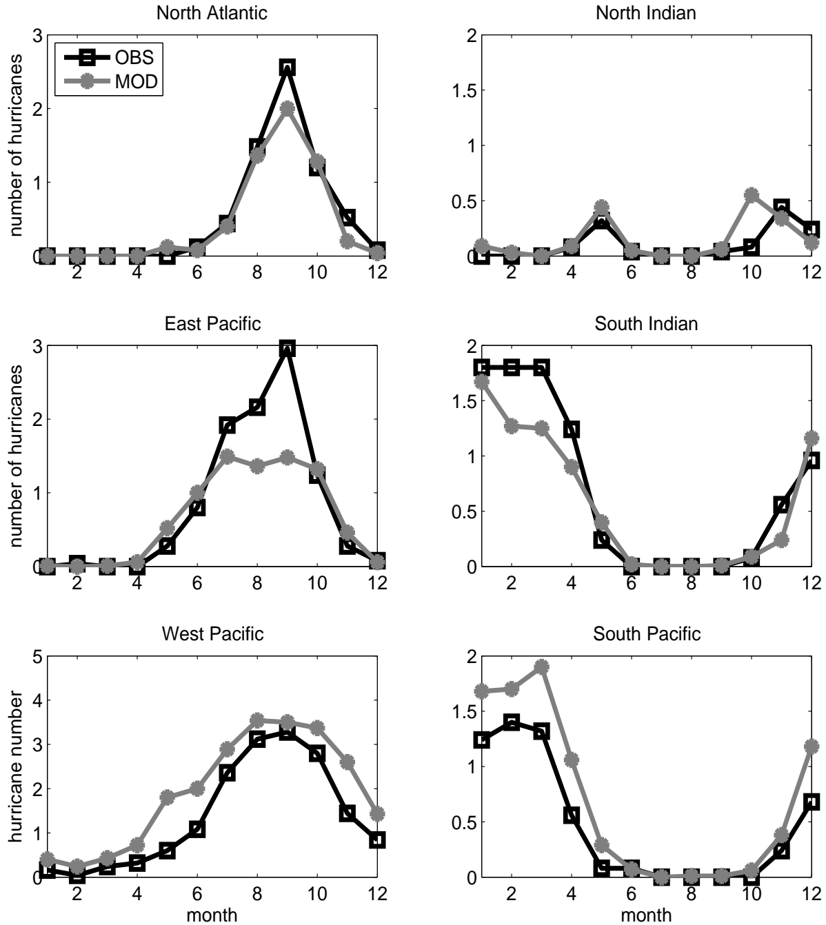
Figure 5. Observed and model simulated seasonal cycle (number of hurricanes per month) for each ocean basin from the 4-member ensemble mean (1=JAN, 12=DEC).
