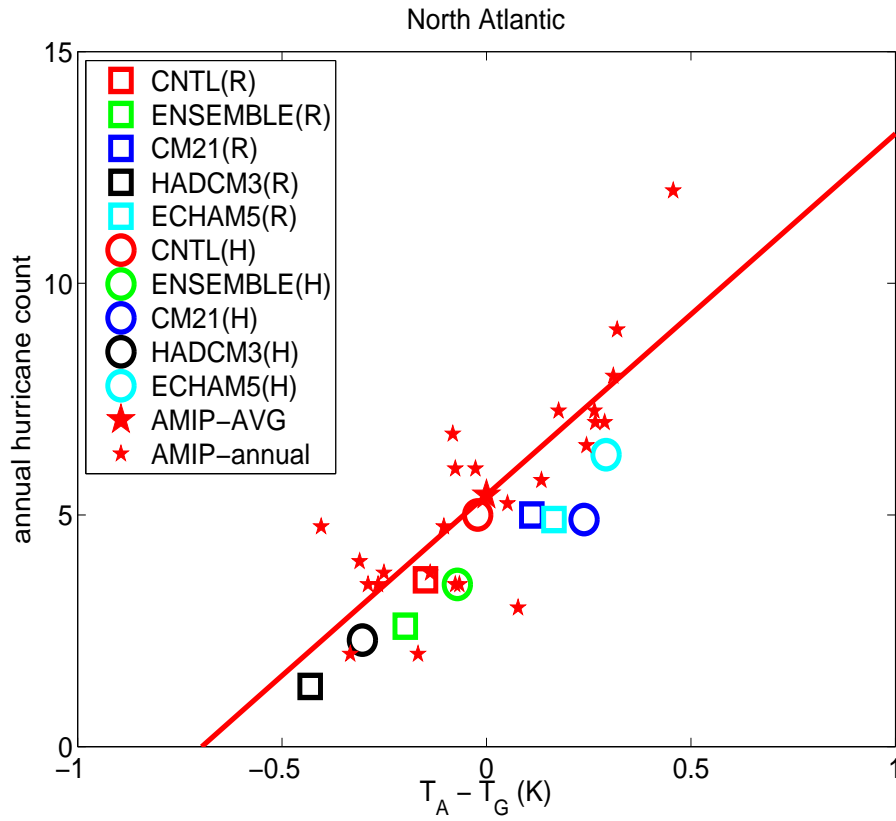
Figure 16. As in Fig. 15a except for scatter plot of annual Atlantic hurricane count versus ASO season Atlantic MDR SST ( T_A ) minus tropical mean SST ( T_G ); T_A - T_G is shown as anomalies from the climatological value obtained for the period of 1981-2005.
