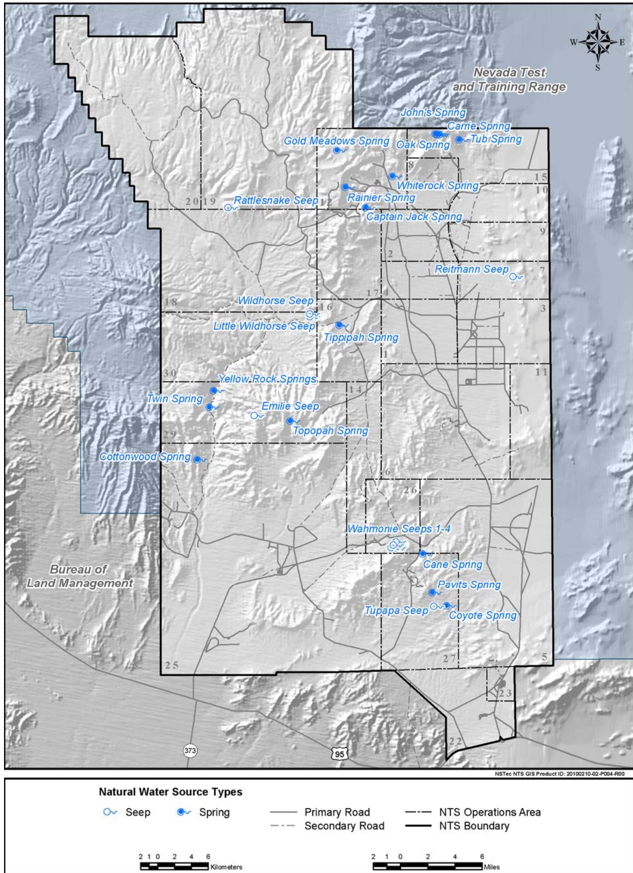
Figure A-4. Natural springs and seeps on the NTS (from Hansen et al., 1997; BN, 1999; Hansen et al., 2010)
