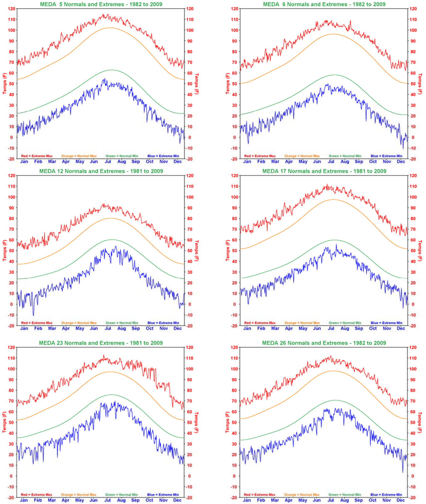
Figure A-13. Temperature extremes and normal maximums and minimums at six NTS MEDA stations (location of numbered stations are shown in Figure A-14)
