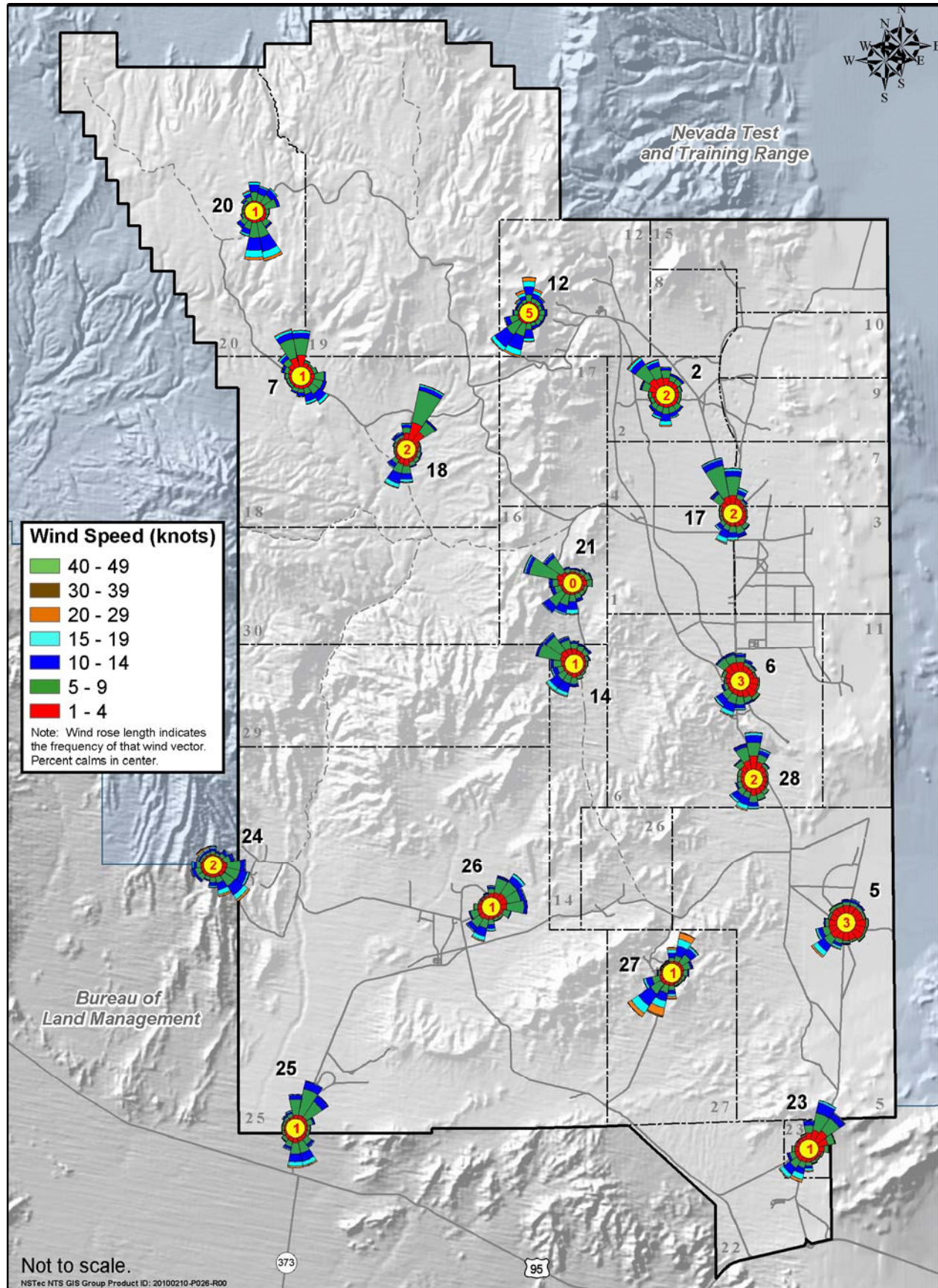
Figure A-14. Twenty-year wind rose climatology for the NTS (1989–2009)
