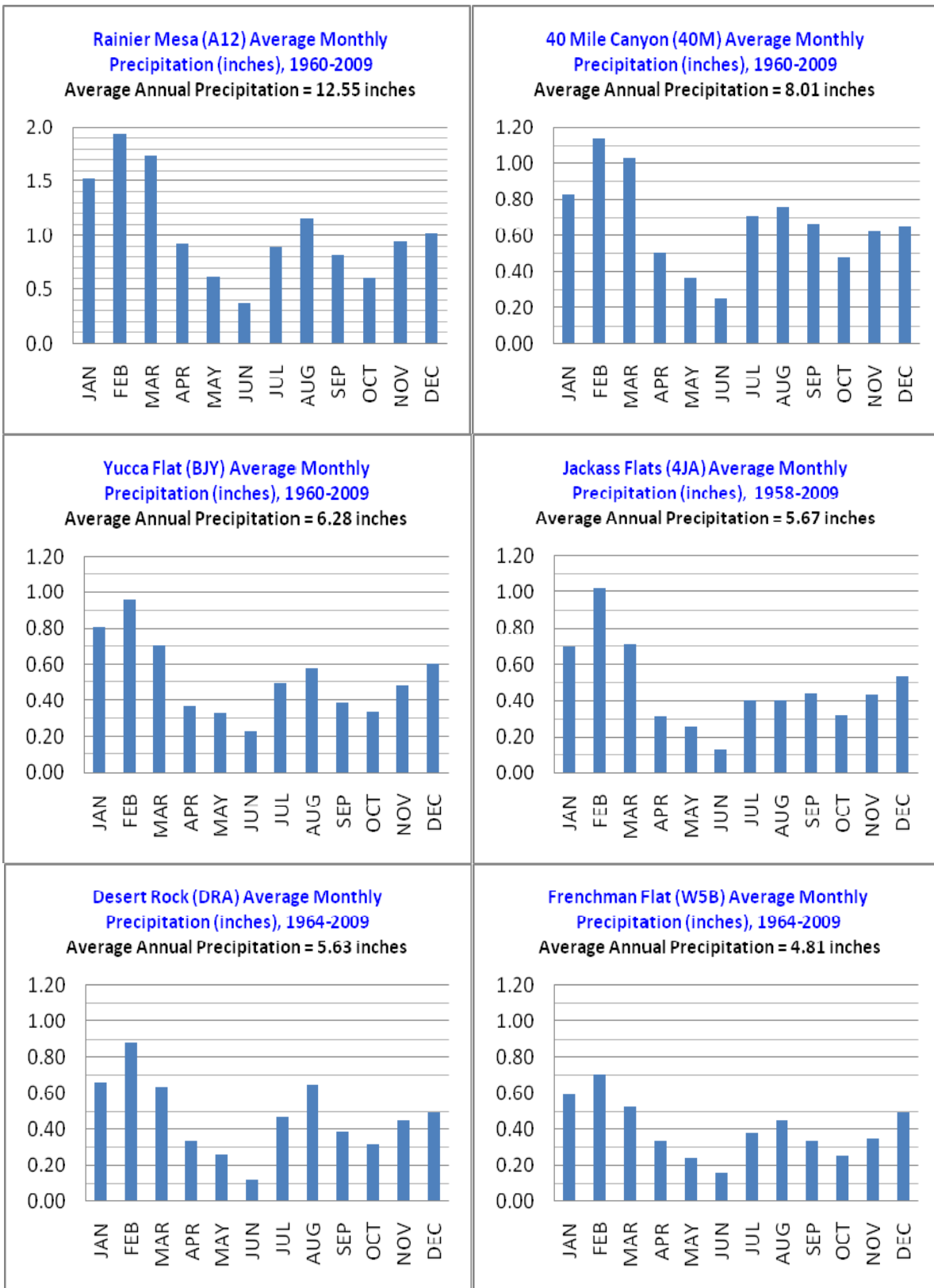
Figure A-12. Mean monthly precipitation at six NTS MEDA stations
