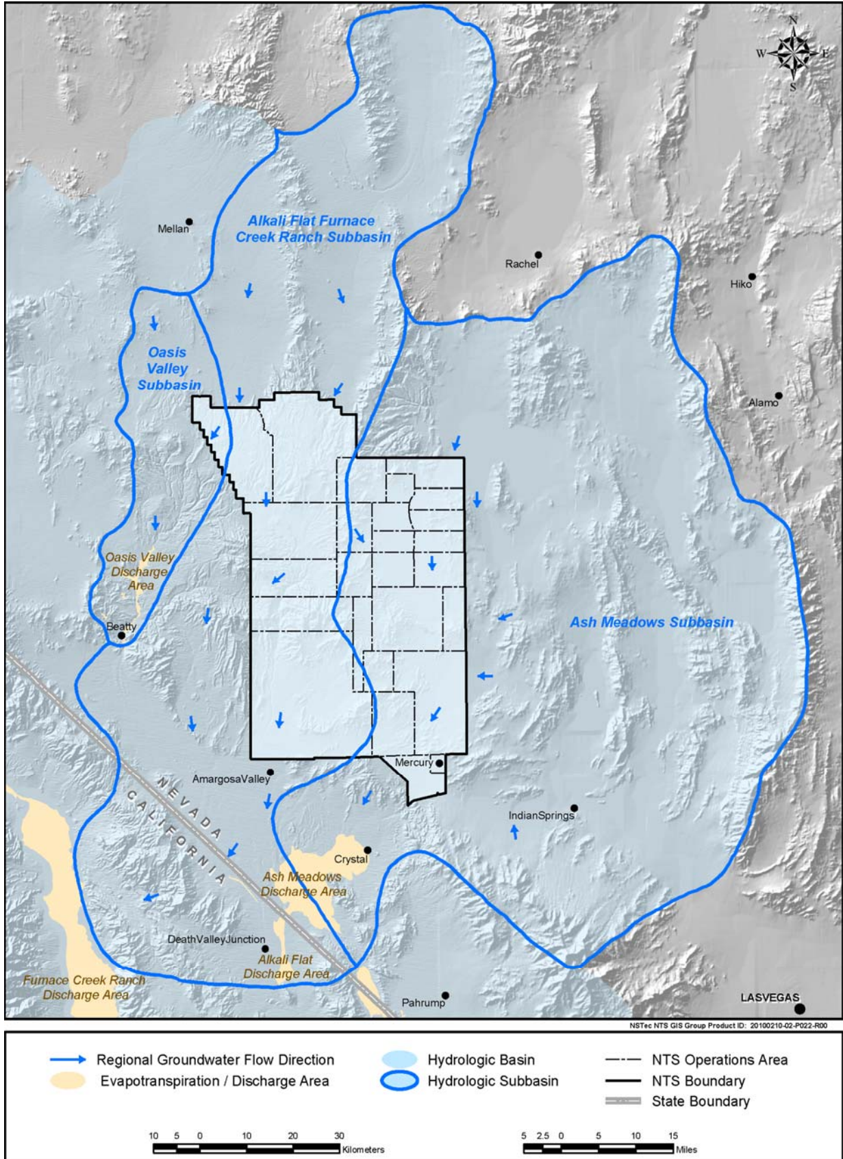
Figure A-5. Groundwater subbasins of the NTS and vicinity (modified from Waddell et al., 1984; Lacznik et al., 1996; and Lacznik et al., 2001)
