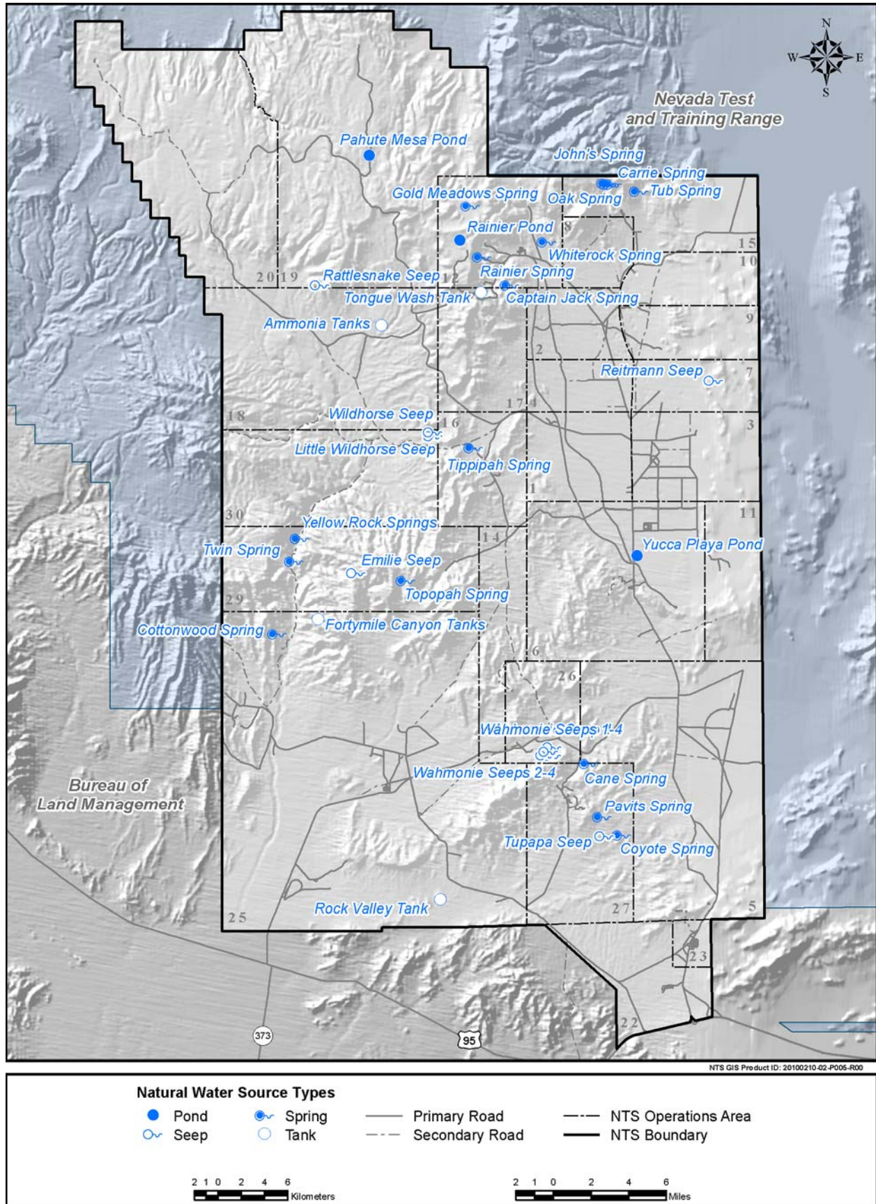
Figure A-17. Natural springs and seeps on the NTS (from Hansen et al., 1997; BN, 1999; Hansen et al., 2010)
