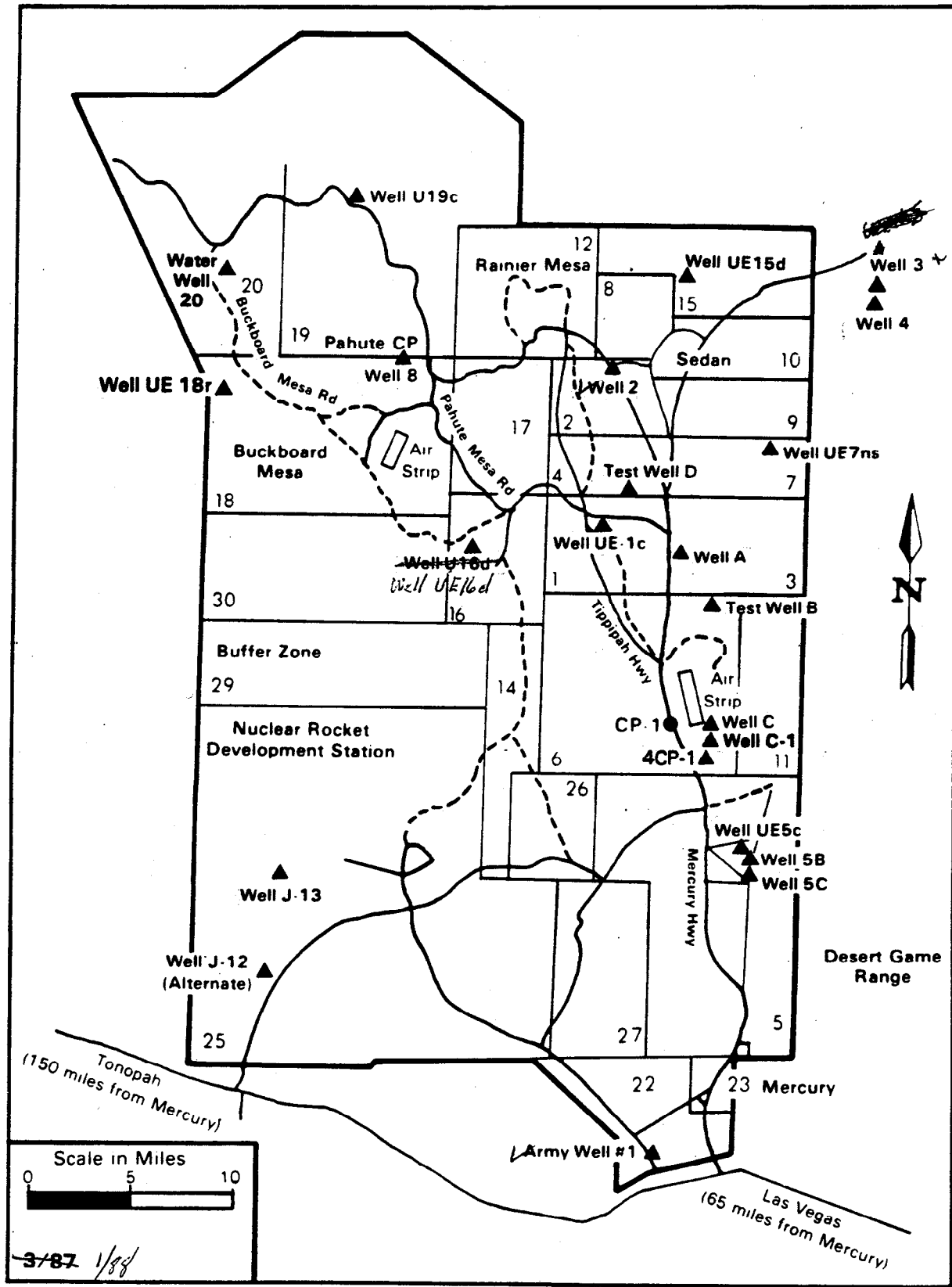
Figure 8. LTHMP sampling locations on the NTS.
