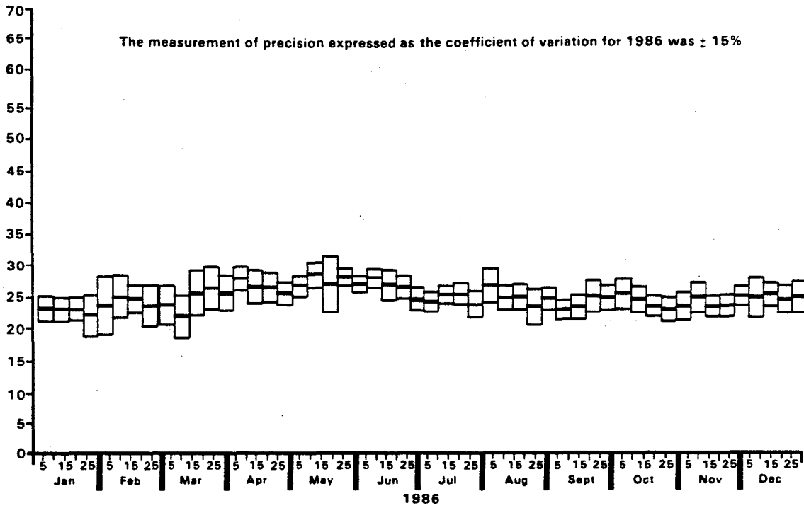
Figure 6. Weekly average krypton-85 concentration in air, 1986 data.
