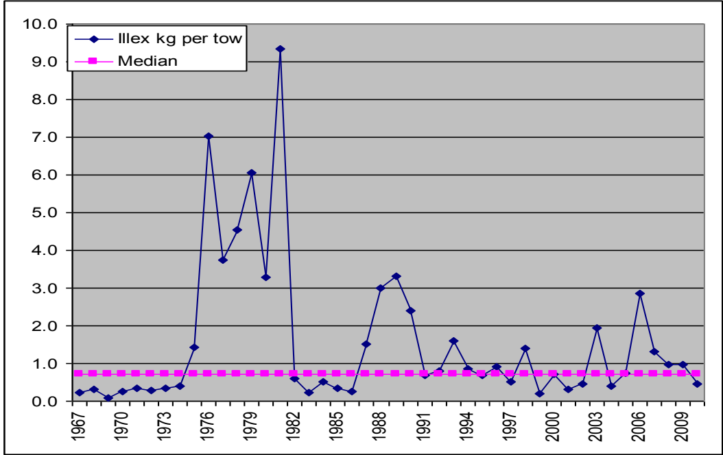
Figure 6. Fall NEFSC Trawl Survey - Illex Mean kg/tow.
