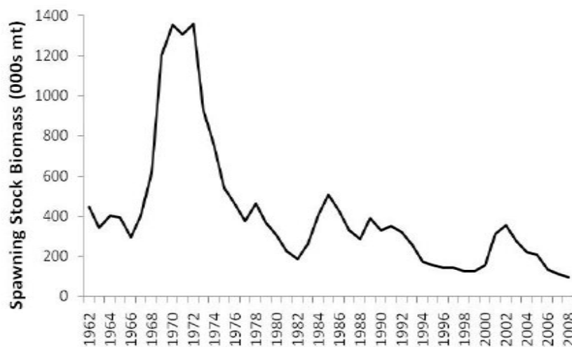
Figure 2. 2010 Mackerel TRAC SSB final model output.
