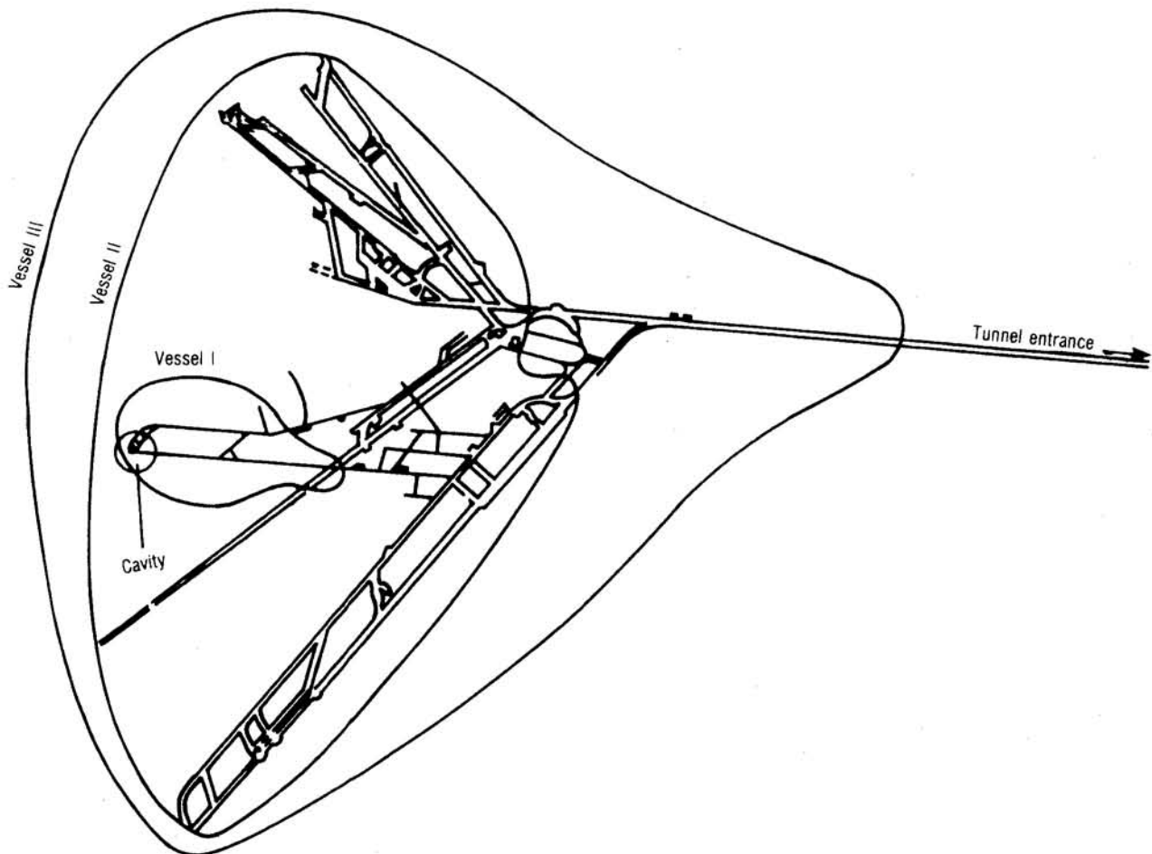
Figure 3-5—Three Redundant Containment Vessels (Plan View)
