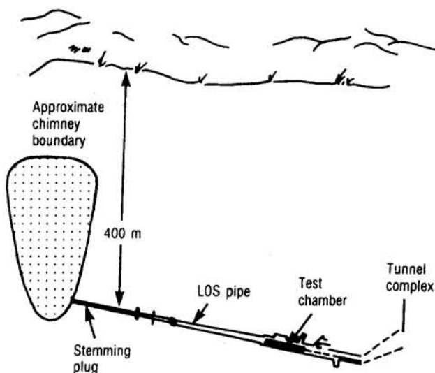
Figure 3-9—Typical Post-Shot Configuration
