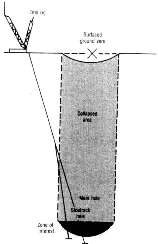
Figure 2-3—Drill-Back Operation
