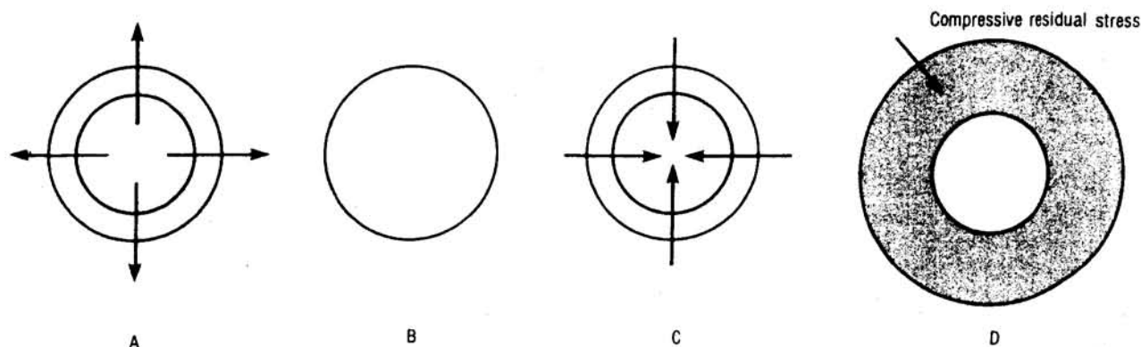
Figure 3-1—Formation of Stress "Containment Cage"
