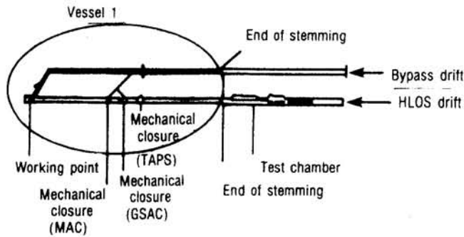
Figure 3-6—Vessel I
