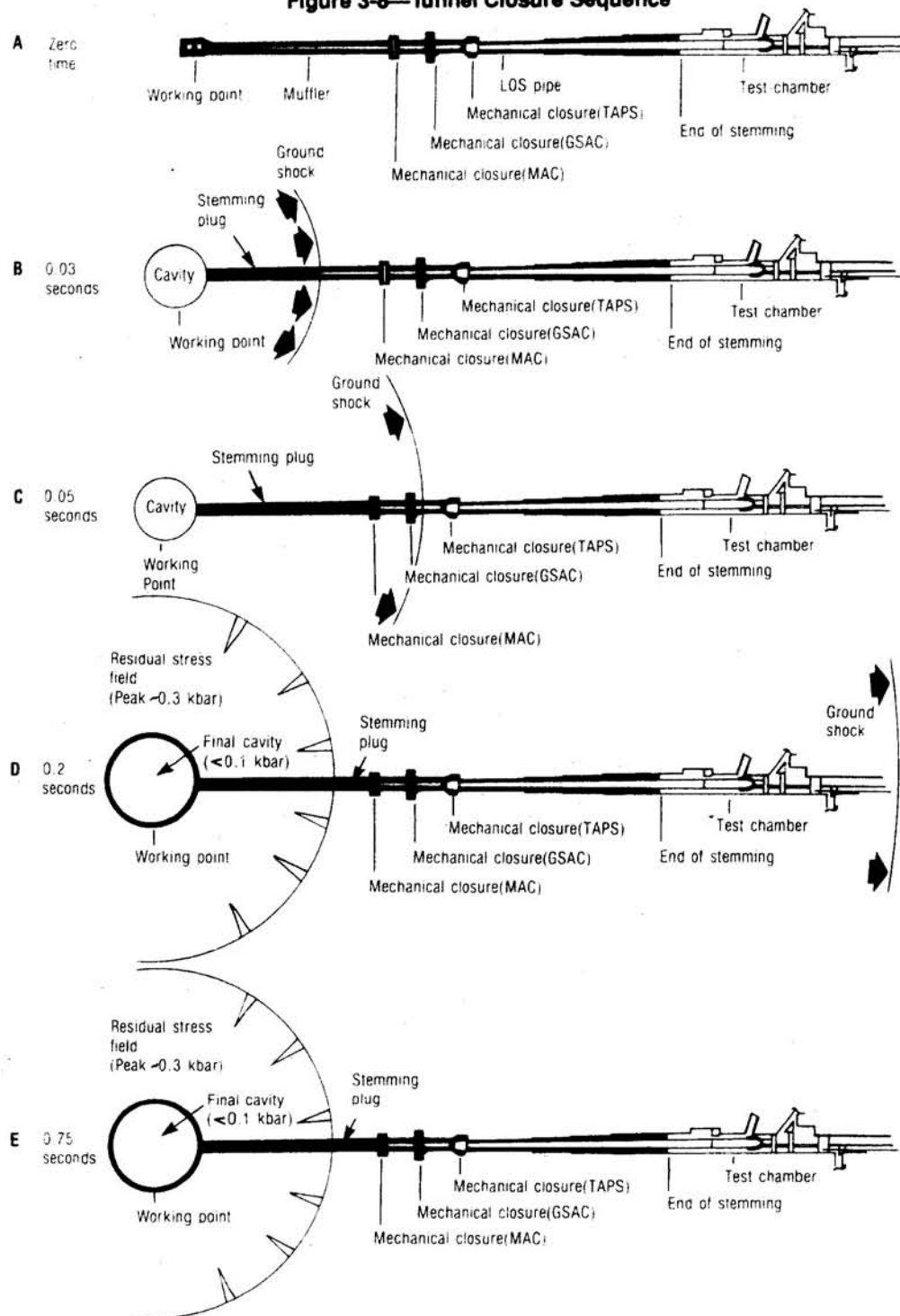
Figure 3-8—Tunnel Closure Sequence
