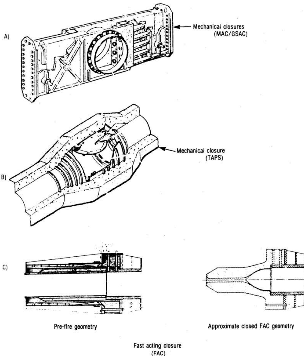
Figure 3-7—Vessel I Closures
