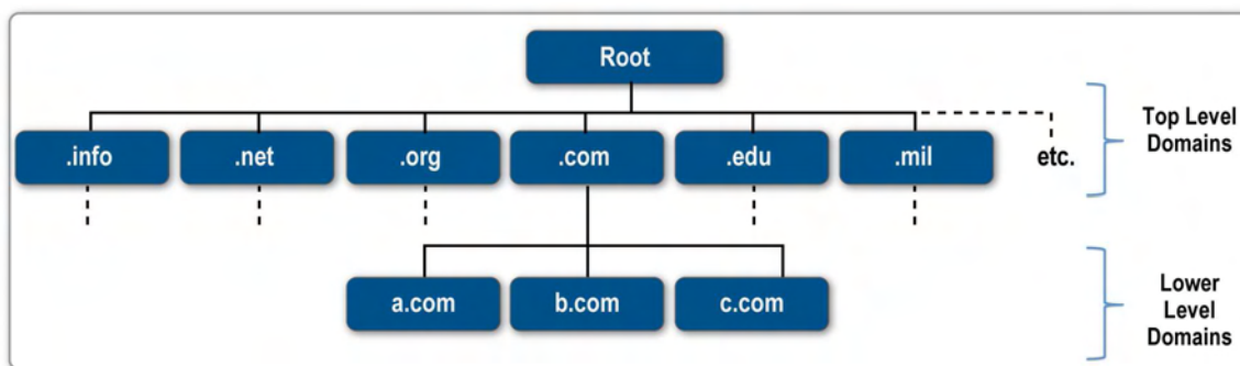
Figure 12: DNS Hierarchy
