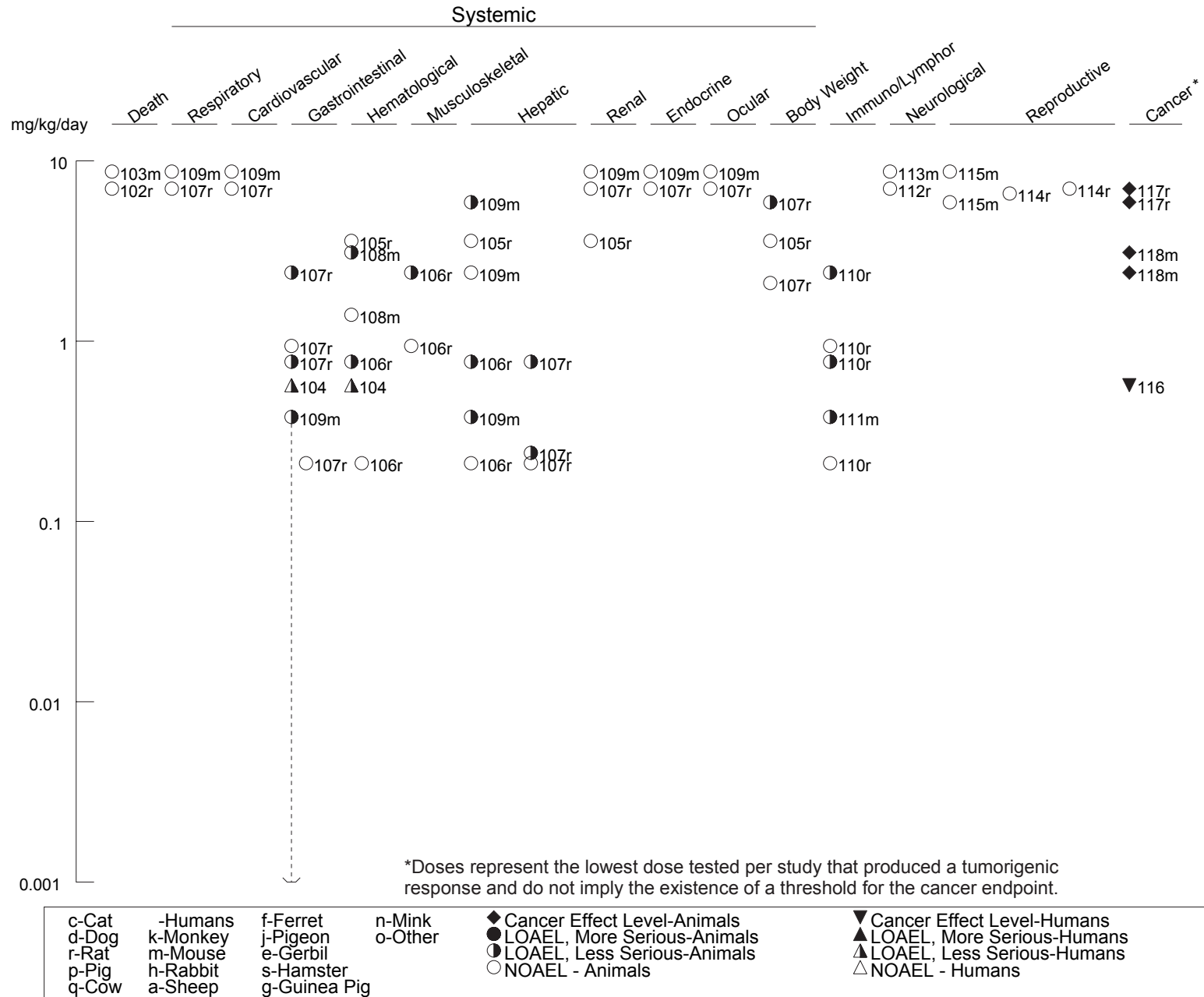
Figure 3-3 Levels of Significant Exposure to Chromium VI - Oral (Continued) Chronic (≥365 days)
