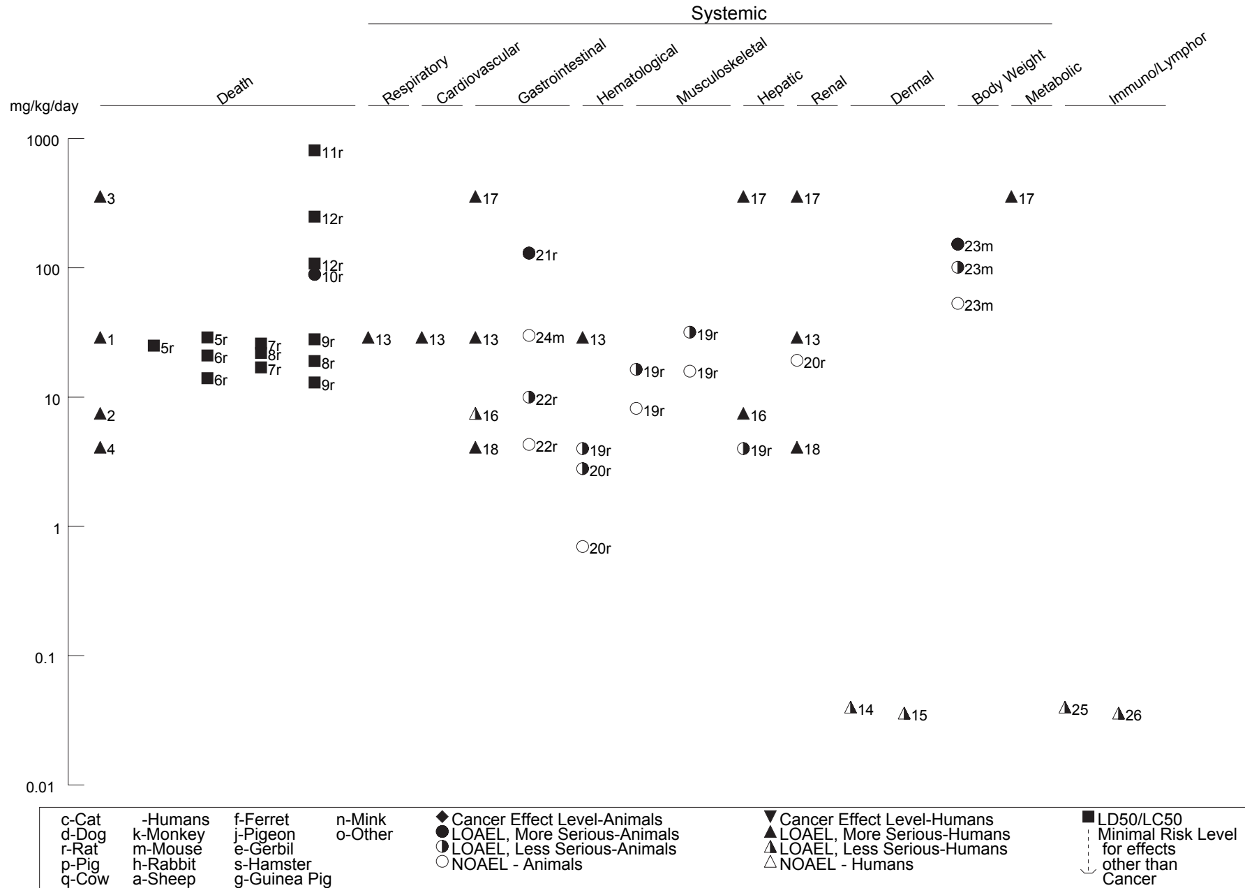
Figure 3-3 Levels of Significant Exposure to Chromium VI - Oral Acute (≤14 days)
