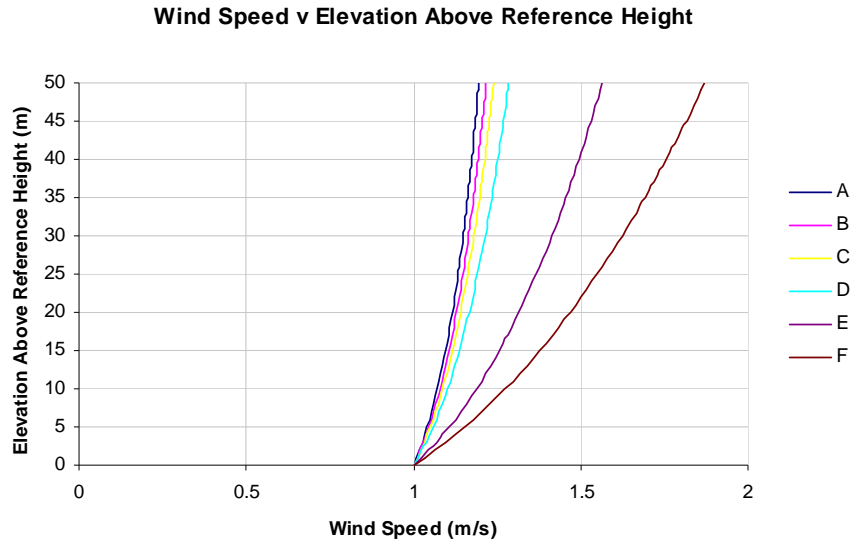
Figure 4-1 Wind Speeds for Elevation Above Reference Height
