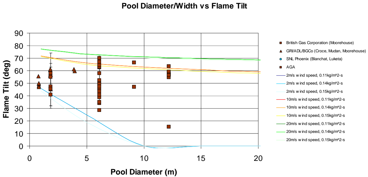
Figure 4-10 Flame Tilt for Pool Fires Compared to Experimental Data as a Function of Pool Fire Size
