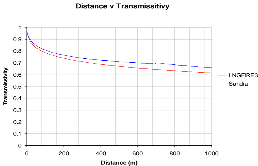
Figure 7-1 Transmissivity Predictions of LNGFIRE3 and SNL Recommendation
