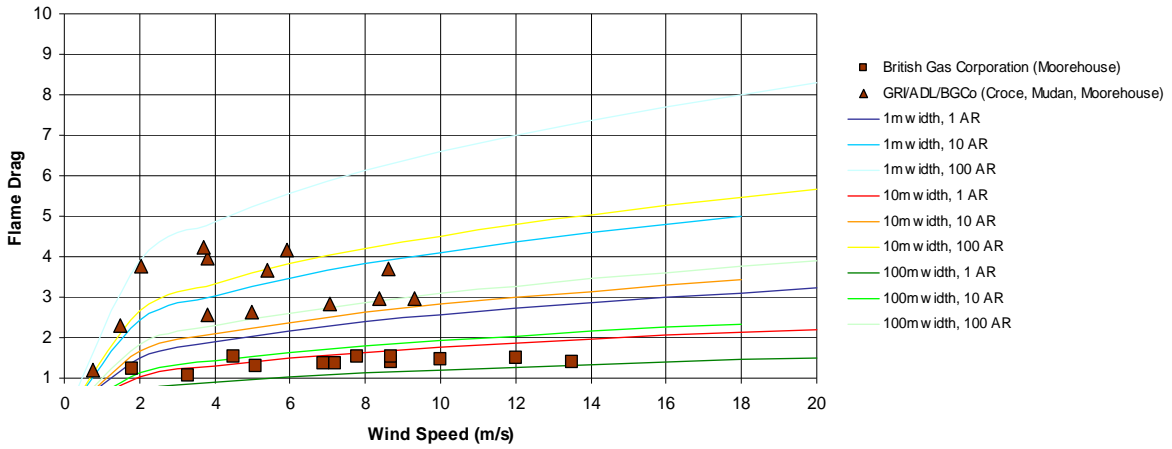
Figure 4-6 Flame Drag for Rectangular Pool Fires Predicted Compared to Experimental Data as a Function of Wind Speed
