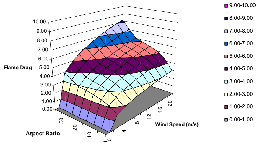
Aspect Ratio and Wind Speed vs Flame Drag
