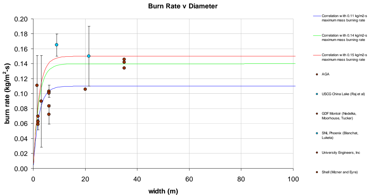
Figure 3-1 Circular Burn Rate Prediction Compared to Experimental Data
