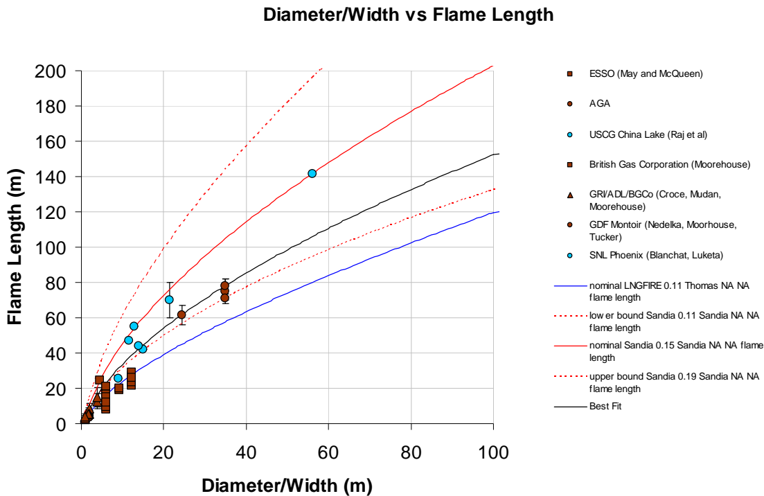
Figure 5-2 Flame Length Predictions and Uncertainties Compared to Experimental Data
