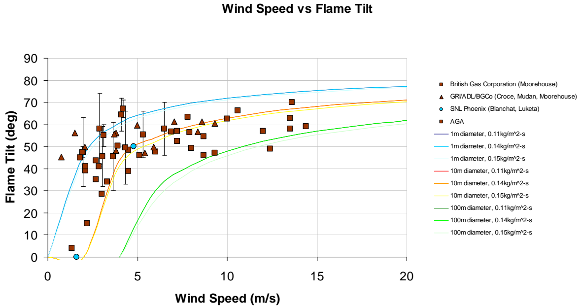
Figure 4-9 Flame Tilt for Pool Fires Compared to Experimental Data as a Function of Wind Speed
