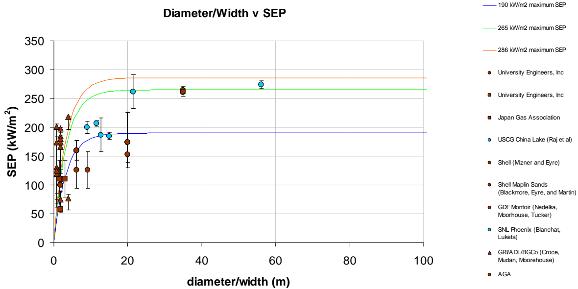
Figure 6-1 Surface Emissive Power Predicted Compared to Experimental Data as a Function of Pool Diameter and Width
