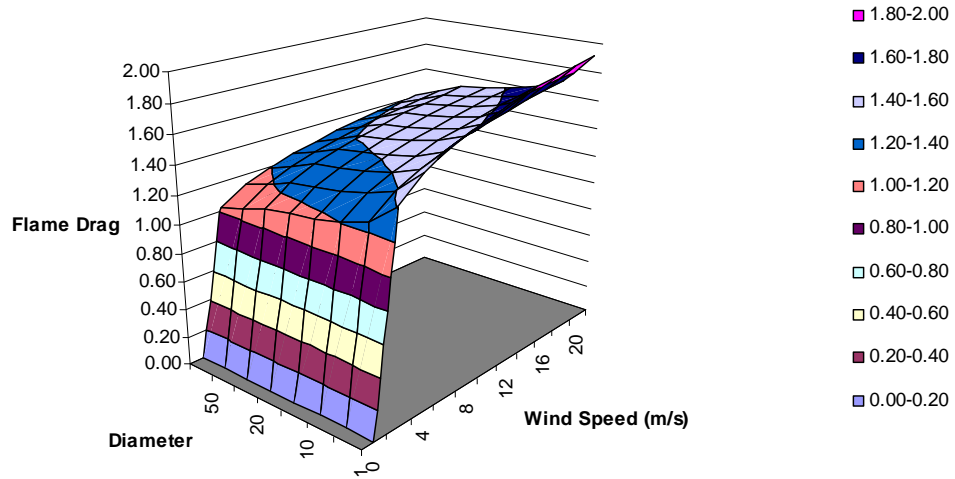
Diameter and Wind Speed vs Flame Drag
