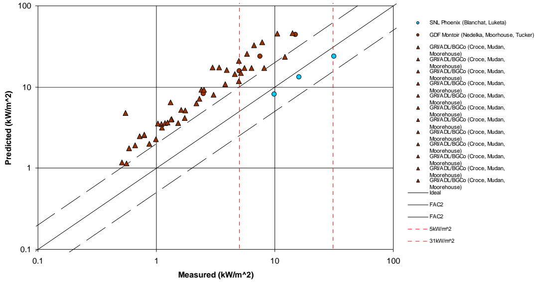
Figure 8-3: Mathcad Solid Flame Model using Montoir Values and SNL Correlations (0.14 kg/m 2 -s maximum mass burning rate, SNL Flame Length Correlation, 265 kW/m 2 maximum SEP, Wayne transmissivity)
