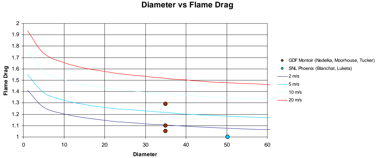
Figure 4-5 Flame Drag for Circular Pool Fires Predicted Compared to Experimental Data as a Function of Pool Diameter
