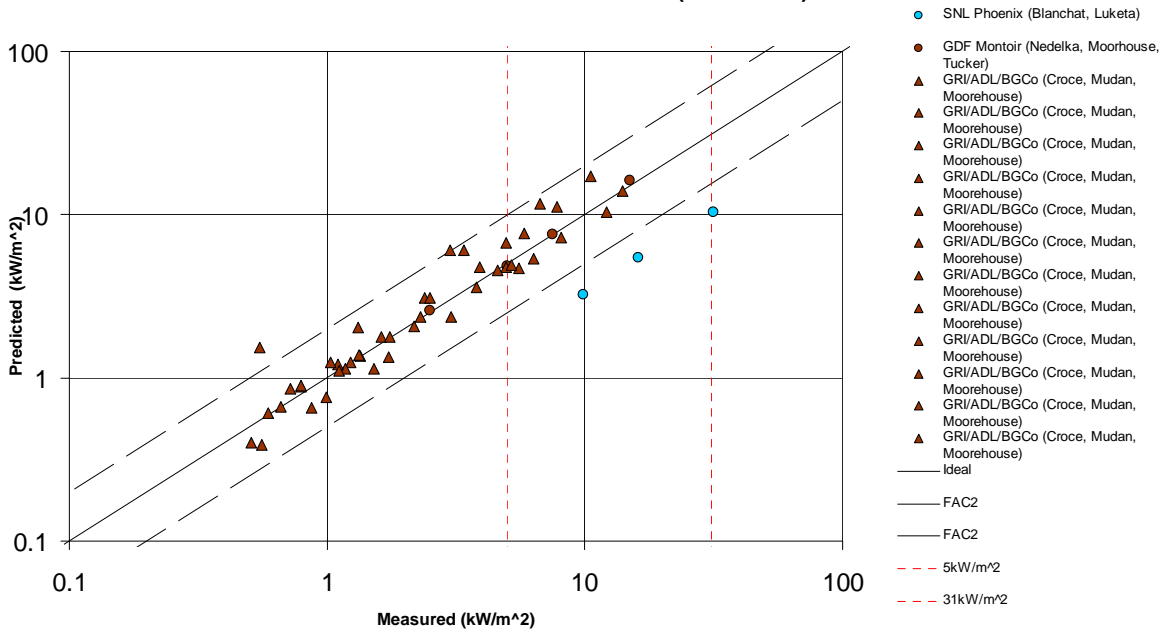
Figure 8-4: Mathcad Solid Flame Model using Best Fit Values and Correlations within SNL Range of Uncertainty (0.14 kg/m 2 -s maximum mass burning rate, Best Fit Flame Length Correlation, 125 kW/m 2 maximum SEP, Wayne transmissivity)
