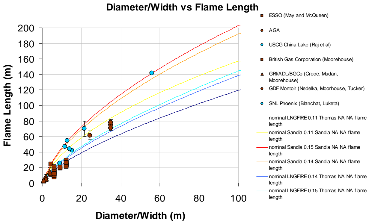
Figure 5-1 Flame Length Predictions Compared to Experimental Data
