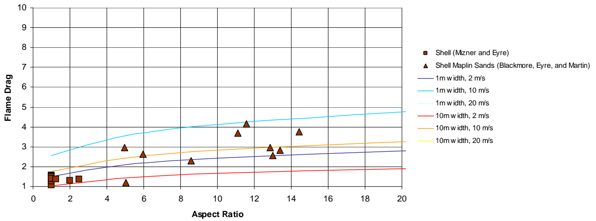
Figure 4-7 Flame Drag for Rectangular Pool Fires Predicted Compared to Experimental Data as a Function of Aspect Ratio
