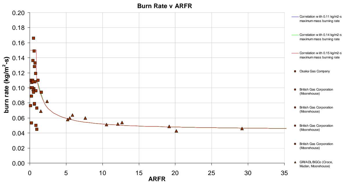
Figure 3-2 Rectangular Burn Rate Prediction Compared to Experimental Data
