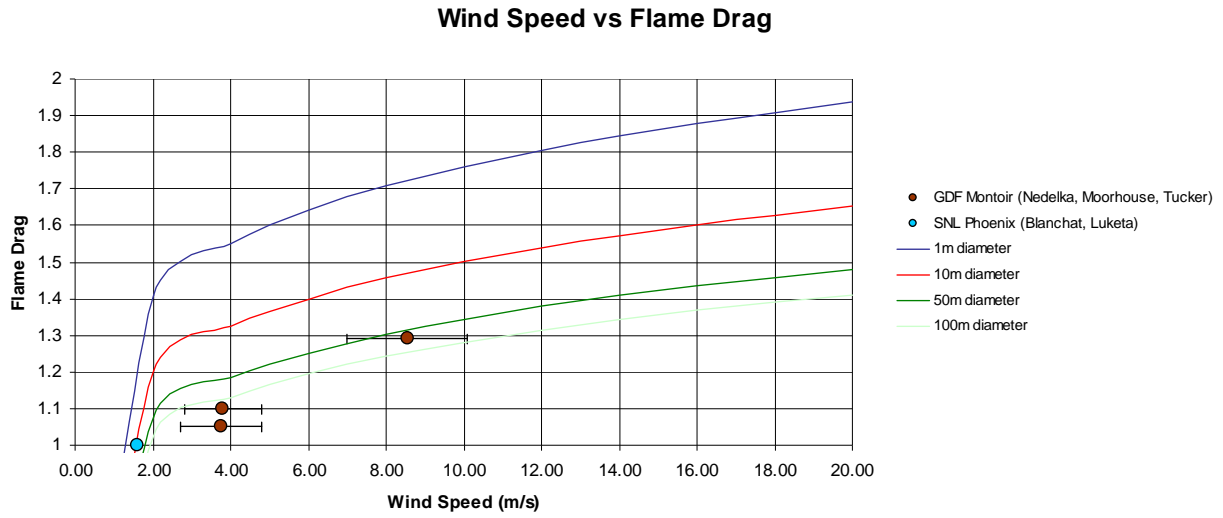
Figure 4-4 Flame Drag for Circular Pool Fires Predicted Compared to Experimental Data as a Function of Wind Speed
