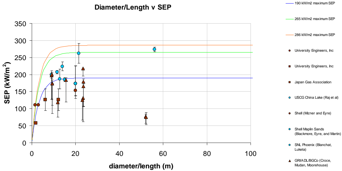
Figure 6-2 Surface Emissive Power Predicted Compared to Experimental Data as a Function of Pool Diameter and Length
