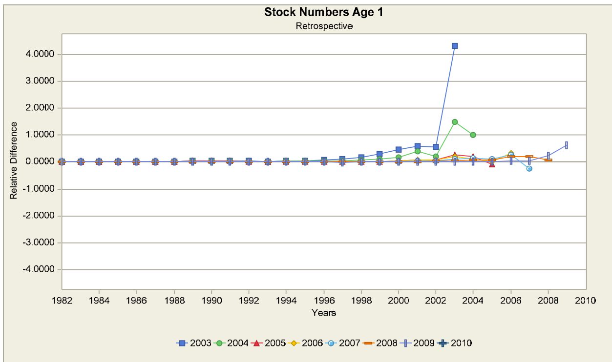
Figure A.146. ASAP BASE model retrospective patterns in Gulf of Maine Atlantic cod age 1 recruitment (000s) in absolute (top) and relative (bottom) terms.
