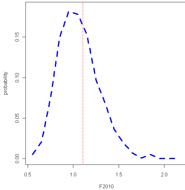
Figure A.142. Top: A 90% probability interval for Gulf of Maine Atlantic cod average fishing mortality from ages 5 to 7 ( F_{5-7} ) from the ASAP BASE model. The median value is in red, while the 5 th and 95 th percentiles are in dark grey. The point estimate from the base model (joint posterior modes) is shown in the thin green line with filled triangles. Bottom: MCMC distribution of average fishing mortality from ages 5 to 7 ( F_{5-7} ) in 2010, ASAP point estimate indicated by dashed red line.
