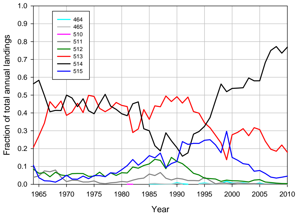
Figure A.19. Total (top) and fractional (as a fraction of the total, bottom) commercial landings of Gulf of Maine Atlantic cod by statistical area from 1964 to 2010.
