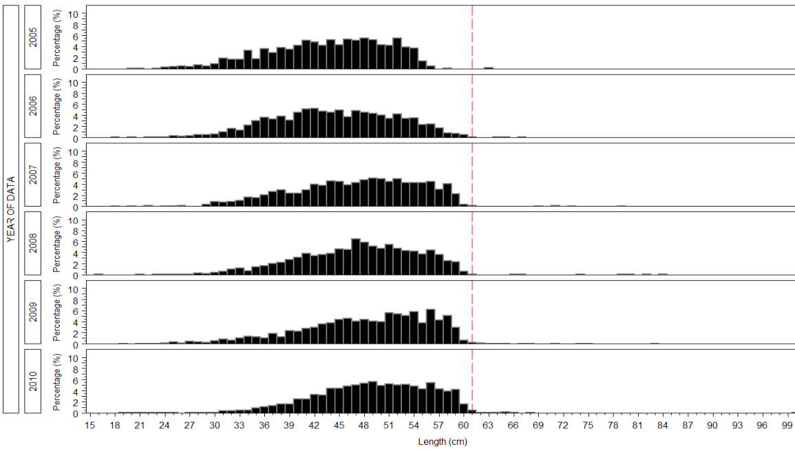
Figures A.59. Comparison of recreational discard length frequency distributions estimated using the survey filter approach (top) to those generated from the B2 sampling of the I9 catch (bottom) between 2005 and 2010 for Gulf of Maine Atlantic cod. The dashed red line represents the recreational minimum retention size of 24 inches (61.0 cm) from May 1, 2006-2010. The minimum retention size from January 1, 2005 to May 1, 2006 was 23 inches (58.4cm).
