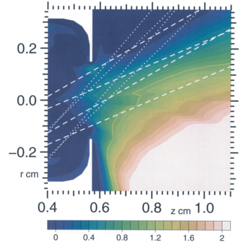
FIG. 14: Schematic of crossing beams in hohlraums at the NIF and flow Mach number for the component of the flow velocity parallel to the beat wavenumber of the crossing laser beams. The outer beams are dotted, the inner dashed.
