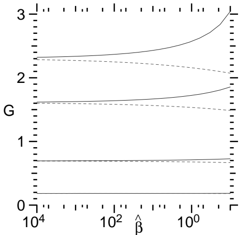
FIG. 4: Total gain G \equiv w|_{\infty}^{\infty} as a function of \hat{\beta} \equiv (1/2)(\gamma_{01}/\nu)^2(\eta\omega_s/\nu)^4|a_1(0)|^2 for linear amplifications \exp(2\pi\Lambda) = 1.2, 2, 5, 10 . Solid (dashed) curves are the (anti-)autoresonant cases.
