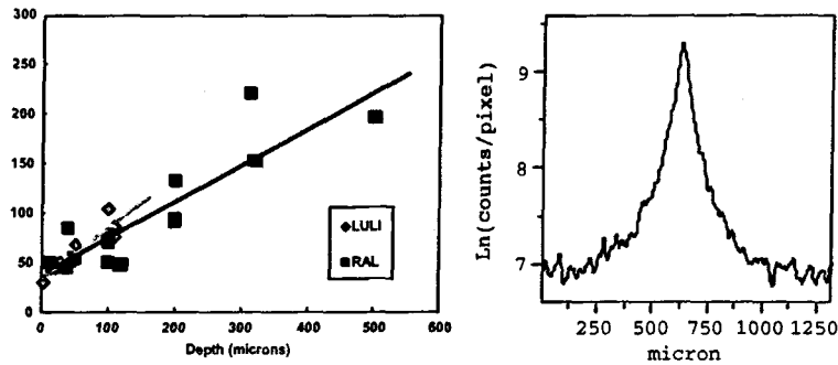
FIG. 1. Left, K\alpha image radius as a function of Al thickness, Cu K\alpha at RAL, (squares) and Ti K\alpha at LULI, (diamonds). Linear fits defining the minimum radius and cone angle are also shown. Right a typical line out showing the natural logarithm of the recorded counts per pixel in a Cu K\alpha image.
