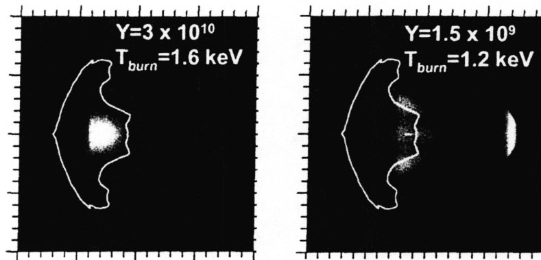
FIG. 8. Radiation /hydro- dynamic modeling of compression and simplified modeling of short pulse heating of a conceptual FI proof of principle target at NIF. The simulations show neutron images. Y is the yield and T_{burn} is the peak temperature. Left assumes parallel transport. Right assumes a 40^\circ cone. Pictures span approx. 200 \mu\text{m} . Tip of cone is at right edge of pictures.
