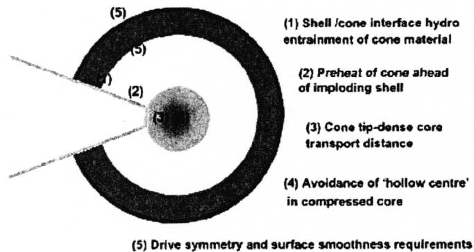
FIG. 6. The cone target concept for fast ignition, with identification of the main physics issues in the hydrodynamics.
