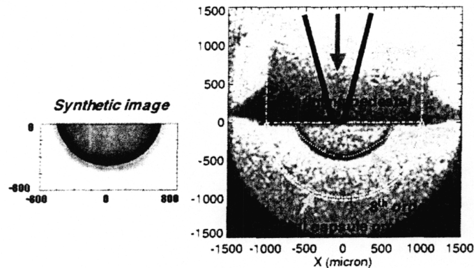
FIG. 7. An initial FI target hydro experiment at Z showing implosion of a hemisphere diagnosed by laser radiography, with an indication of how it could be adapted for cone guided ignition (right) and a numerical simulation of the same implosion (left)
