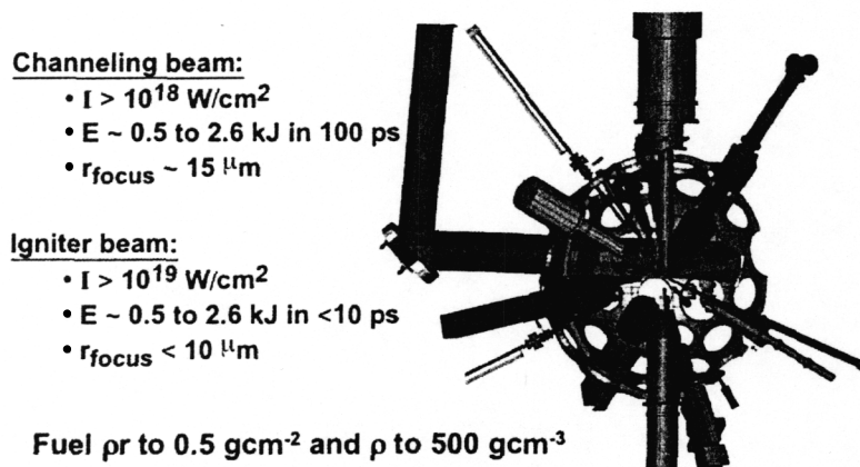
FIG. 9. Omega target chamber with HEPW adaptation. HEPW beam shown in purple.
