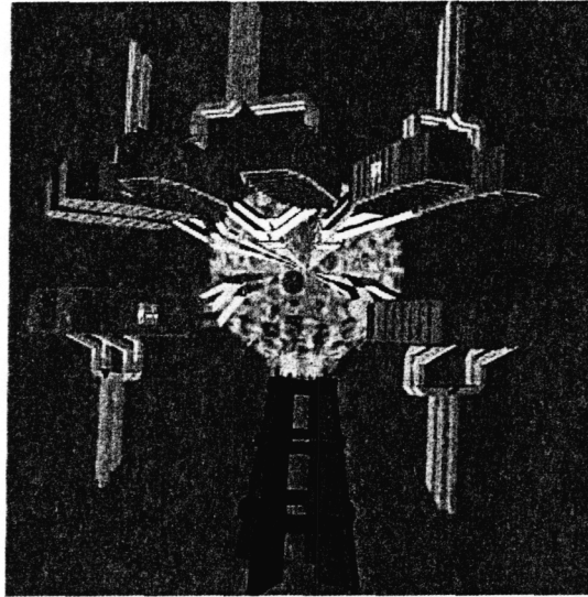
FIG. 10. Engineering concept for adapting NIF for full scale fast ignition. HEPW beamlines with grating compressors are shown. Long pulse beamlines are omitted.
