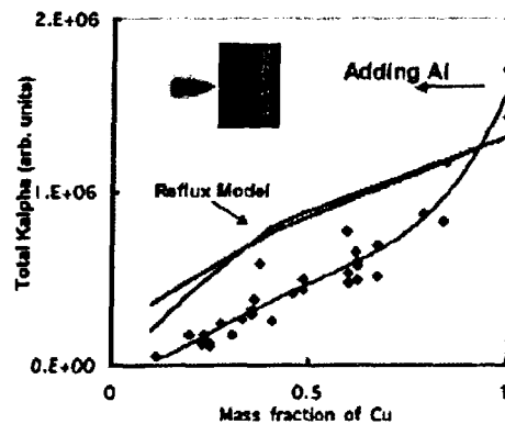
FIG. 2. MonteCarlo model of the integrated fluorescence in refluxing electron transport and measured data.
