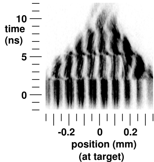
FIG. 5: The 6.79 \mu\text{m}/\text{ns}/\text{fringe} VISAR image from shot 29040809 is typical high quality VISAR data. Horizontal is both position on the target and phase; vertical is time. The discontinuities at 2 ns and 5.3 ns are shock breakout and coalescence, respectively. Increasing curvature of the shock front as it propagates causes the triangular envelope of the fringes.
