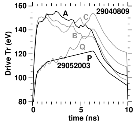
FIG. 8: The three upper curves are the X-ray drives corresponding to the three simulations of shot 29040809 plotted in Fig. 7; the two lower curves correspond to the two simulations of shot 29052003. The dark curves match the VISAR shock overtake times best. The overtake time and combined shock strength are sensitive to details of the drive shape.
