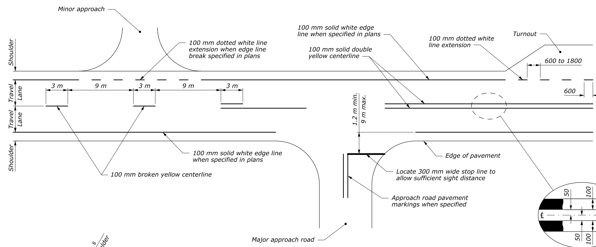
CENTERLINE DETAIL
