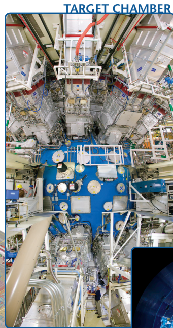
NIF's massive target chamber 192 laser beams enter through the square openings.
