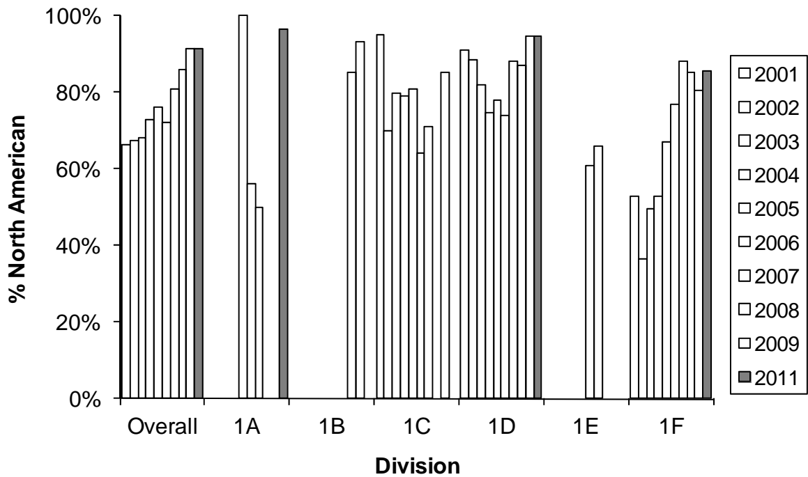
Figure 3. The non-weighted proportion of North American origin Atlantic salmon ( Salmo salar ) caught at West Greenland from 2001 – 2011 (left to right, 2011 is represented by the grey filled columns) by NAFO division according to the sample data. Division 1B 2011 data were not available and will be updated in 2012. Division 1A 2005 value is based off of one sample.
