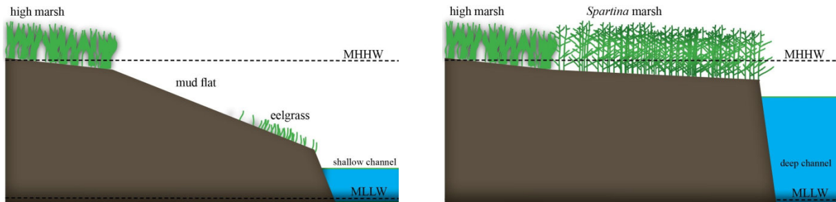
Figure 4. Spartina invasion of mudflats results in sediment accretion, an increase in elevation, and alteration of estuarine hydrology.
