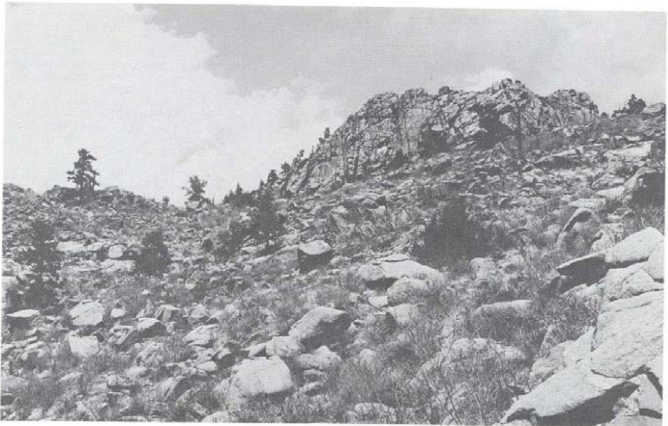
Figure 8.—Area of Haploborolls-Rock outcrop complex, steep.
