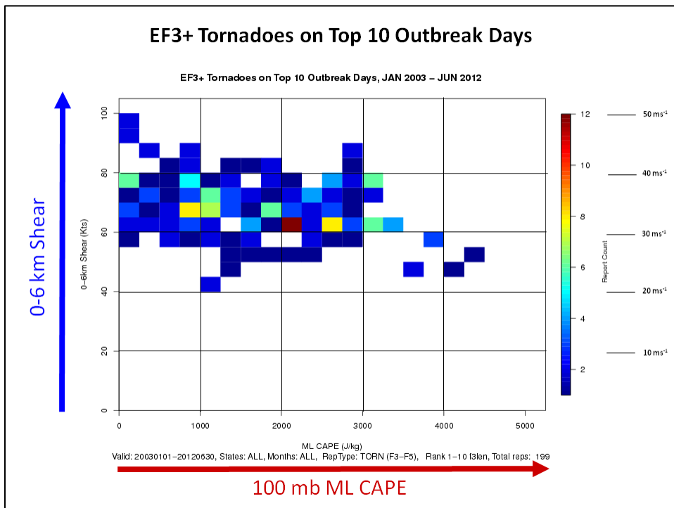
Fig. 14. Plot of F3+/EF3+ tornadoes from the top 10 outbreak days, binned by MLCAP/SHR6.
