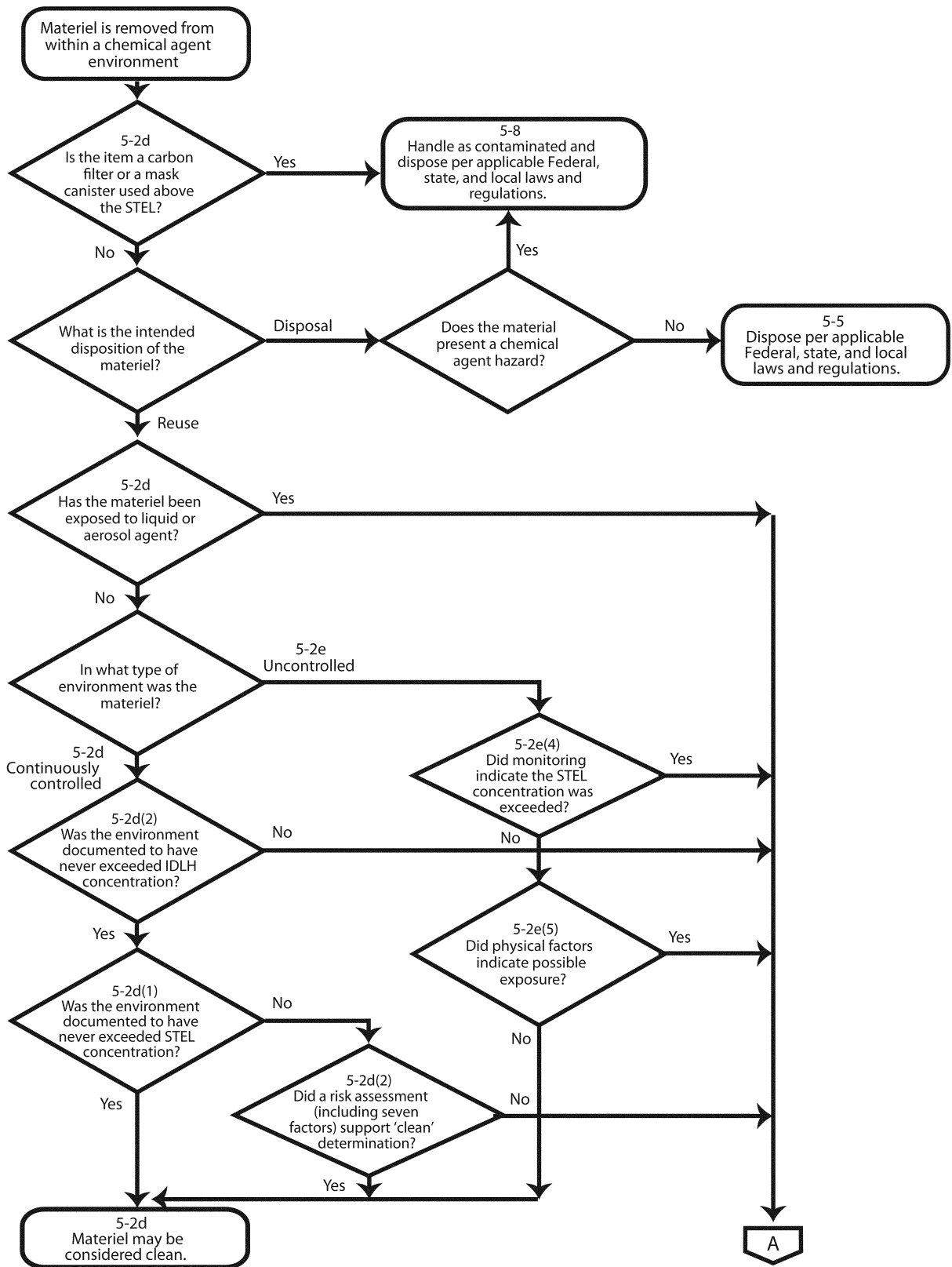
Figure D-1. Decontamination flow diagram
