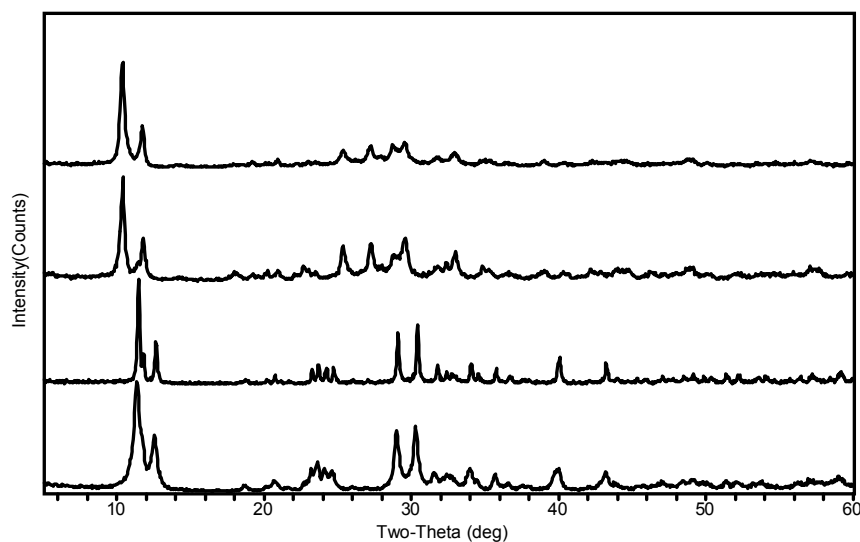
Figure 1. a) SOMS framework, \text{Na}_2\text{Nb}_{2-x}\text{M}^{\text{IV}}_x\text{O}_{6-x}(\text{OH})_x \cdot \text{H}_2\text{O} ; small balls = O, medium balls = Nb/Ti, large balls = Na, occluded waters and Na(1) are not shown, for clarity, but are located in the pores; b) Powder XRD data for the as-synthesized and Sr-exchanged samples; peak shifts due to changes in unit cell size from ion exchanged cation size. 12b
