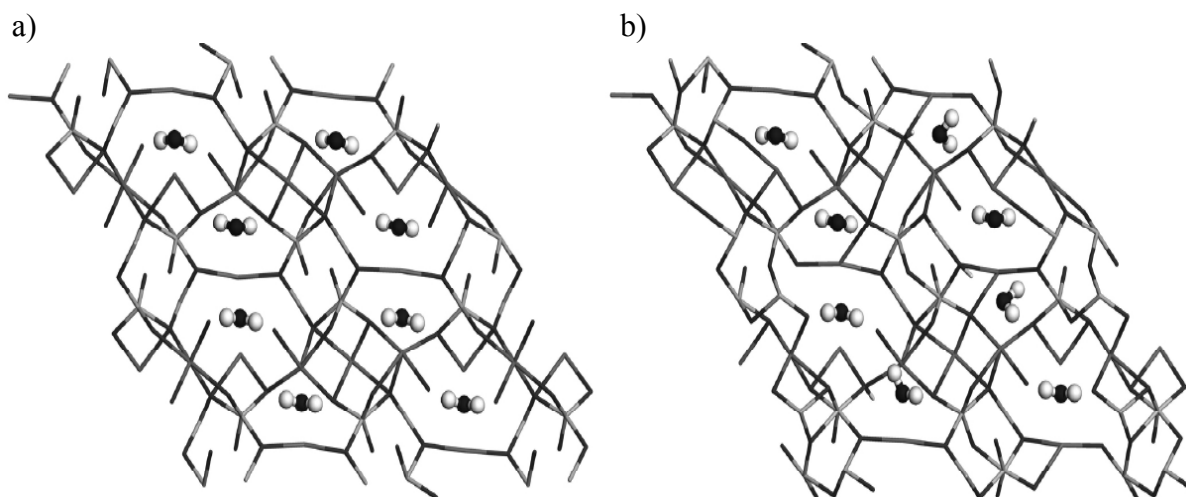
Figure 6. DFT optimized SOMS unit cell. The framework atoms are shown in wireframe and the water are depicted as ball-and-stick models. (a) 0% Ti; (b) 18.75% Ti.
