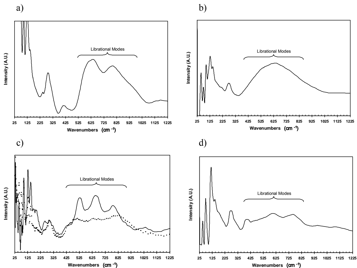
Figure 3. INS data collected at 10K for: a) SOMS end member, ice-like peak at \approx 550\text{ cm}^{-1} ; b) Sr-exchanged SOMS end member, librational modes at \approx 450\text{ cm}^{-1} ; c) 20%Ti SOMS, librational modes of water at 533, 654 and 785\text{ cm}^{-1} (decreased intensity data dotted line is ^2\text{H} sample); d) Sr-exchanged 20%Ti SOMS, librational modes at 503, 604 and 759\text{ cm}^{-1} .
