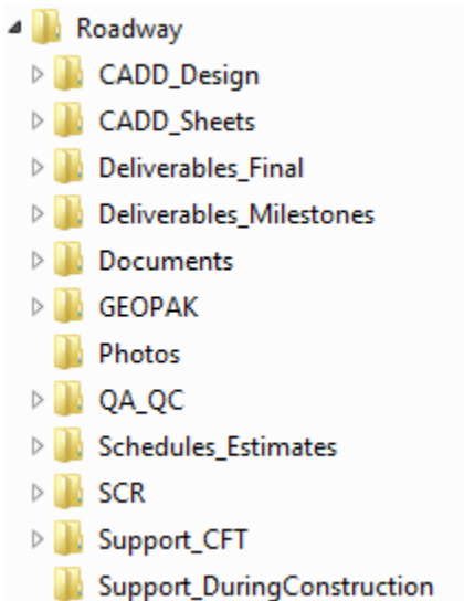
Figure 2-2: Roadway Directory
