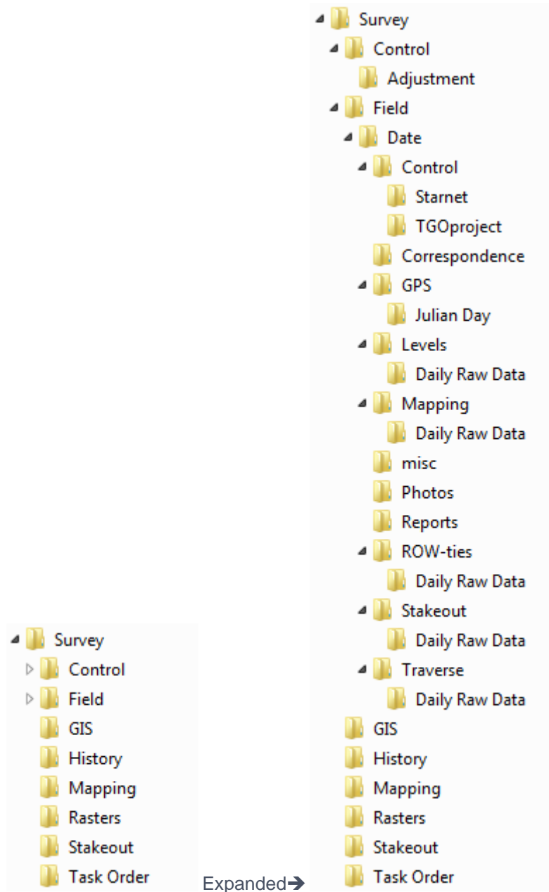
Figure 2-6: Survey Directory
