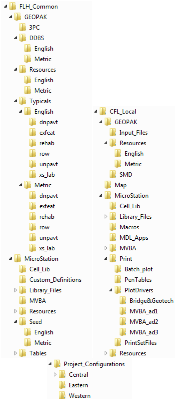
Figure 2-10: CADD Resource Files
