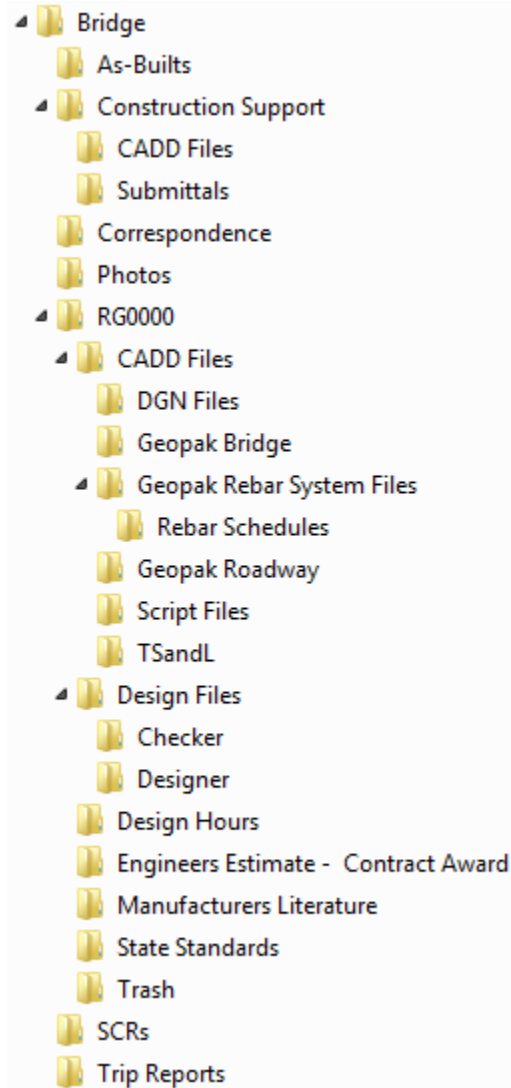
Figure 2-8: Bridge Directory
