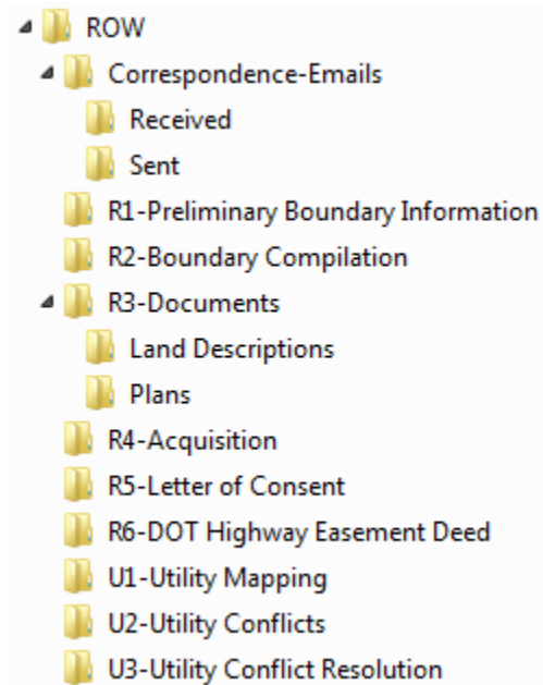
Figure 2-4: ROW Directory
