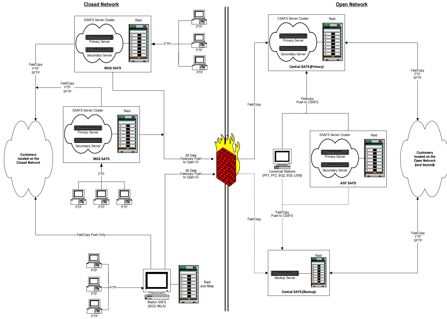
Figure 12-3. SAFS Architecture
