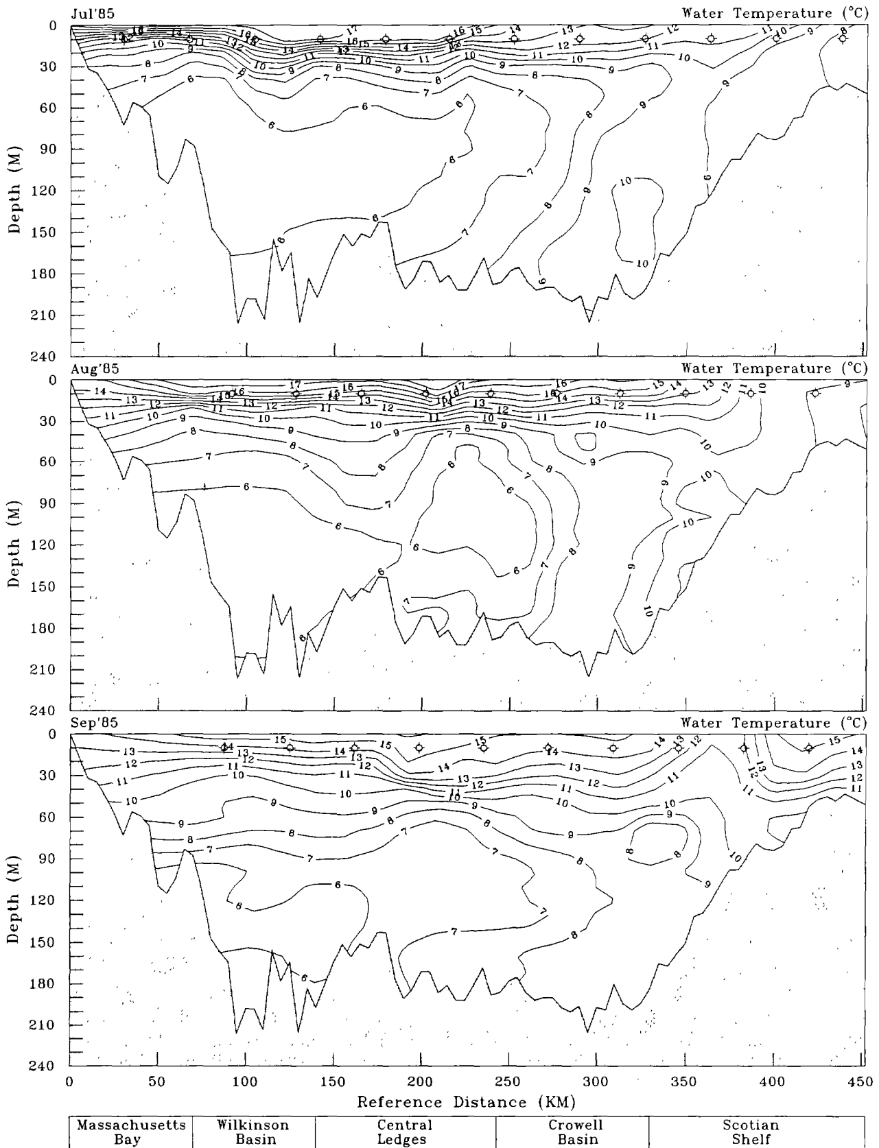
Figure 122. Water-column thermal structure (degrees Celsius) and CPR station locations at the 10-m depth (x) along the Gulf of Maine transect during July, August, and September 1985.
