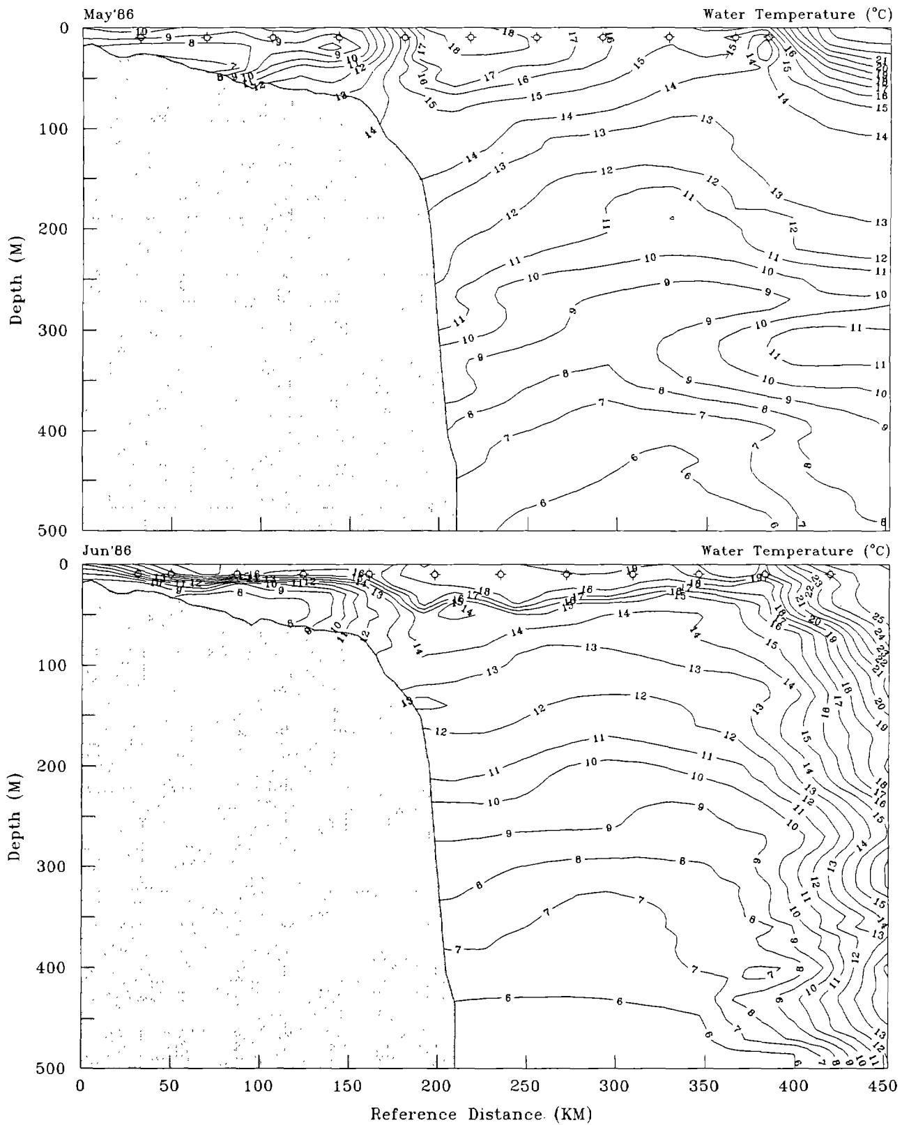
Figure 52. Water-column thermal structure (degrees Celsius) and CPR station locations at the 10-m depth (⊗) along the Middle Atlantic Bight transect during May and June 1986.
