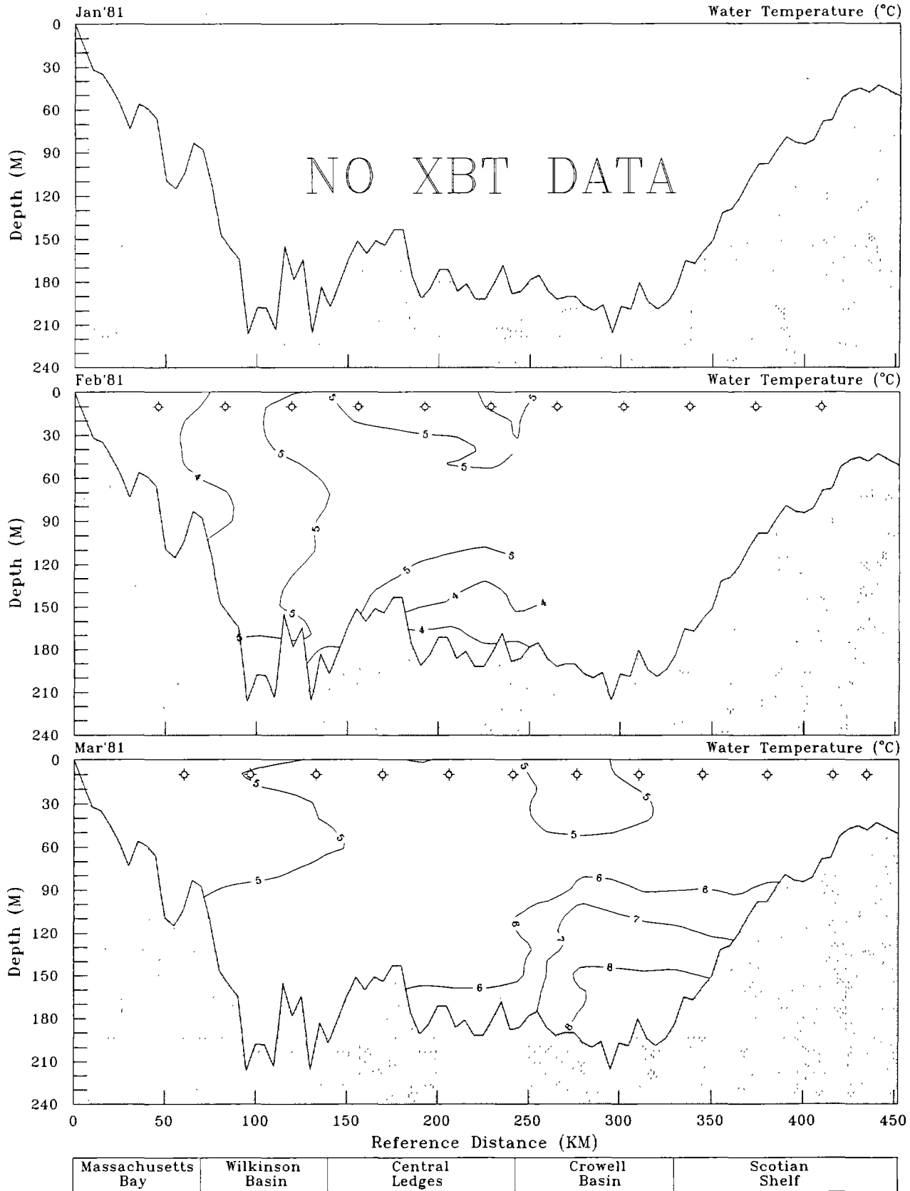
Figure 104. Water-column thermal structure (degrees Celsius) and CPR station locations at the 10-m depth (□) along the Gulf of Maine transect during January, February, and March 1981.
