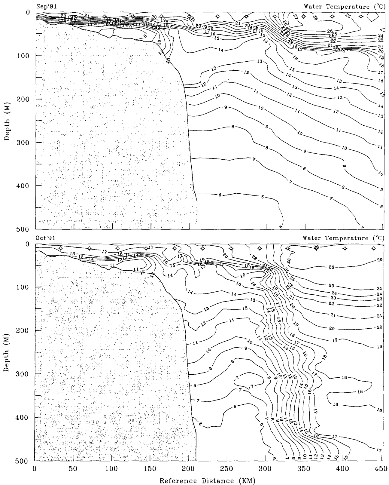
Figure 84. Water-column thermal structure (degrees Celsius) and CPR station locations at the 10-m depth (■) along the Middle Atlantic Bight transect during September and October 1991.
