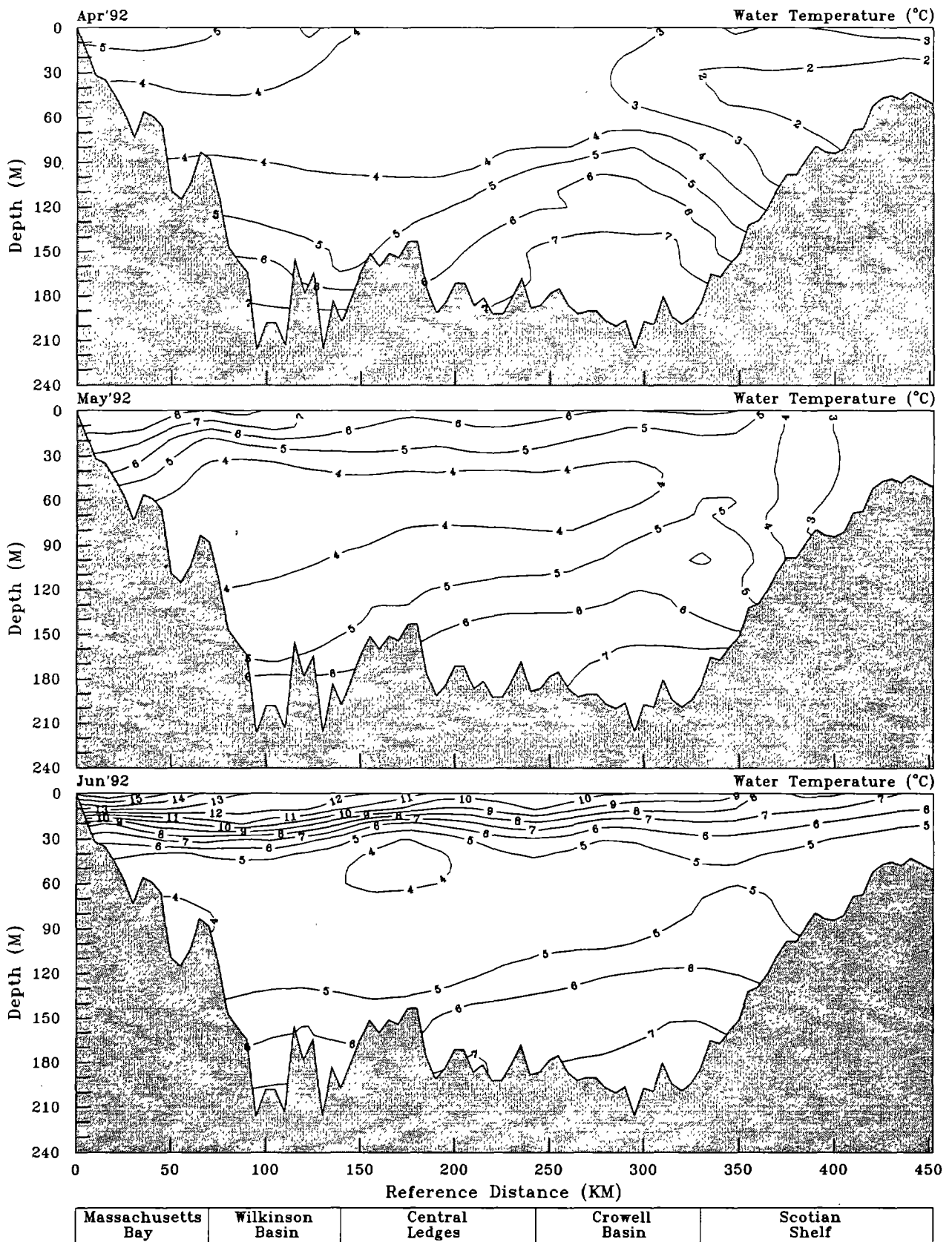
Figure 145. Water-column thermal structure (degrees Celsius) and CPR station locations at the 10-m depth (■) along the Gulf of Maine transect during April, May, and June 1992.
