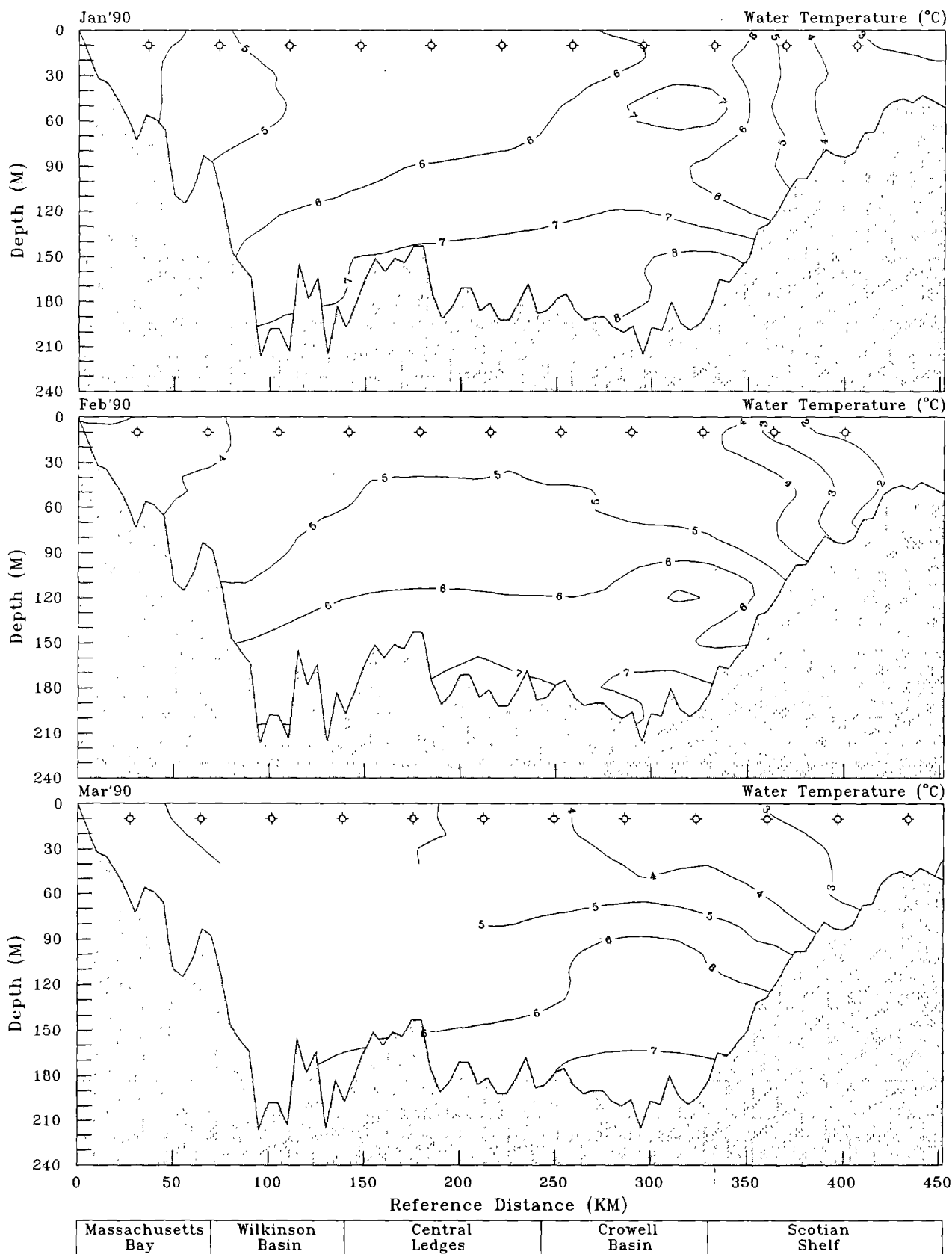
Figure 136. Water-column thermal structure (degrees Celsius) and CPR station locations at the 10-m depth (◻) along the Gulf of Maine transect during January, February, and March 1990.
