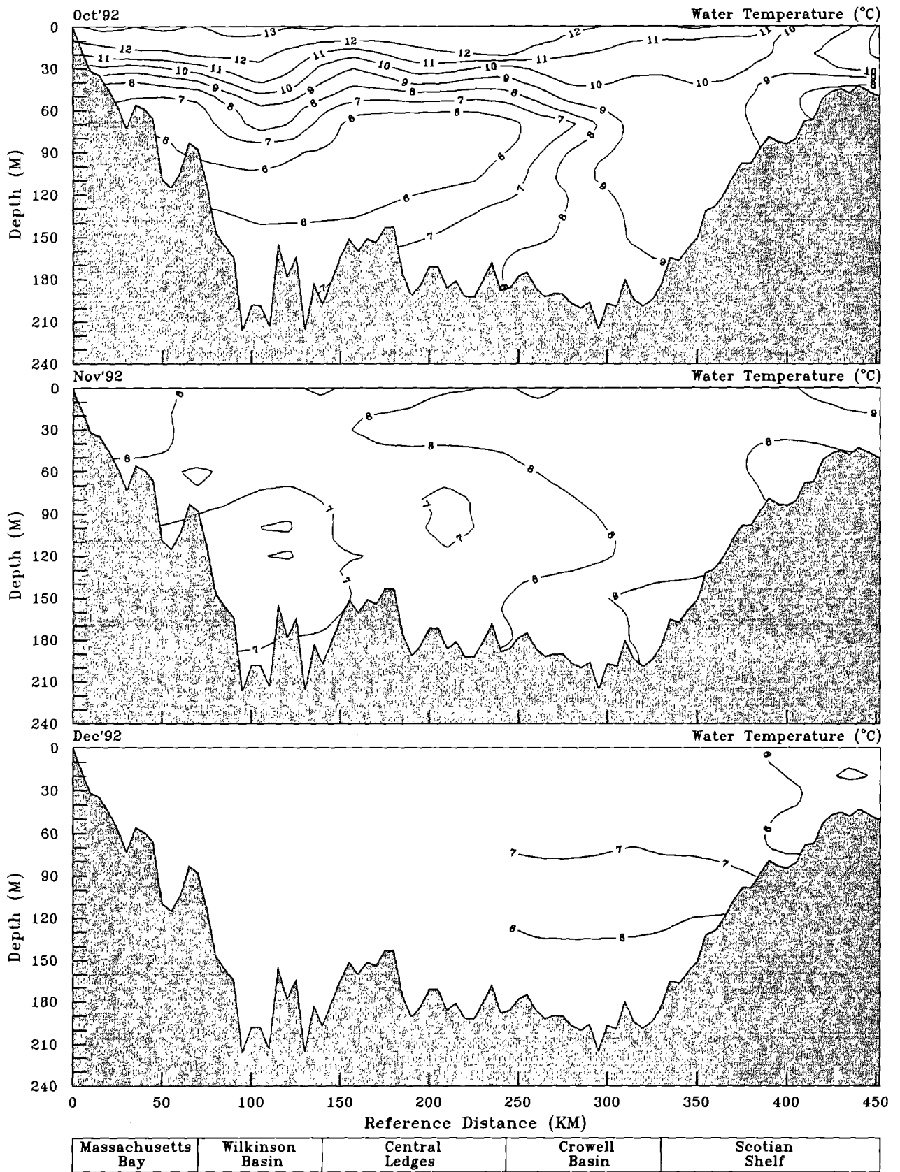
Figure 147. Water-column thermal structure (degrees Celsius) and CPR station locations at the 10-m depth (⊕) along the Gulf of Maine transect during October, November, and December 1992.
