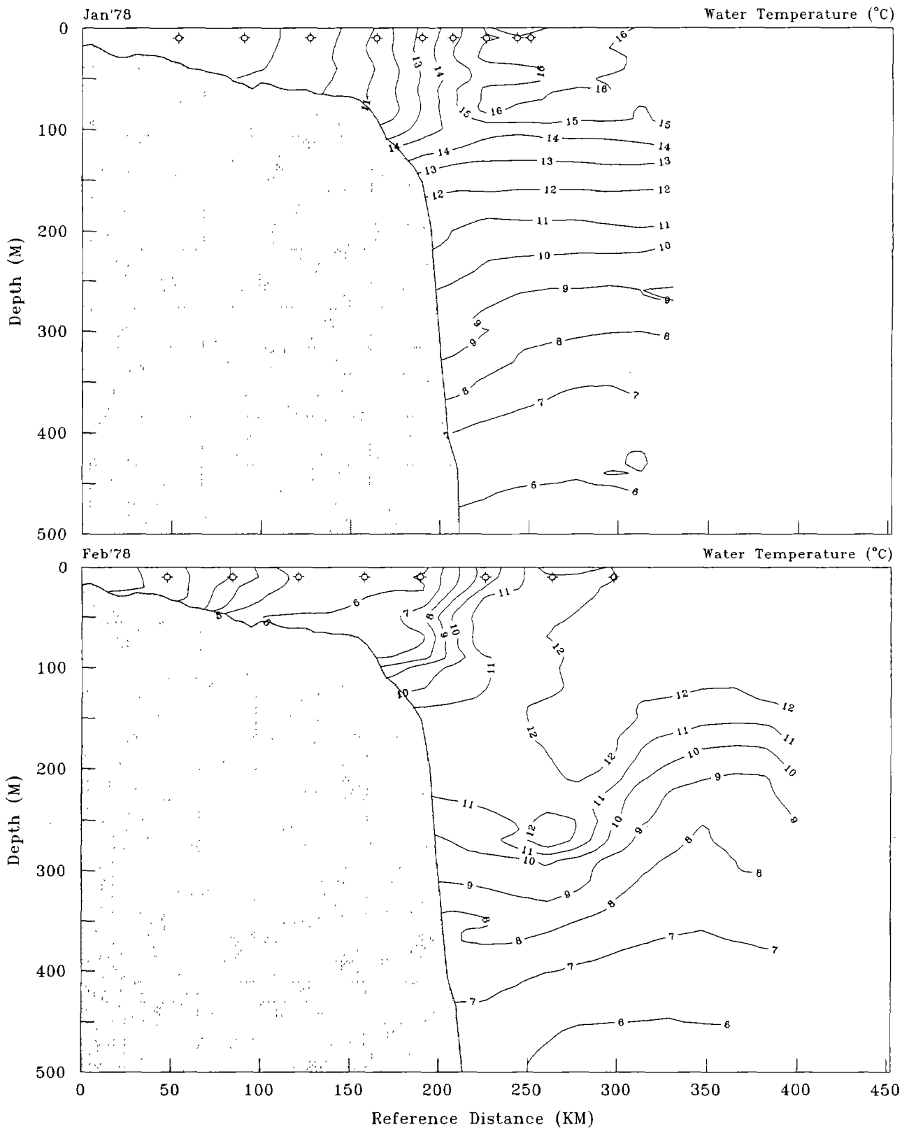
Figure 2. Water-column thermal structure (degrees Celsius) and CPR station locations at the 10-m depth (♠) along the Middle Atlantic Bight transect during January and February 1978.
