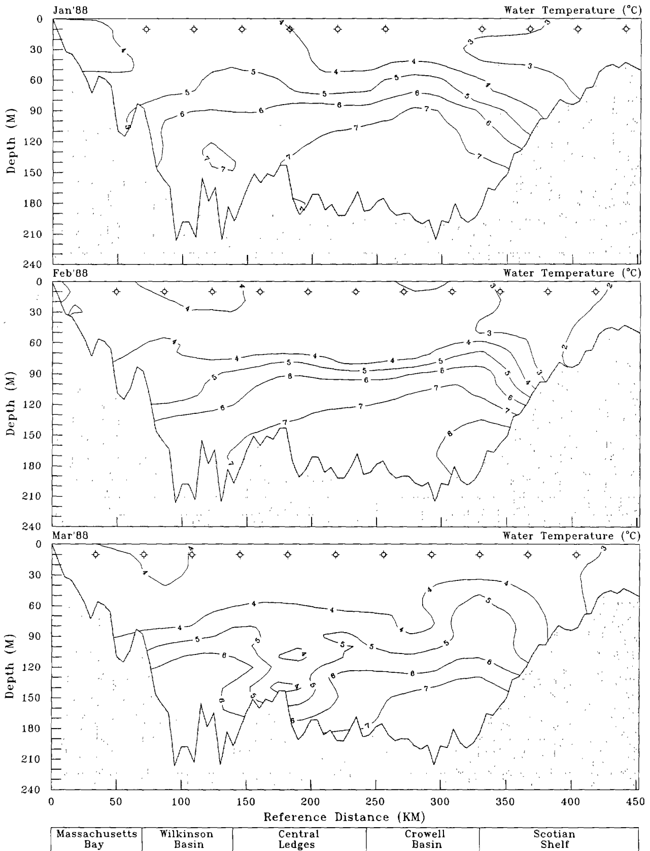
Figure 128. Water-column thermal structure (degrees Celsius) and CPR station locations at the 10-m depth (■) along the Gulf of Maine transect during January, February, and March 1988.
