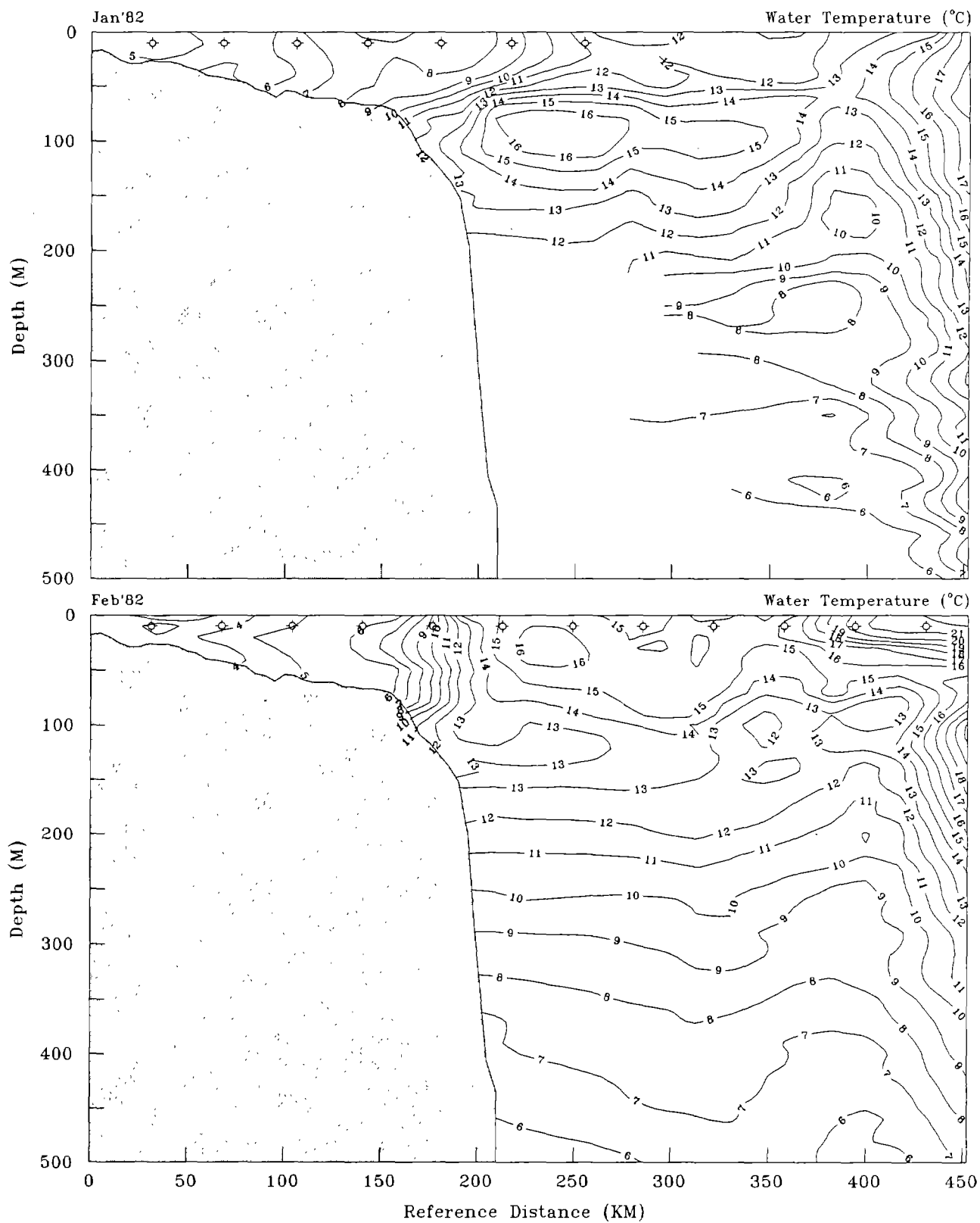
Figure 26. Water-column thermal structure (degrees Celsius) and CPR station locations at the 10-m depth ( \pi ) along the Middle Atlantic Bight transect during January and February 1982.
