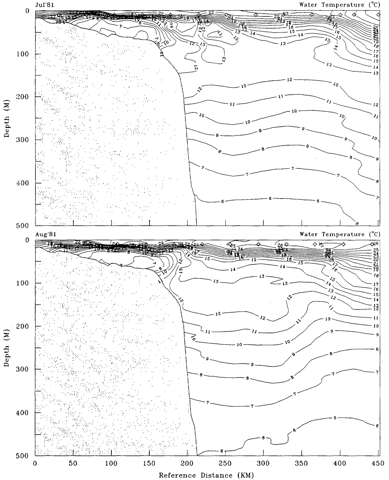
Figure 23. Water-column thermal structure (degrees Celsius) and CPR station locations at the 10-m depth ( \sigma ) along the Middle Atlantic Bight transect during July and August 1981.
