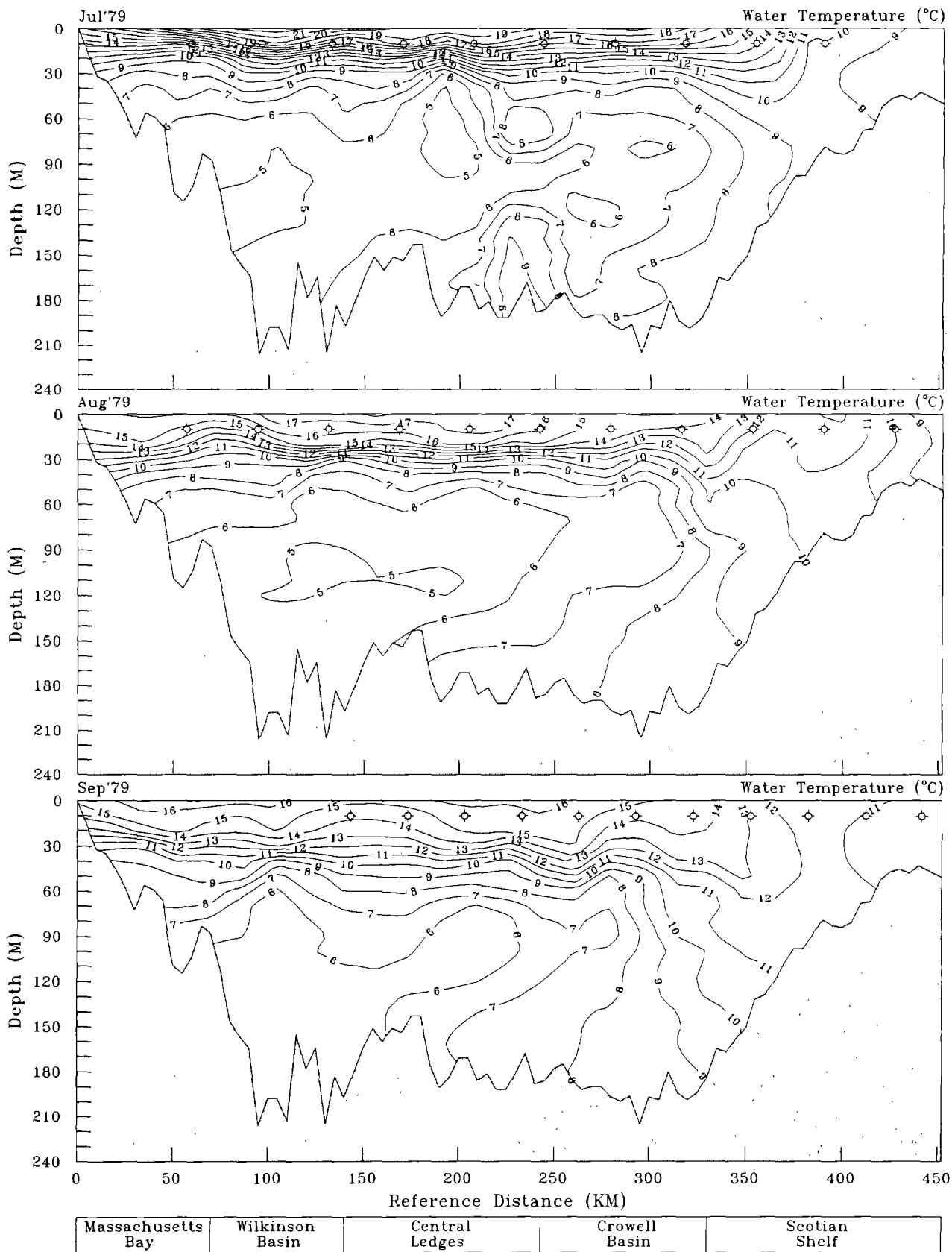
Figure 98. Water-column thermal structure (degrees Celsius) and CPR station locations at the 10-m depth (□) along the Gulf of Maine transect during July, August, and September 1979.
