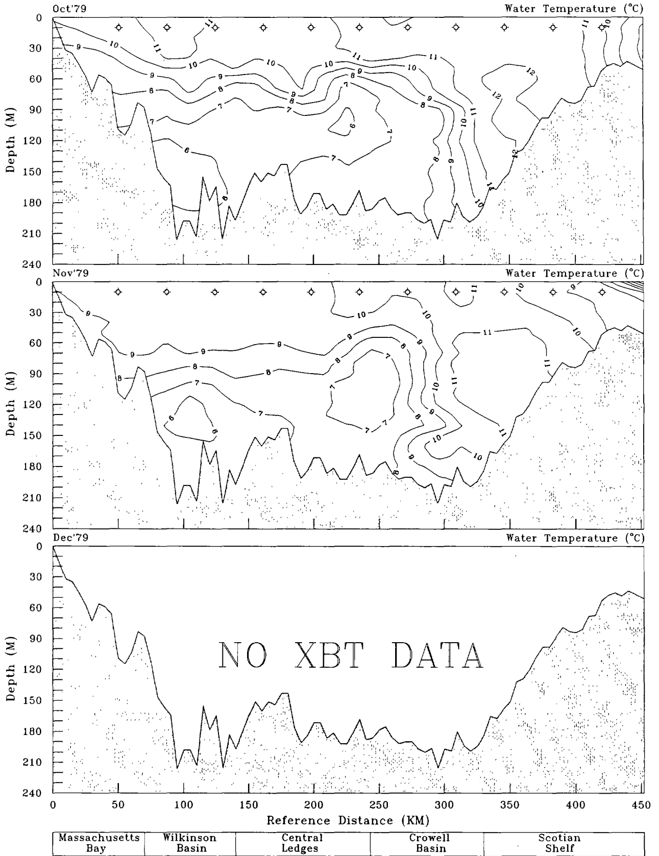
Figure 99. Water-column thermal structure (degrees Celsius) and CPR station locations at the 10-m depth (□) along the Gulf of Maine transect during October, November, and December 1979.
