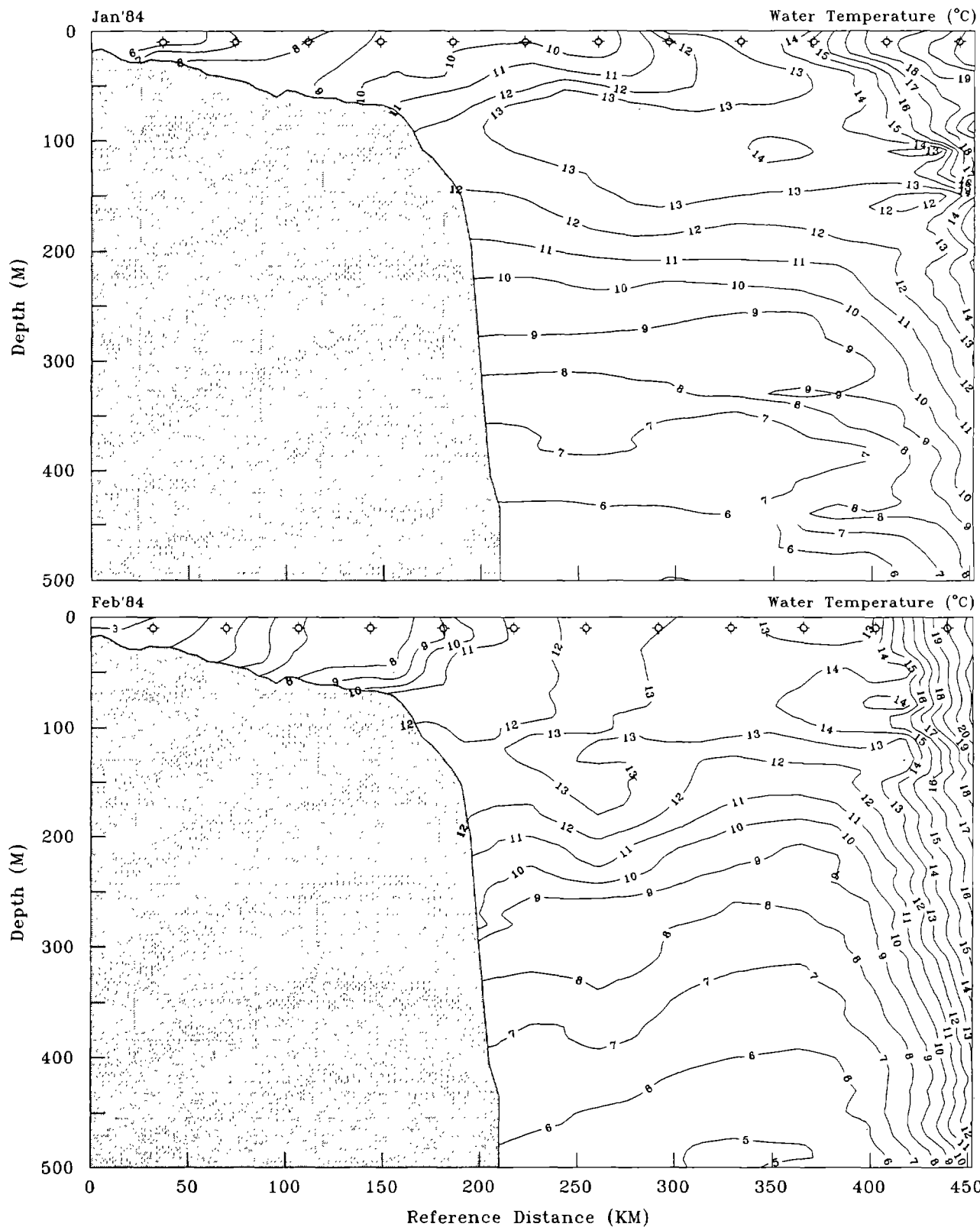
Figure 38. Water-column thermal structure (degrees Celsius) and CPR station locations at the 10-m depth ( \sigma ) along the Middle Atlantic Bight transect during January and February 1984.
