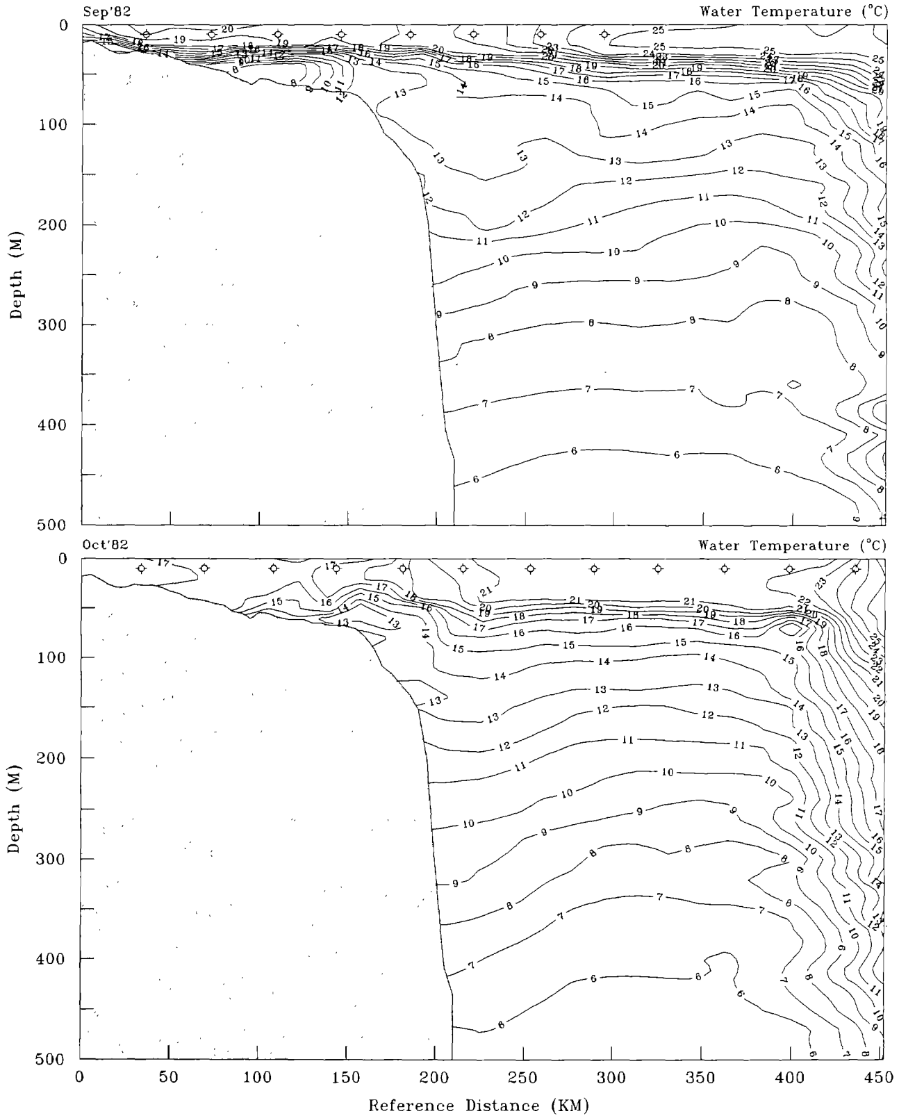
Figure 30. Water-column thermal structure (degrees Celsius) and CPR station locations at the 10-m depth ( \square ) along the Middle Atlantic Bight transect during September and October 1982.
