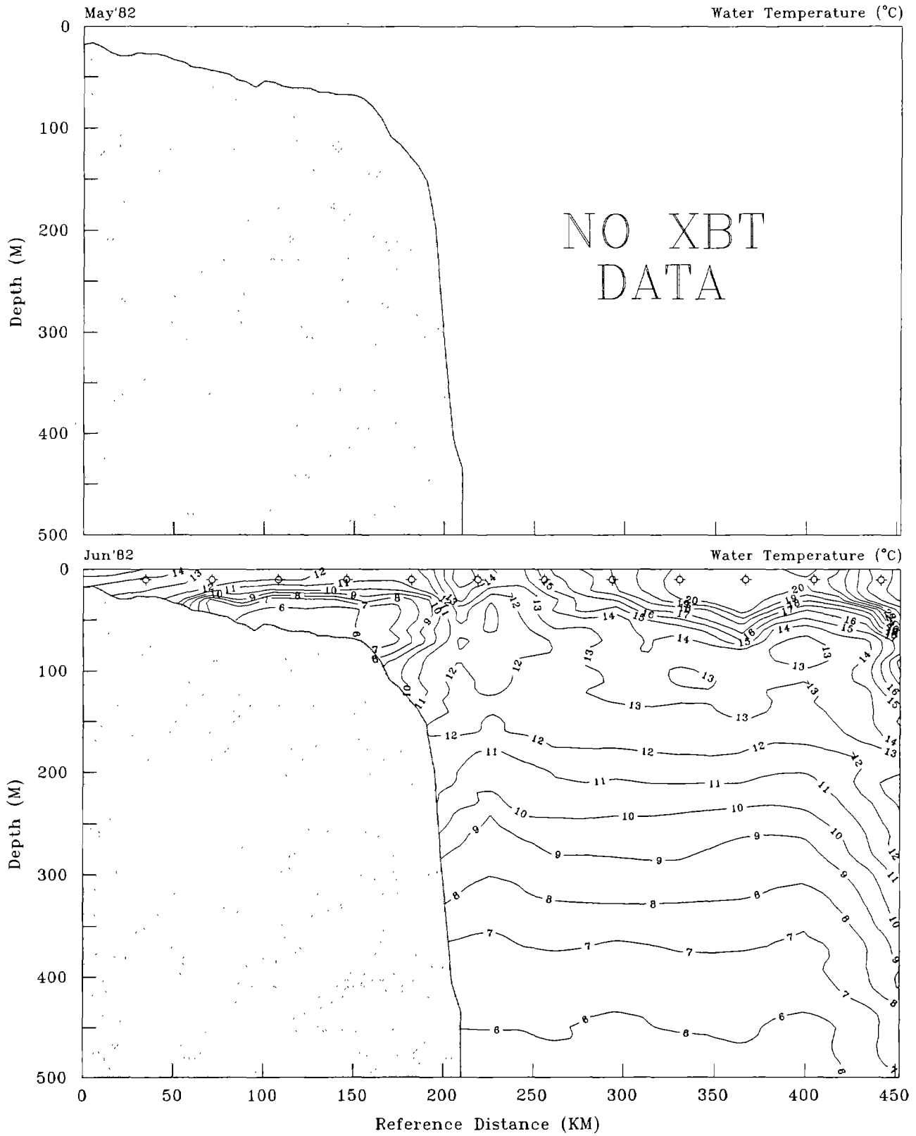
Figure 28. Water-column thermal structure (degrees Celsius) and CPR station locations at the 10-m depth ( \sigma ) along the Middle Atlantic Bight transect during May and June 1982.
