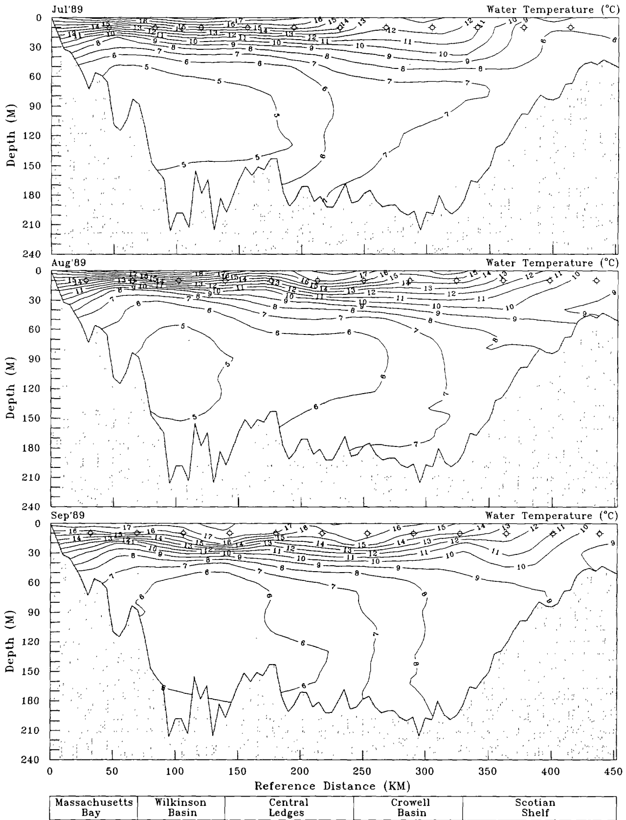
Figure 134. Water-column thermal structure (degrees Celsius) and CPR station locations at the 10-m depth (□) along the Gulf of Maine transect during July, August, and September 1989.
