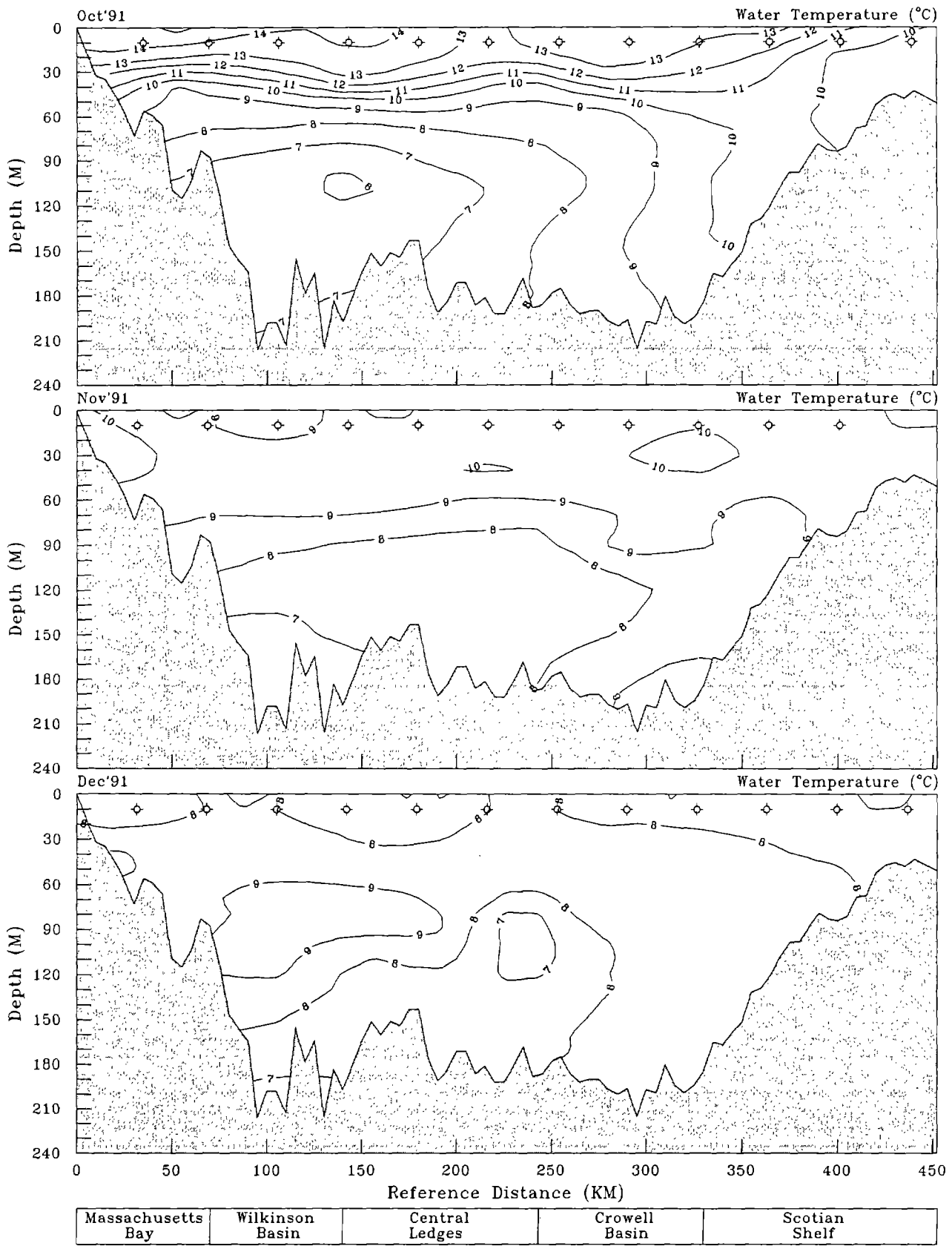
Figure 143. Water-column thermal structure (degrees Celsius) and CPR station locations at the 10-m depth (⊕) along the Gulf of Maine transect during October, November, and December 1991.
