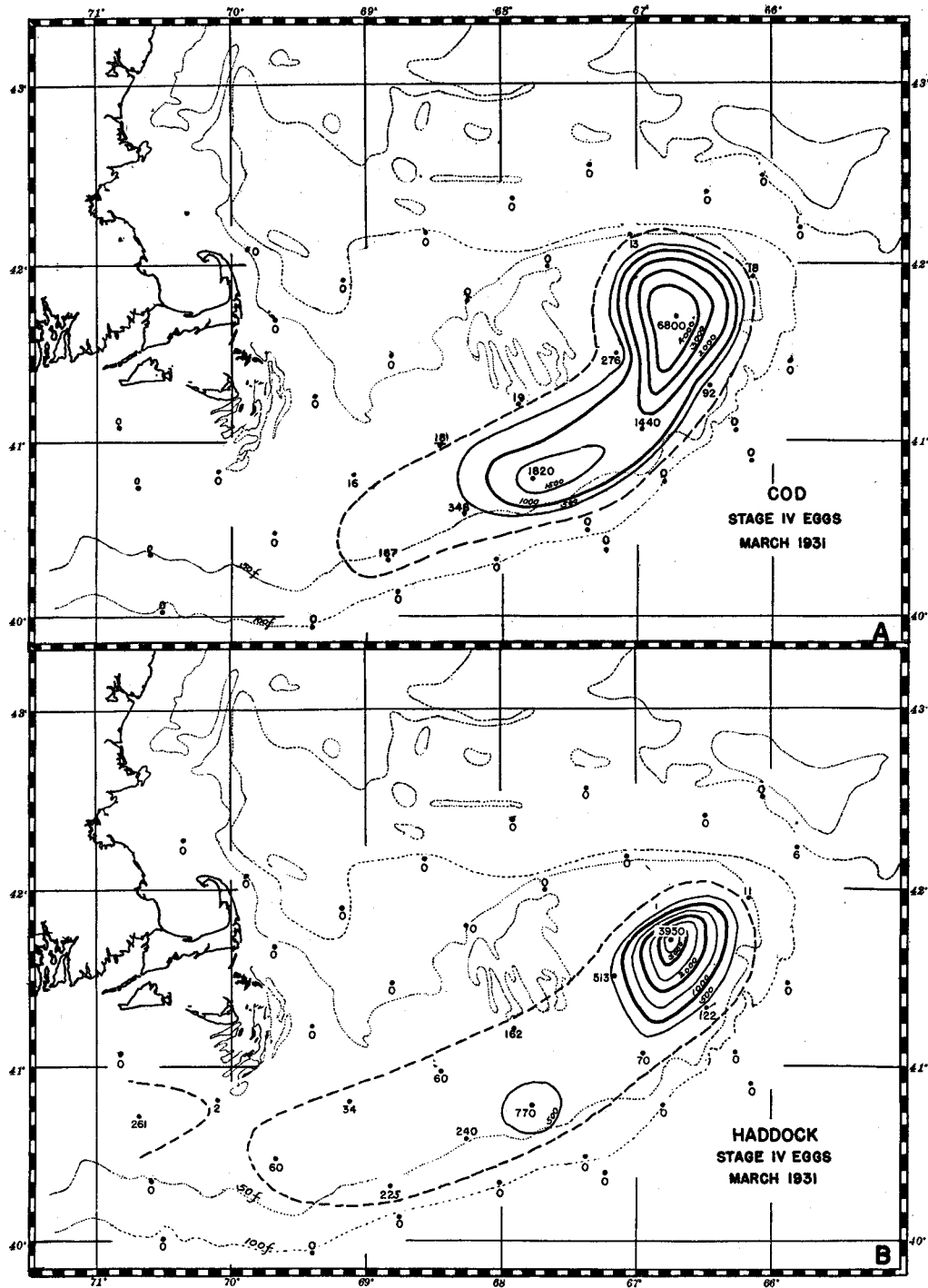
FIGURE 3.—Isometric chart showing the distribution of (A) stage IV cod eggs, and (B) stage IV haddock eggs, in March 1931. The numbers are population indices (p. 61).
