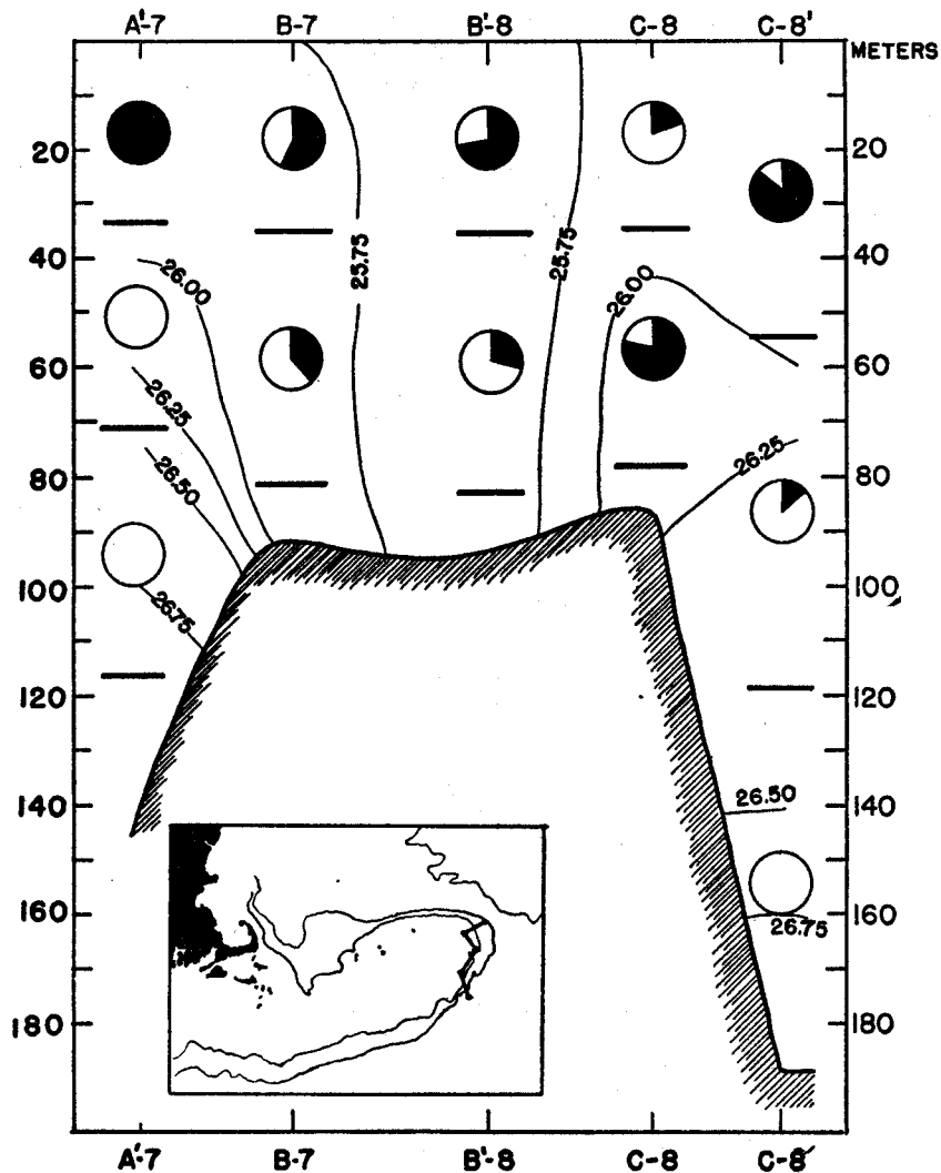
FIGURE 32.—Relation between the vertical distribution of cod-haddock eggs and the isopycnics on stations along the eastern edge of Georges Bank in April 1932. The solid line in the inset gives the location of the stations; Figure 9 gives an explanation of the symbols.
