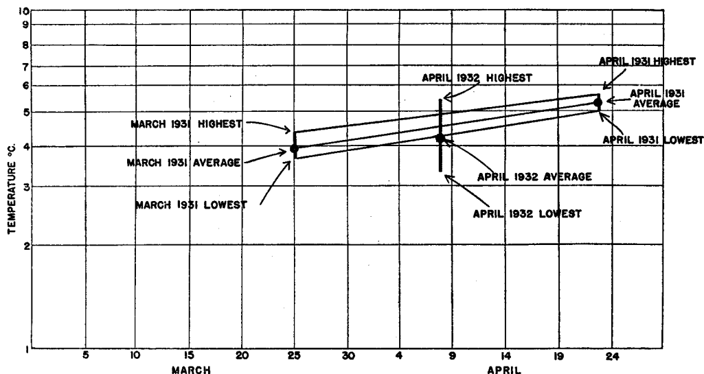
FIGURE 30.—Comparison of the temperature ranges in the eastern part of the bank from March to April 1931, with those for April 1932.
