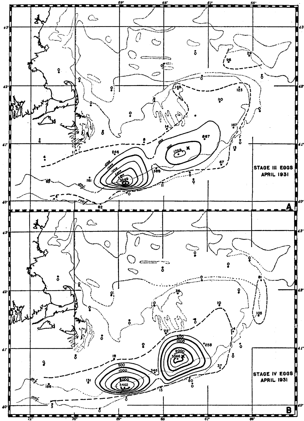
FIGURE 14.—Distribution of stage III (A) and IV (B) eggs, April 1931. The cross indicates the location of the reference point in the B concentration zone (p. 26).
