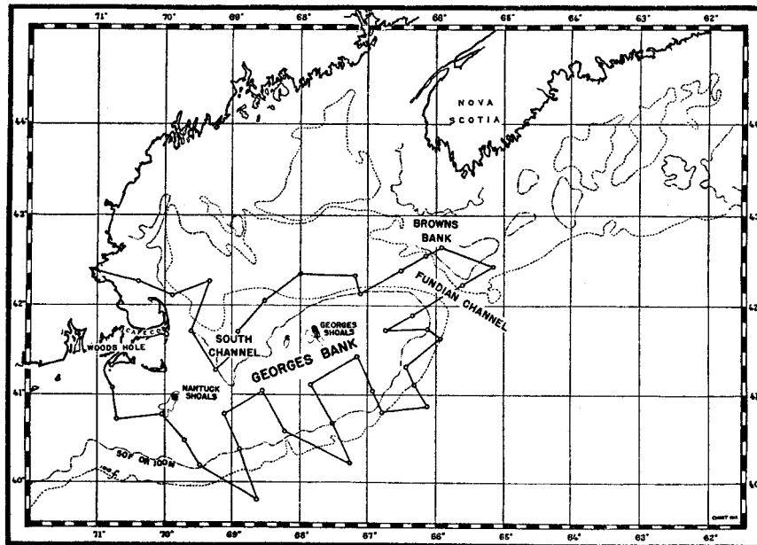
FIGURE 44.—Course followed by the Albatross II on the April 1932 cruise.
