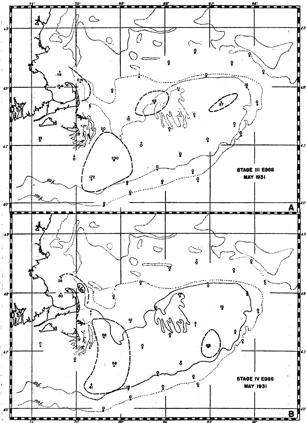
FIGURE 22.—Distribution of stage III (A) and IV (B) eggs in May 1931.
