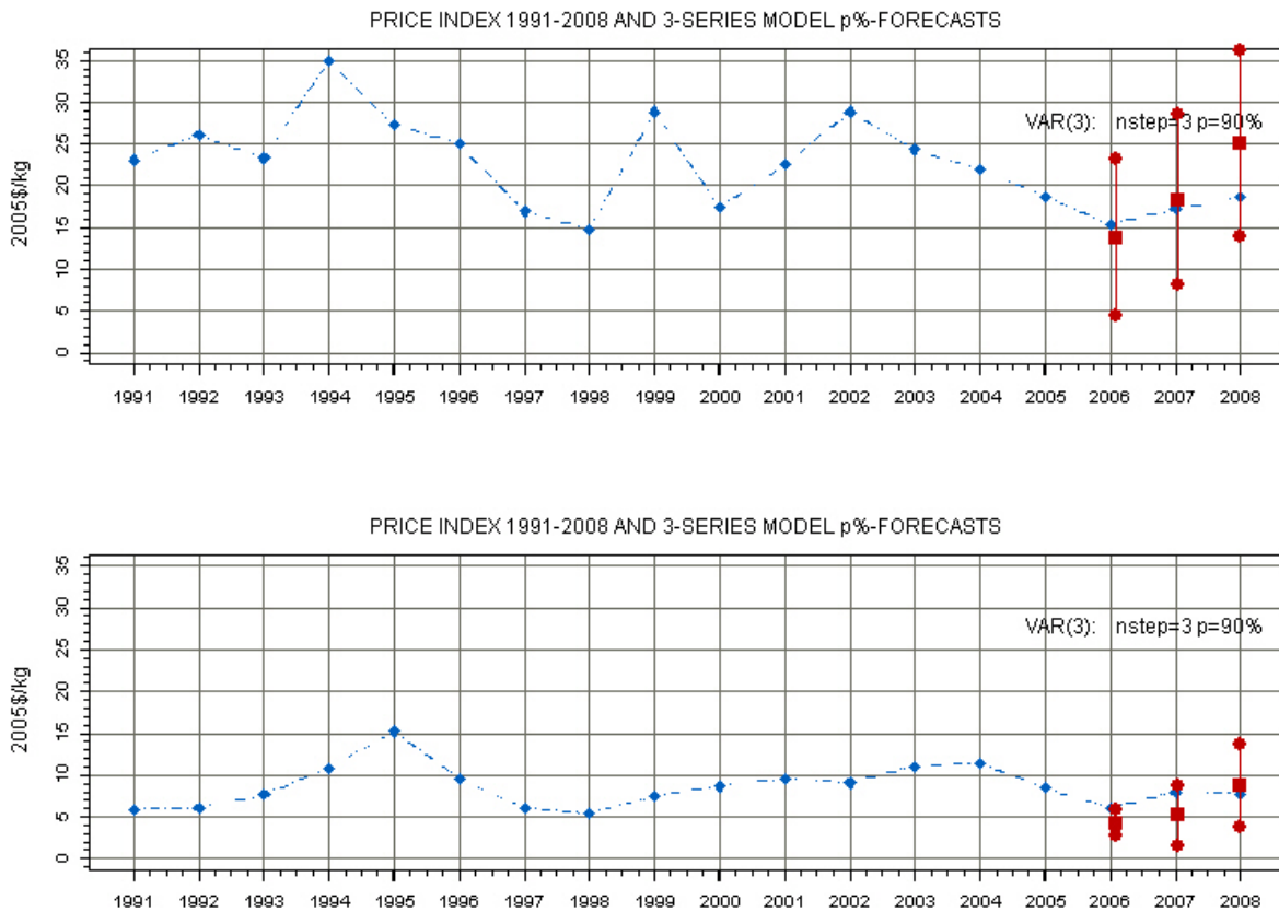
Fig. 1b: Red king crab VAR(3) model and data 1991-2008 with three price series based on COAR wholesale values for gold king crab (upper plot), COAR wholesale values for snow crab (lower plot), and TPIS king crab imports (not shown). The regression runs through 2005 with 90% 3-step forecasts for 2006-2008. The expected values of each forecast are represented by squares in the forecast intervals for each year. All values are in 2005 dollars per kilogram.
