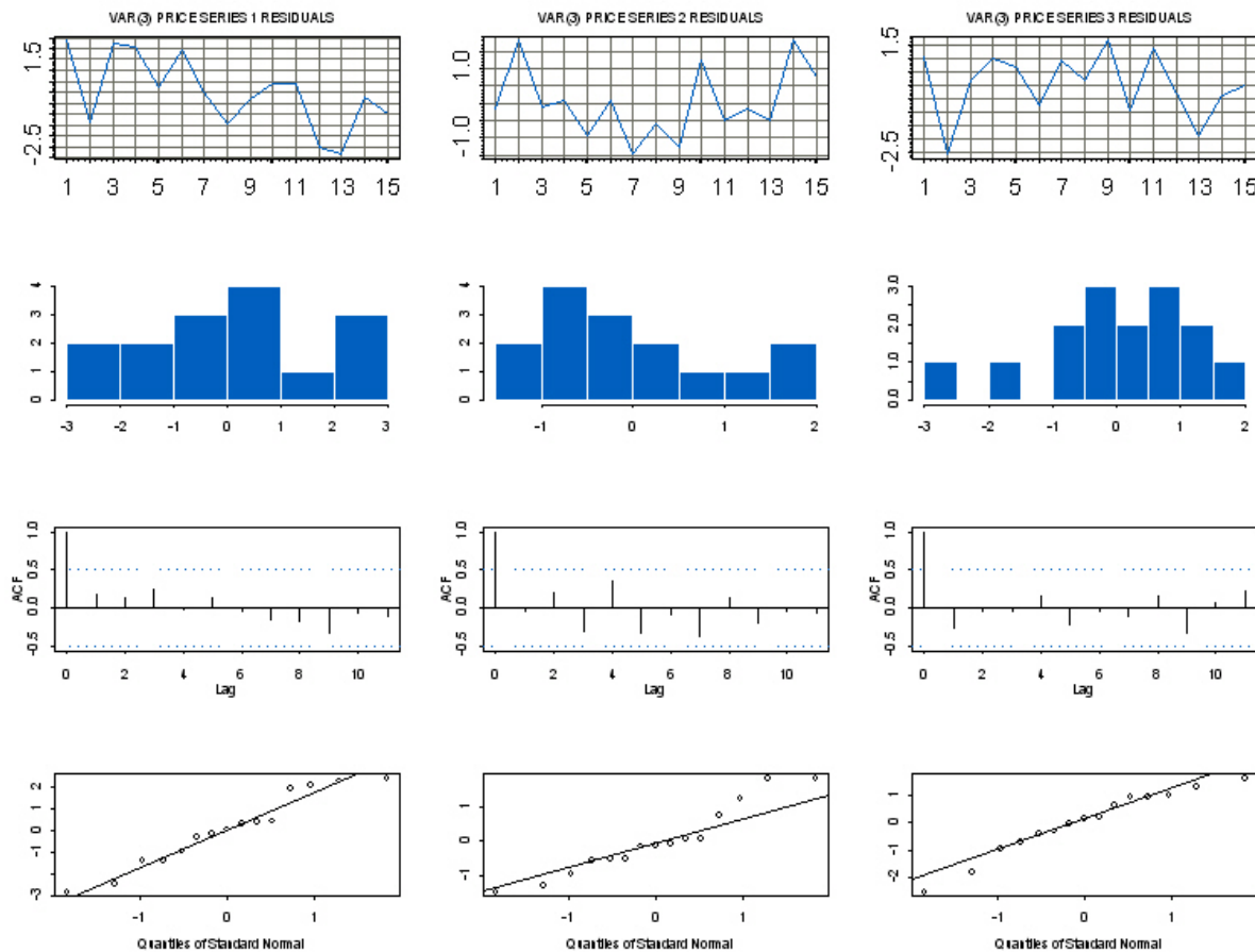
Fig. 5c: Snow crab VAR(3) model residual time series (upper row plots), residual histograms (upper-middle row plots), autocorrelation functions (lower-middle row plots), and normal quantile-quantile plots (lower row plots) for three price series based on COAR wholesale values for king crab (series 1, left-column plots), COAR wholesale values for snow crab (series 2, middle-column plot), and TPIS king crab imports (series 3, right-column plots). The regression runs through 2008. All values are standardized.
