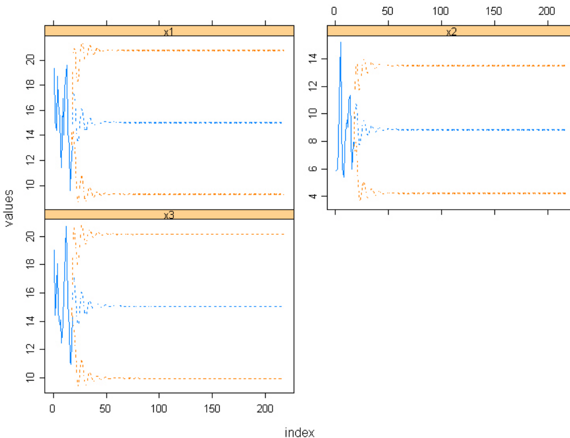
Fig. 3a: Gold king crab VAR(3) model and data 1991-2008 with three price series based on COAR wholesale values for gold king crab (x1, upper-left plot), COAR wholesale values for snow crab (x2, upper-right plot), and TPIS king crab imports (x3, lower-left plot). The regression runs through 2008 with 200-step 90%-forecasts for 2009-2208. All values are in 2005 dollars per kilogram.
