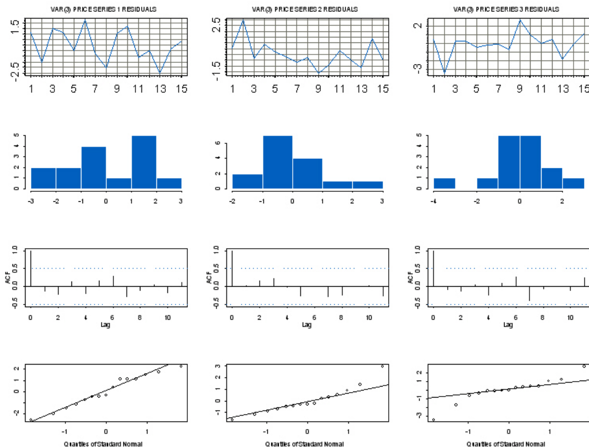
Fig. 5a: Gold king crab VAR(3) model residual time series (upper row plots), residual histograms (upper-middle row plots), autocorrelation functions (lower-middle row plots), and normal quantile-quantile plots (lower row plots) for three price series based on COAR wholesale values for gold king crab (series 1, left-column plots), COAR wholesale values for snow crab (series 2, middle-column plot), and TPIS king crab imports (series 3, right-column plots). The regression runs through 2008. All values are standardized.
