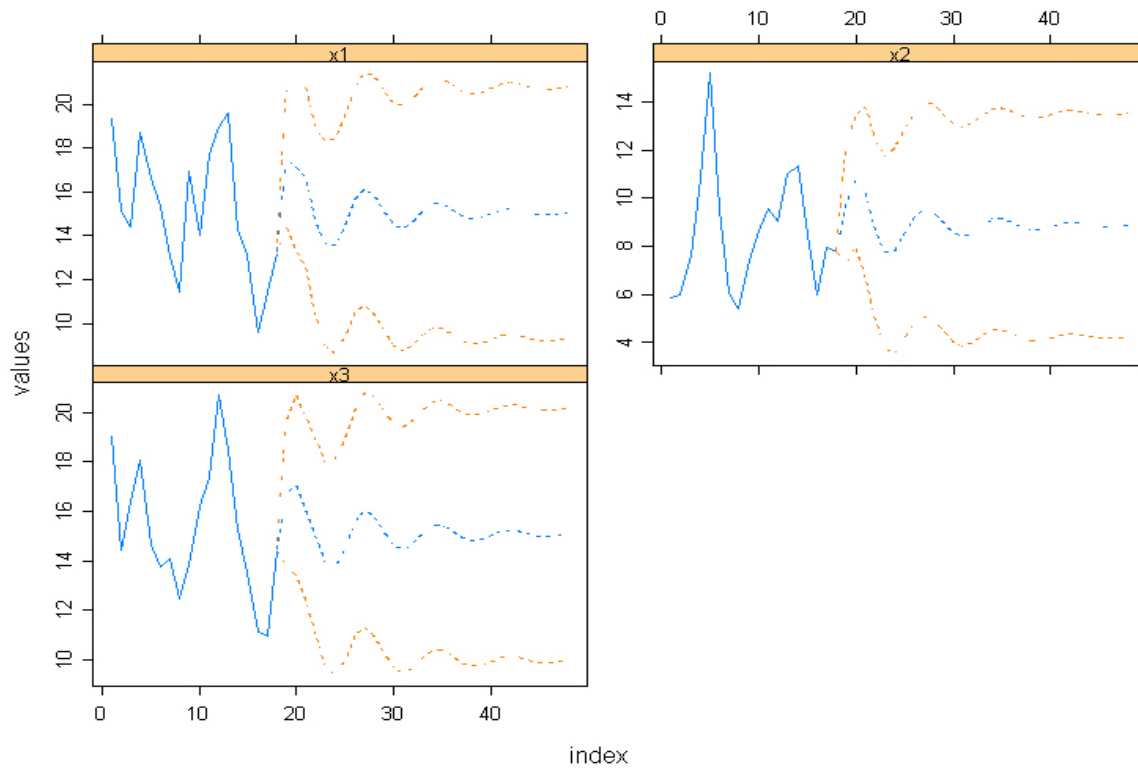
Fig. 2a: Gold king crab VAR(3) model and data 1991-2008 with three price series based on COAR wholesale values for gold king crab (x1, upper-left plot), COAR wholesale values for snow crab (x2, upper-right plot), and TPIS king crab imports (x3, lower-left plot). The regression runs through 2008 with 30-step 90%-forecasts for 2009-2038. All values are in real 2005 dollars per kilogram.
