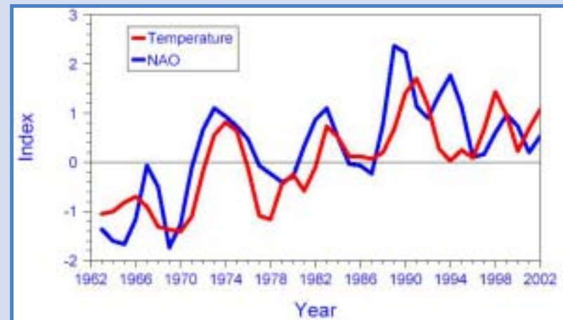
Relationship between the North Atlantic Oscillation index and water temperature at Woods Hole (both series smoothed using a low pass filter)
